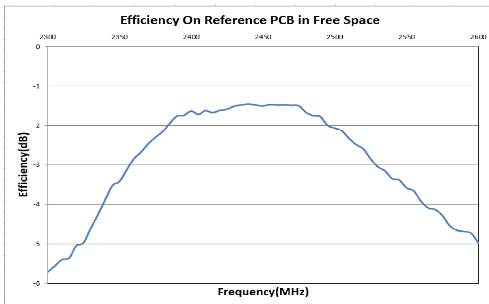
FIGURE 2.3 EFFICIENCY OF ANTENNA ON REFERENCE PCB AT REFERENCE LOCATION IN FREE SPACE
