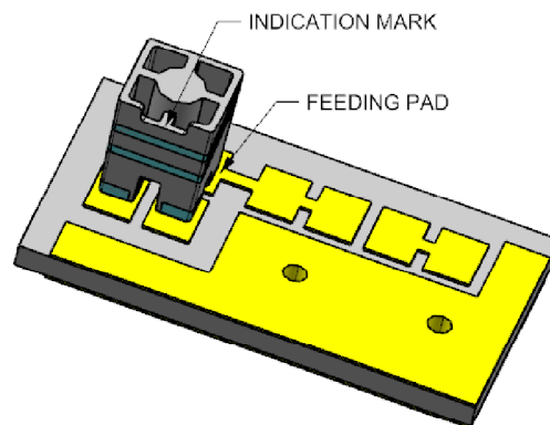
FIGURE 7.3 ANTENNA ASSEMBLY
