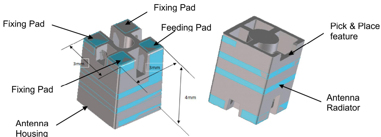
Figure 1: 2.4 GHz MID SMT Antenna
