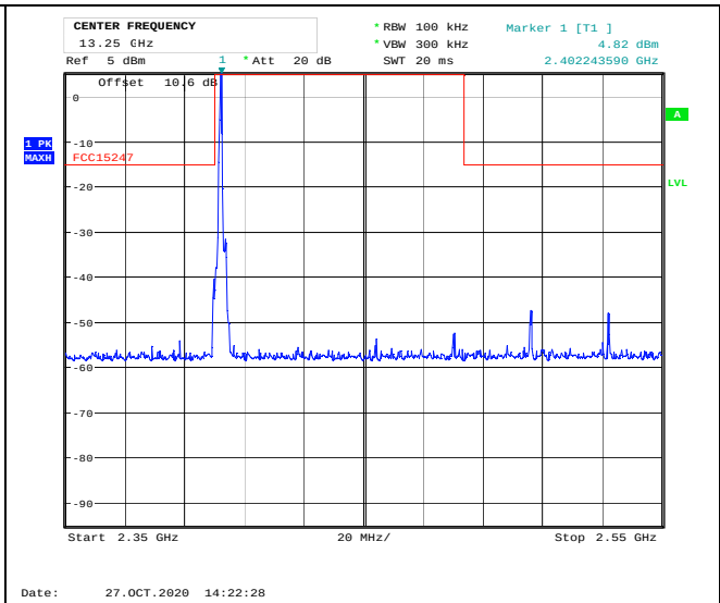
Conducted Emissions 2350-2550 MHz, 2402 MHz, GFSK
