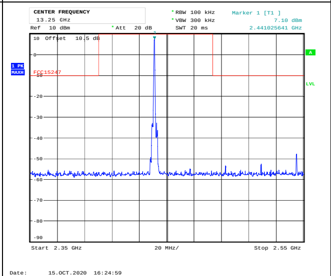
Conducted Emissions 2350-2550 MHz, 2441 MHz, GFSK
