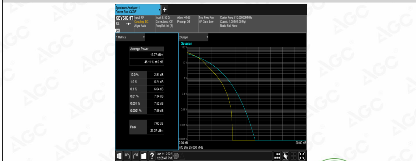
Band17-5MHz-16QAM-23790-25RB#0
