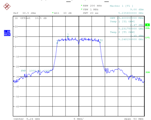
802.11a_5240MHz_Chain 1
