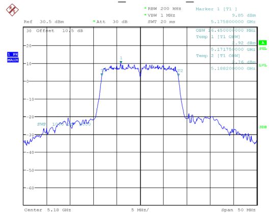
802.11a_5180MHz_Chain 1
