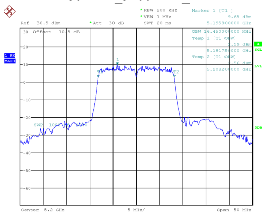
802.11a_5200MHz_Chain 1
