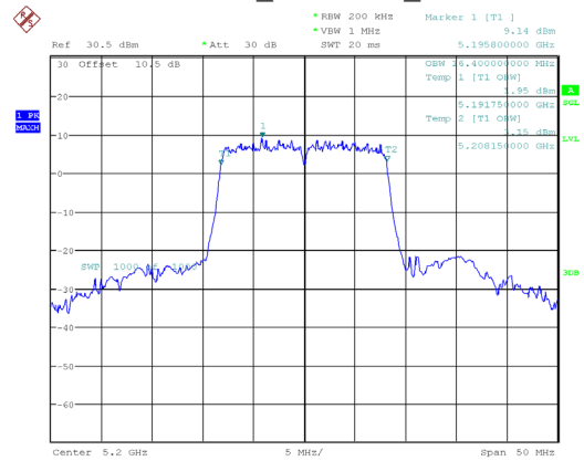
802.11a_5200MHz_Chain 0
