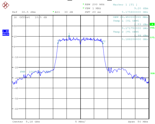
802.11a_5180MHz_Chain 0
