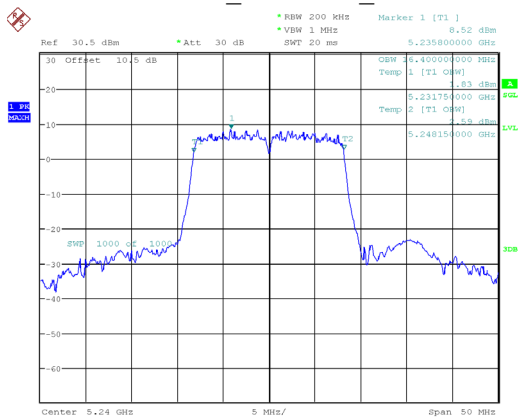
802.11a_5240MHz_Chain 0
