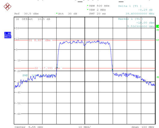
802.11ac40_5550MHz_Chain 0
