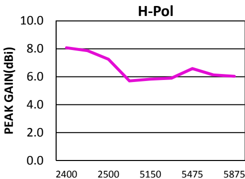
PEAK GAIN
