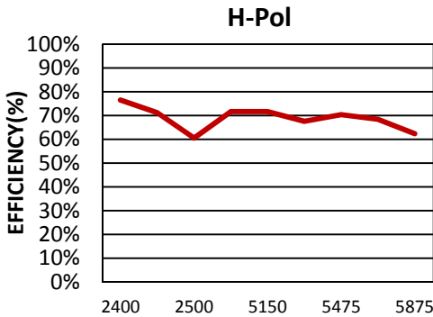
EFFICIENCY
