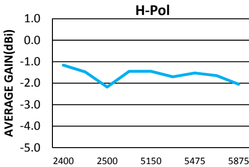
AVERAGE GAIN
