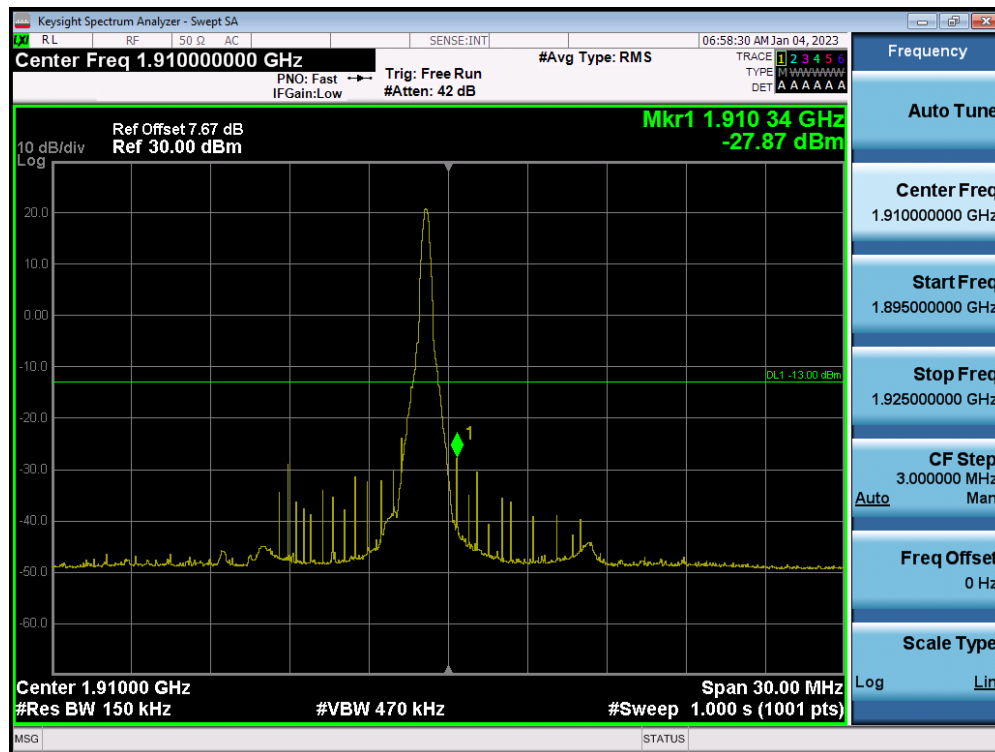
LTE Band 2 / 15MHz / 64QAM - RB Size/Offset (1/74)
