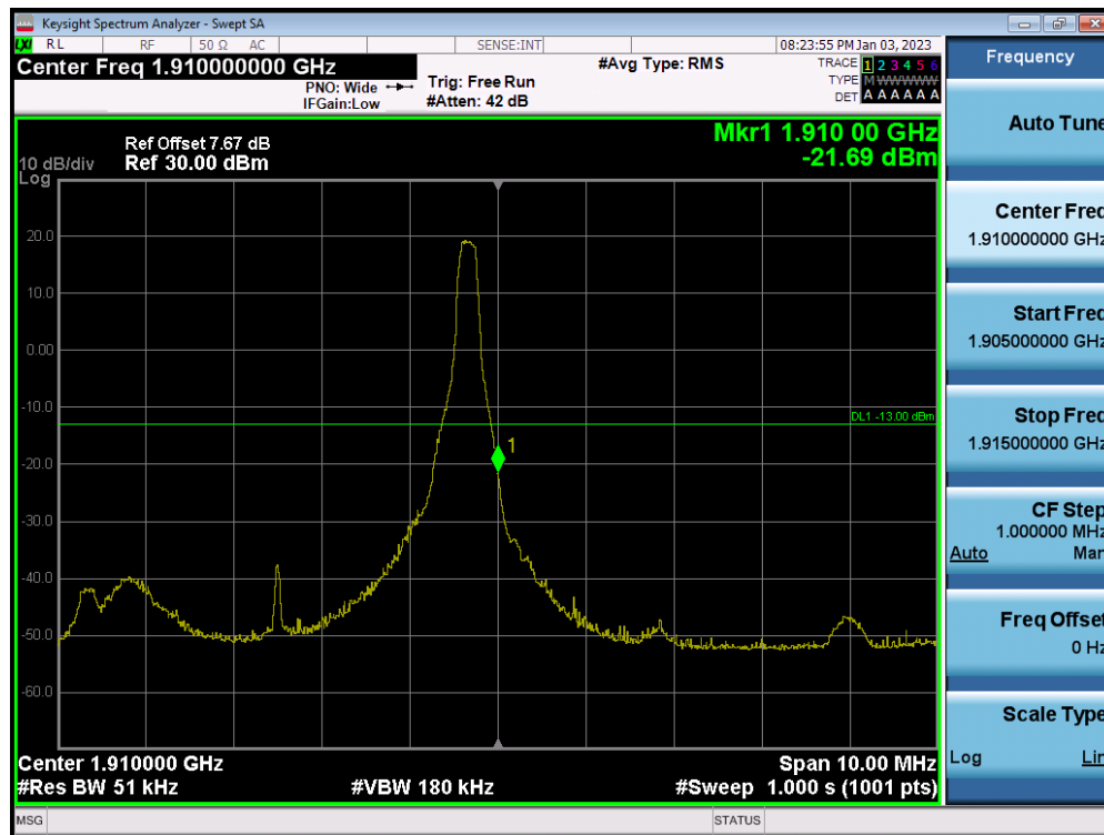
LTE Band 2 / 5MHz / QPSK - RB Size/Offset (1/24)
