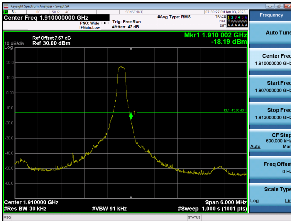
LTE Band 2 / 3MHz / QPSK - RB Size/Offset (1/14)
