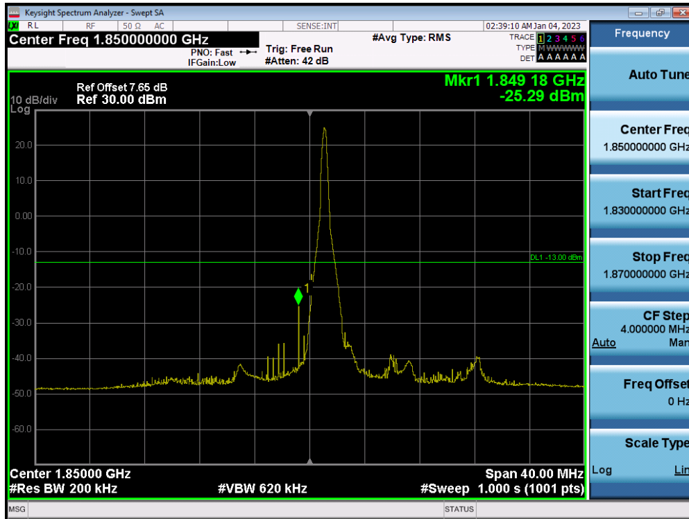
LTE Band 2 / 20MHz / 16QAM - RB Size/Offset (1/0)
