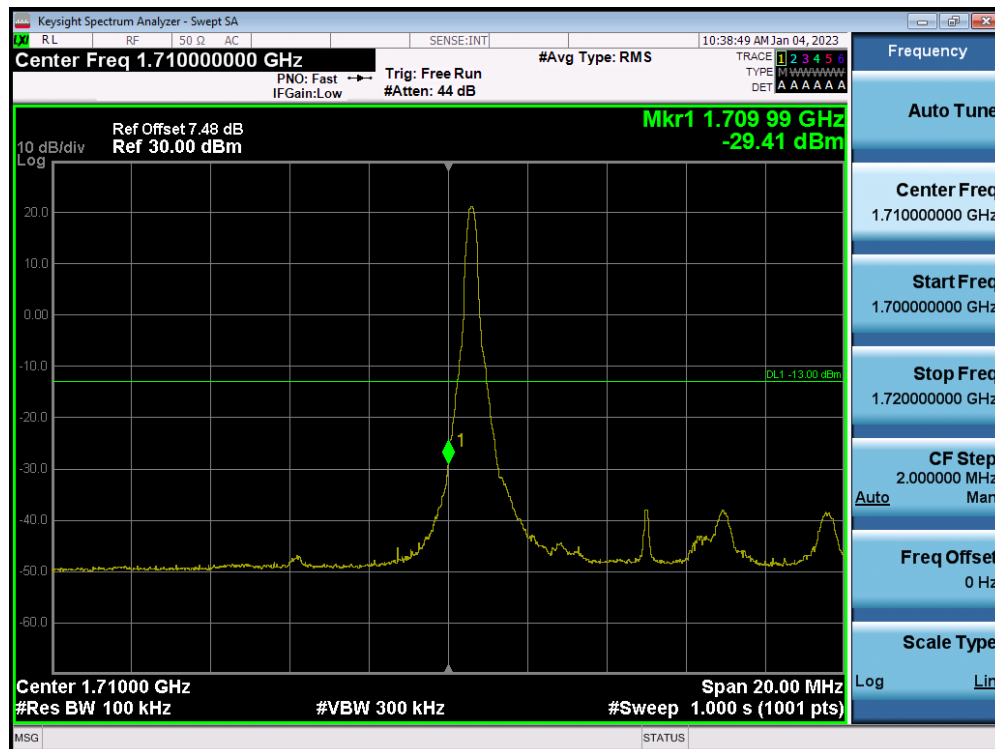
LTE Band 66(4) / 10MHz / QPSK - RB Size/Offset (1/0)
