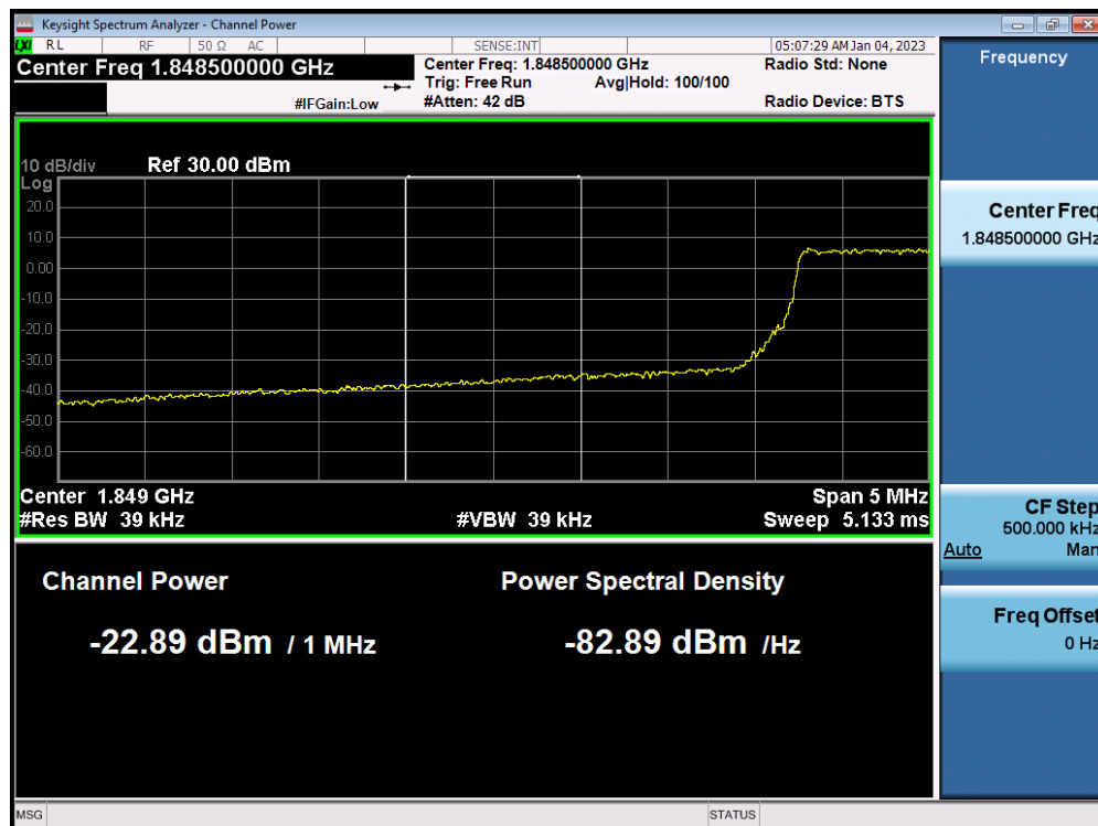
LTE Band 2 / 5MHz / 64QAM - RB Size/Offset (12/0)
