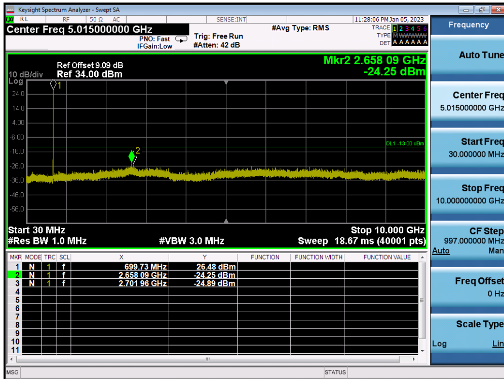
LTE Band 12 / 5MHz / 64QAM - RB Size/Offset (12/0) - Low Channel
