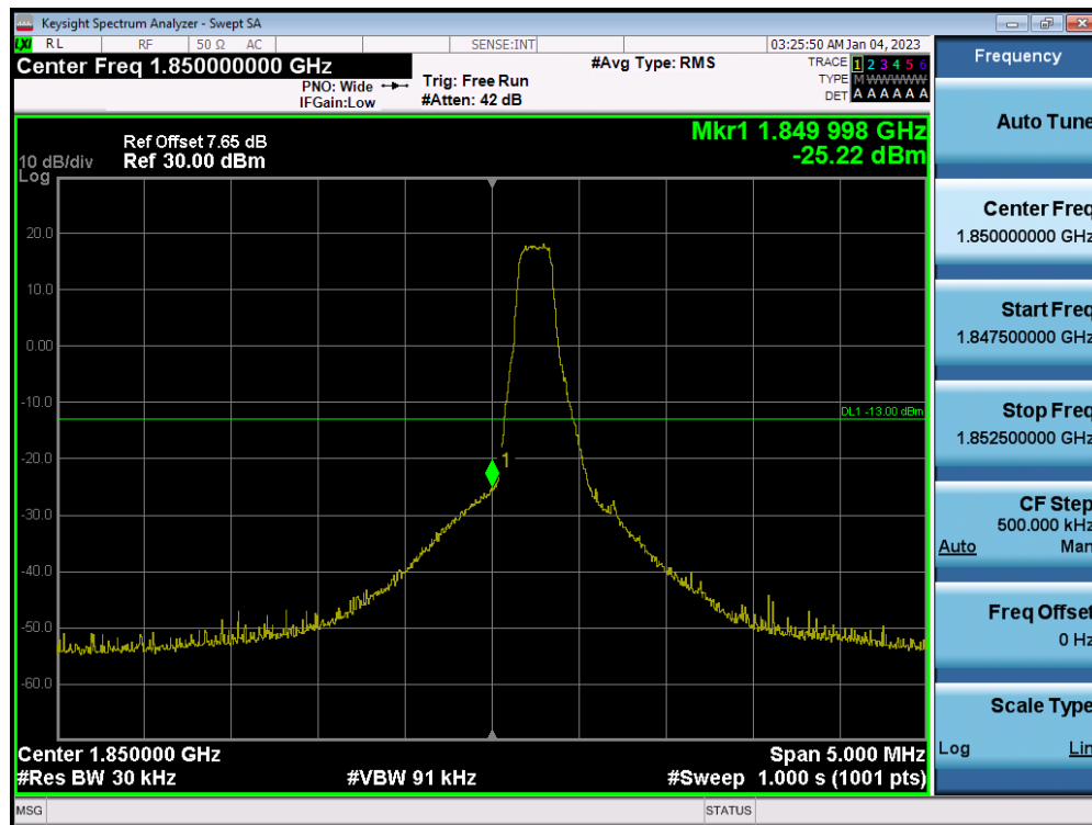
LTE Band 2 / 1.4MHz / 64QAM - RB Size/Offset (1/0)
