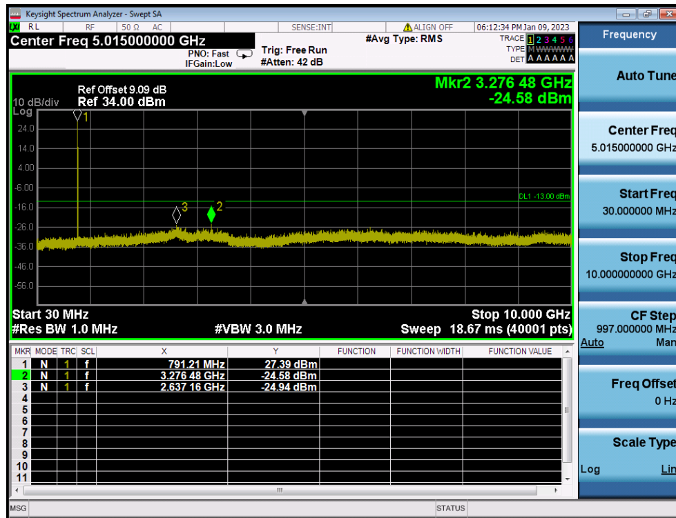
LTE Band 14 / 5MHz / 16QAM - RB Size/Offset (12/13) - Low Channel
