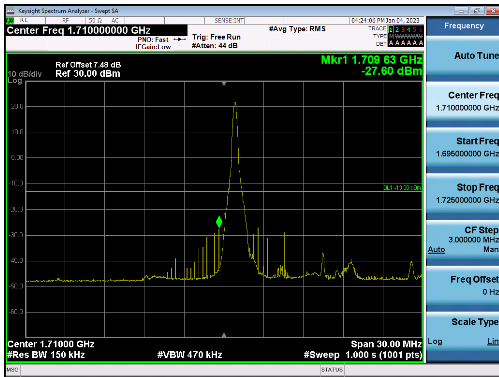
LTE Band 66(4) / 15MHz / 16QAM - RB Size/Offset (1/0)
