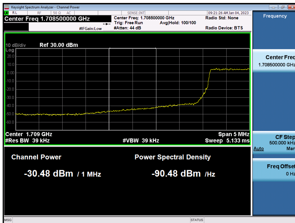
LTE Band 66(4) / 3MHz / QPSK - RB Size/Offset (15/0)
