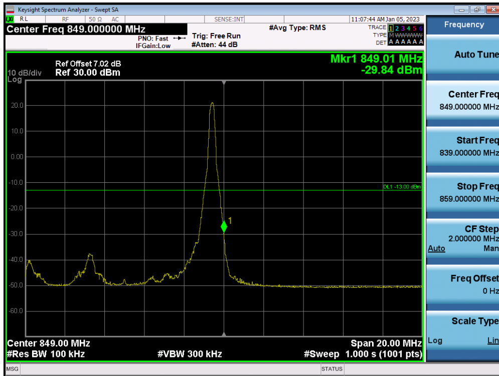
LTE Band 5 / 10MHz / QPSK - RB Size/Offset (1/49)
