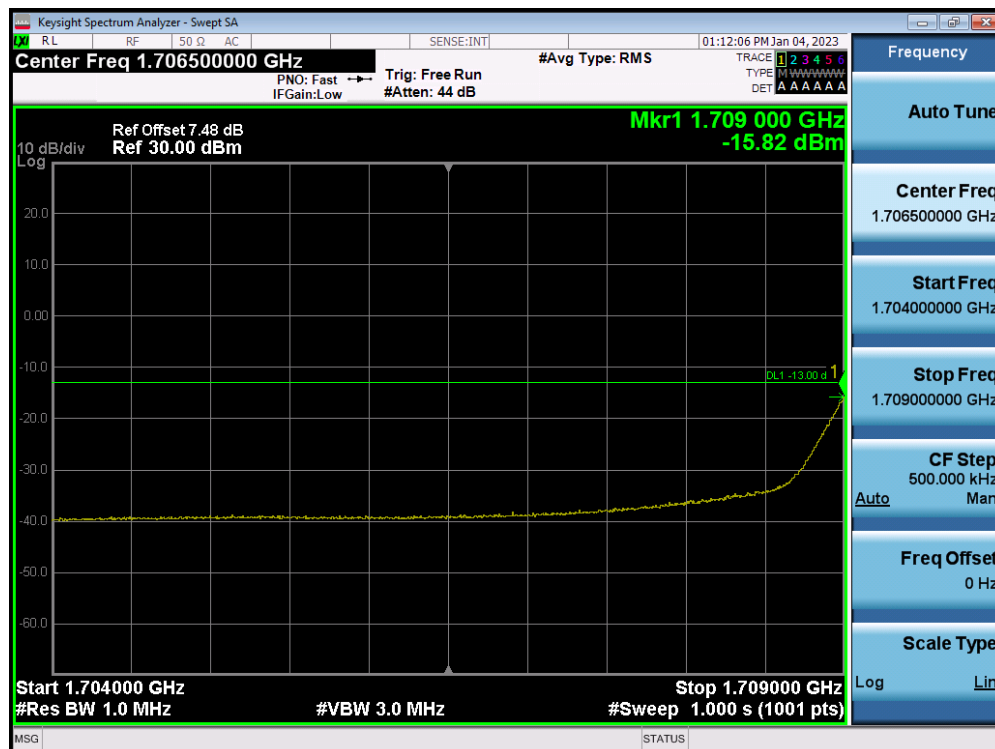
LTE Band 66(4) / 1.4MHz / 16QAM - RB Size/Offset (3/2)
