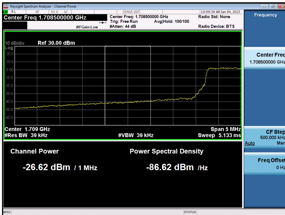
LTE Band 66(4) / 5MHz / QPSK - RB Size/Offset (25/0)
