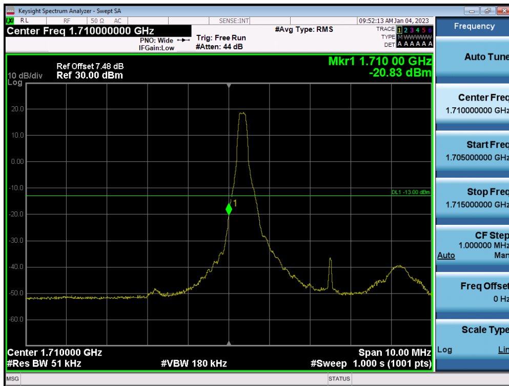
LTE Band 66(4) / 5MHz / QPSK - RB Size/Offset (1/0)
