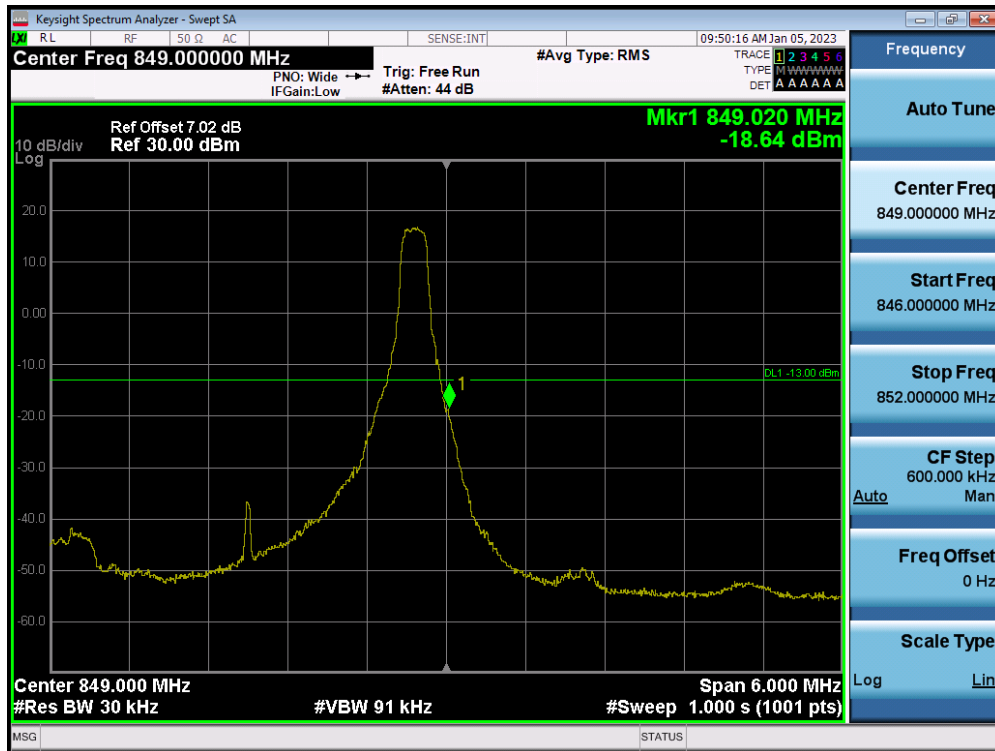
LTE Band 5 / 3MHz / QPSK - RB Size/Offset (1/14)
