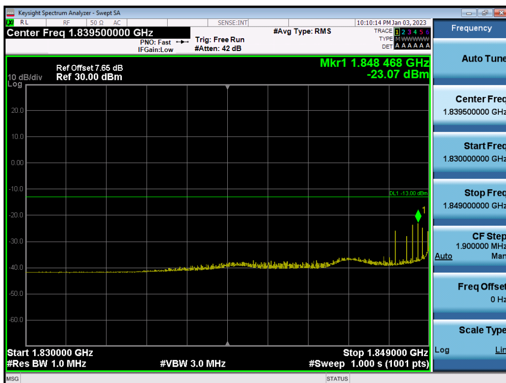
LTE Band 2 / 20MHz / QPSK - RB Size/Offset (1/0)
