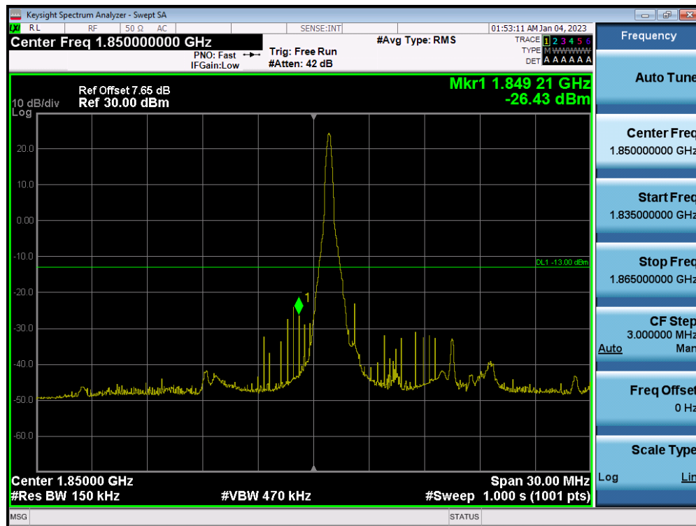
LTE Band 2 / 15MHz / 16QAM - RB Size/Offset (1/0)
