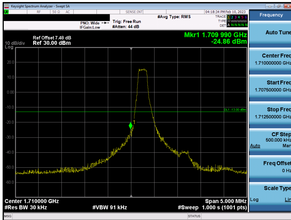
LTE Band 66(4) / 1.4MHz / 16QAM - RB Size/Offset (1/0)
