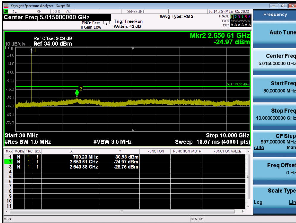
LTE Band 12 / 1.4MHz / 64QAM - RB Size/Offset (1/5) - Low Channel
