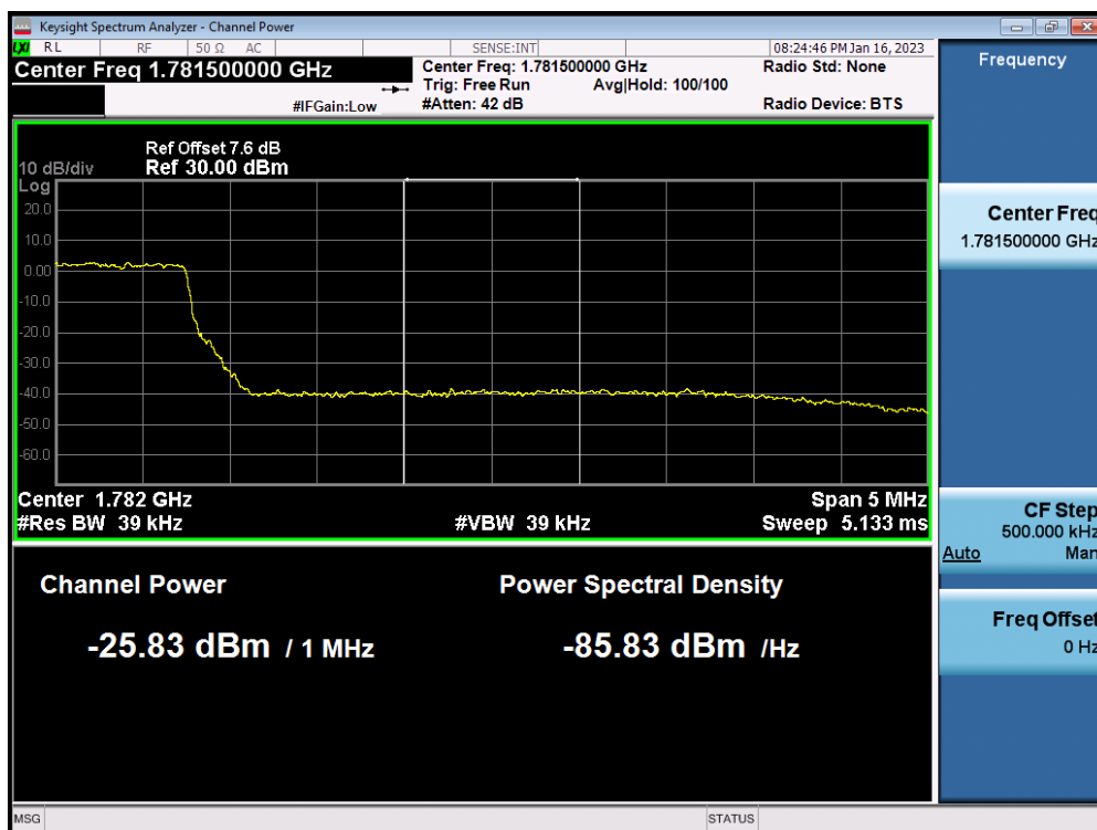
LTE Band 66(4) / 5MHz / 16QAM - RB Size/Offset (25/0)
