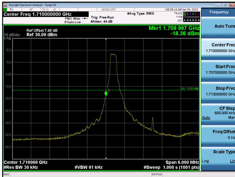
LTE Band 66(4) / 3MHz / QPSK - RB Size/Offset (1/0)
