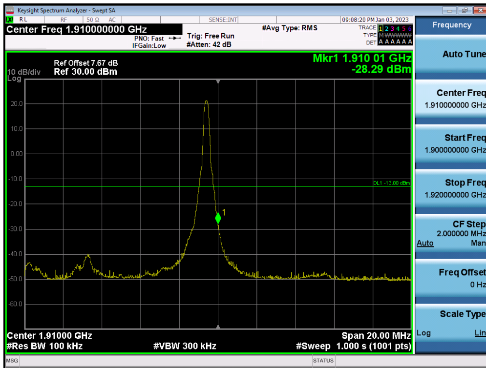
LTE Band 2 / 10MHz / QPSK - RB Size/Offset (1/49)
