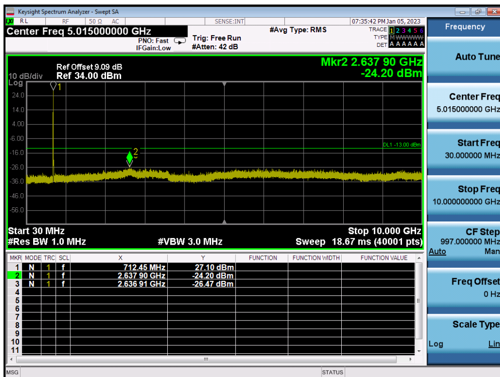
LTE Band 12 / 10MHz / QPSK - RB Size/Offset (25/12) - Mid Channel
