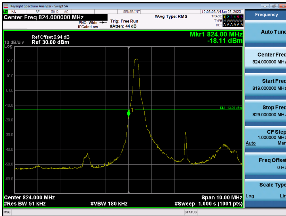
LTE Band 5 / 5MHz / QPSK - RB Size/Offset (1/0)
