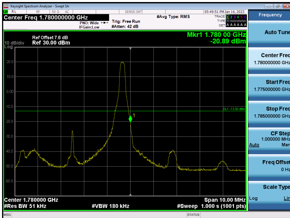
LTE Band 66(4) / 5MHz / QPSK - RB Size/Offset (1/24)
