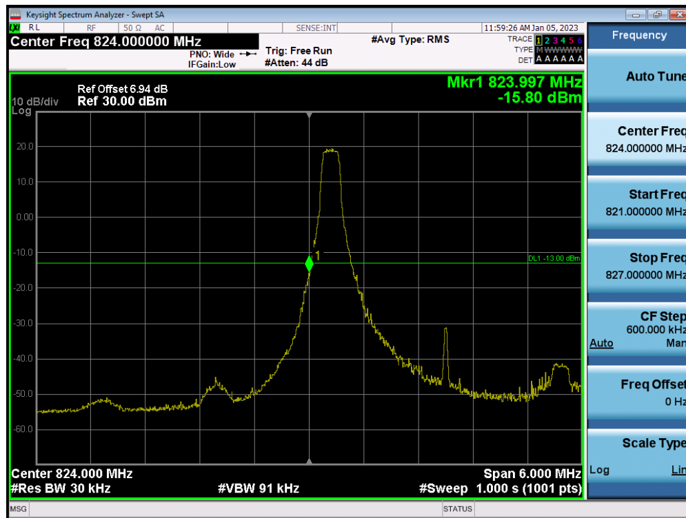
LTE Band 5 / 3MHz / 16QAM - RB Size/Offset (1/0)
