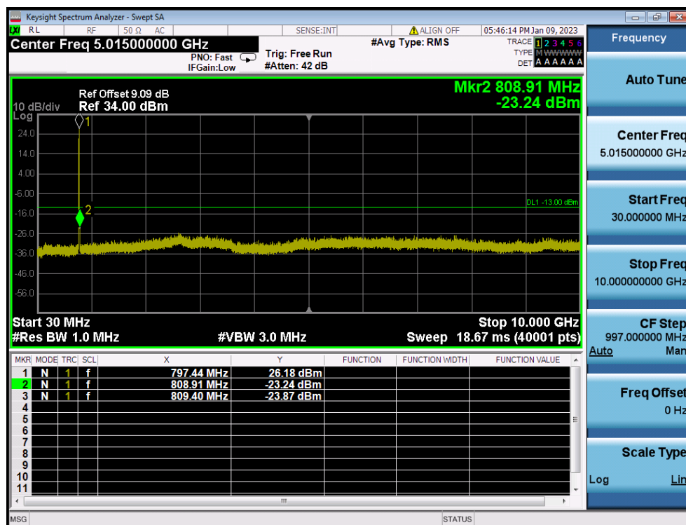
LTE Band 14 / 5MHz / QPSK - RB Size/Offset (25/0) - Mid Channel
