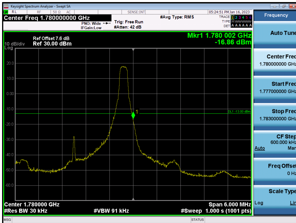
LTE Band 66(4) / 3MHz / QPSK - RB Size/Offset (1/14)
