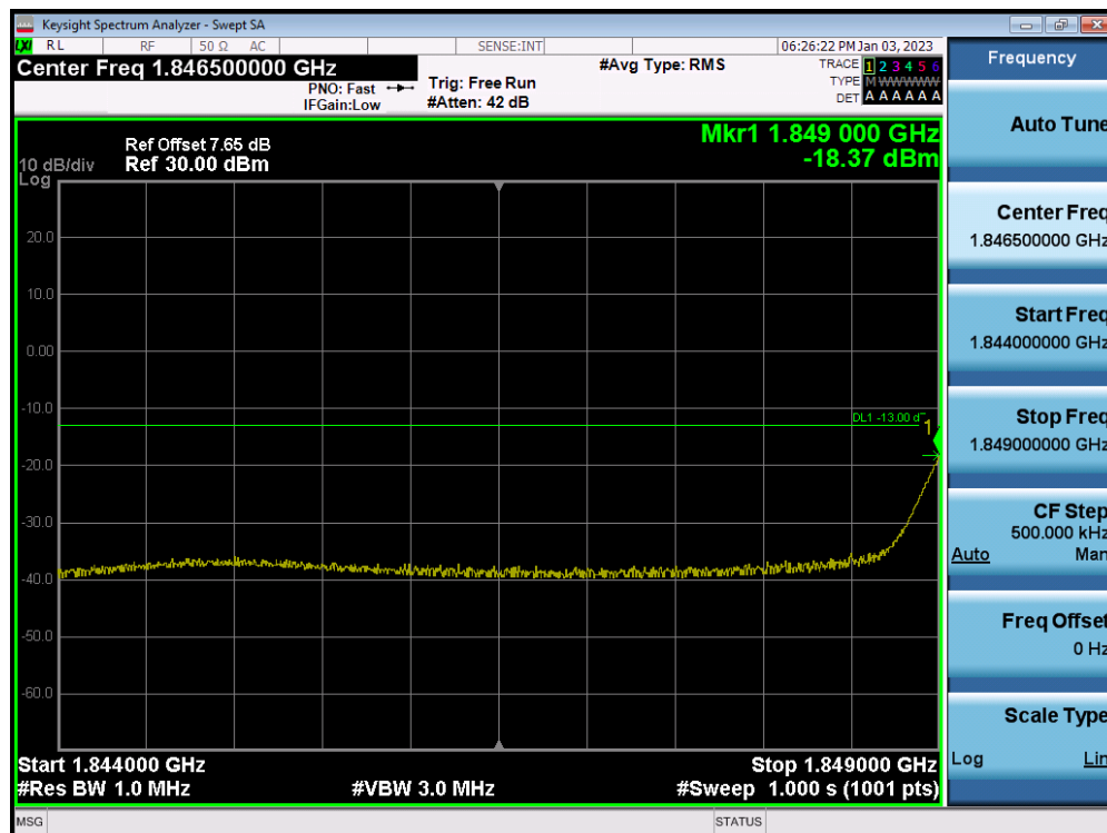
LTE Band 2 / 1.4MHz / QPSK - RB Size/Offset (1/2)
