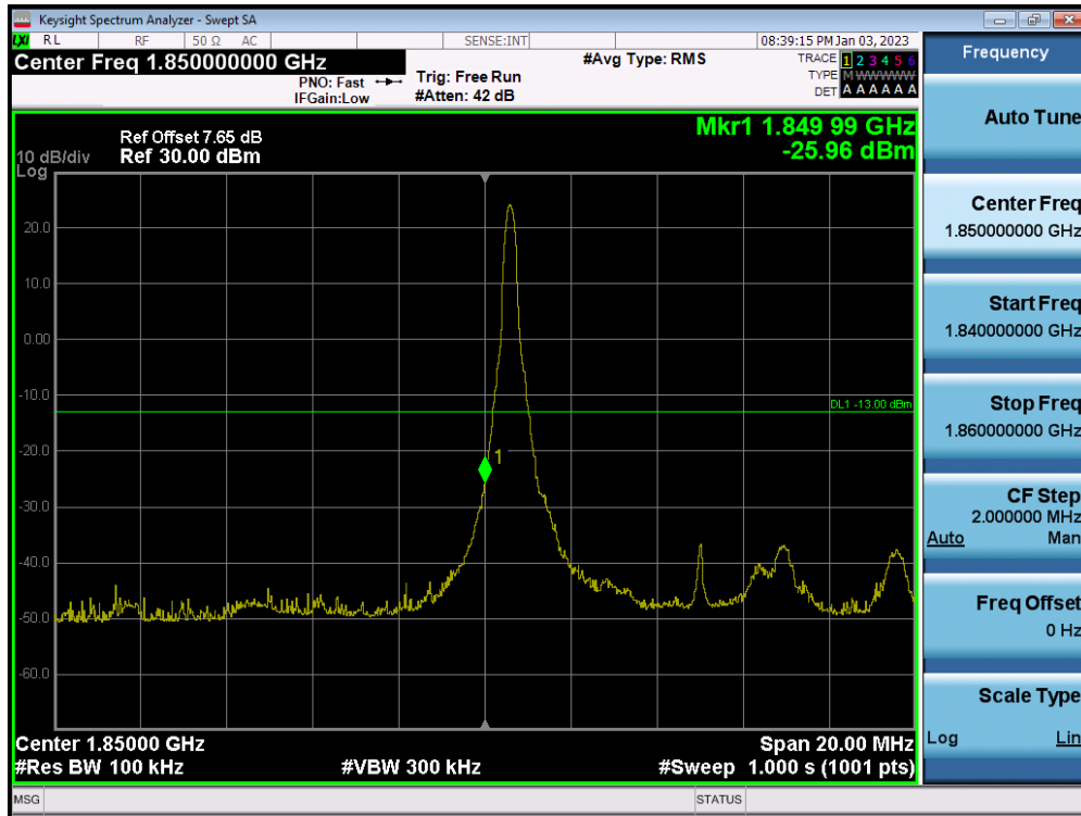
LTE Band 2 / 10MHz / QPSK - RB Size/Offset (1/0)
