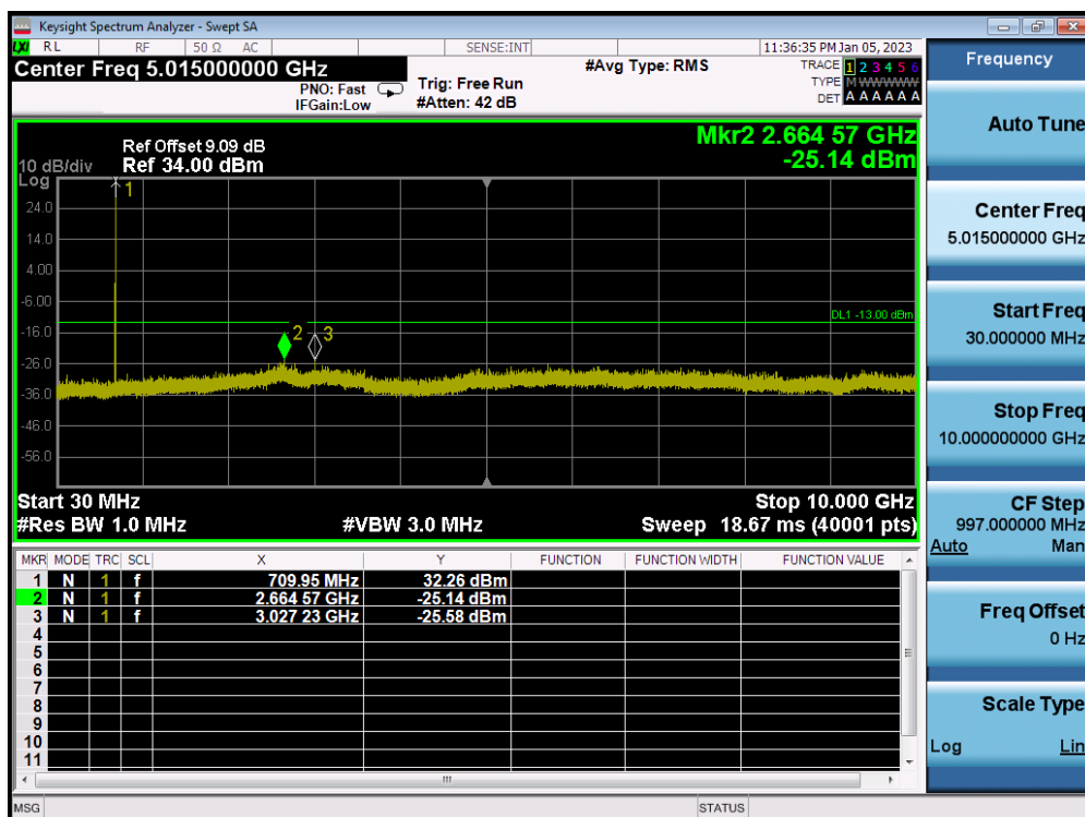
LTE Band 12 / 5MHz / 64QAM - RB Size/Offset (1/24) - Mid Channel
