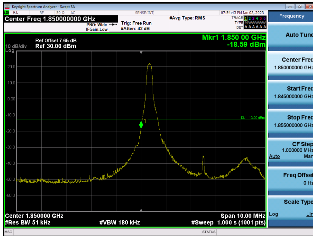
LTE Band 2 / 5MHz / QPSK - RB Size/Offset (1/0)
