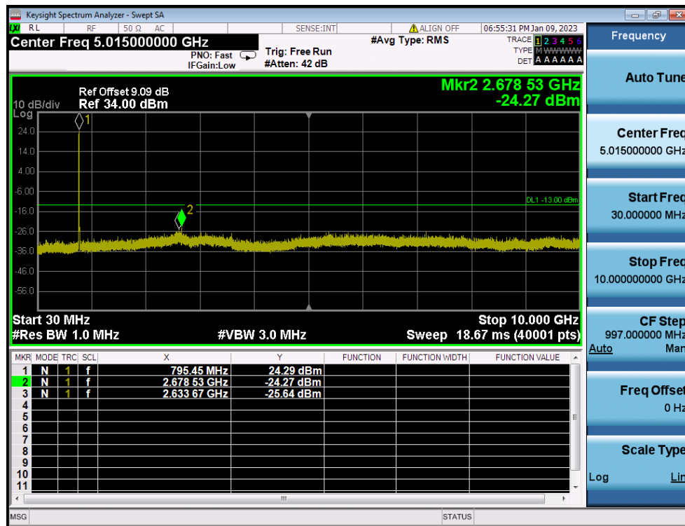
LTE Band 14 / 10MHz / 64QAM - RB Size/Offset (25/25) - Low Channel
