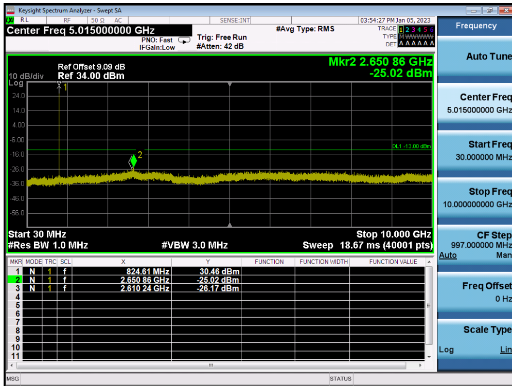
LTE Band 5 / 5MHz / 64QAM - RB Size/Offset (1/0) - Low Channel
