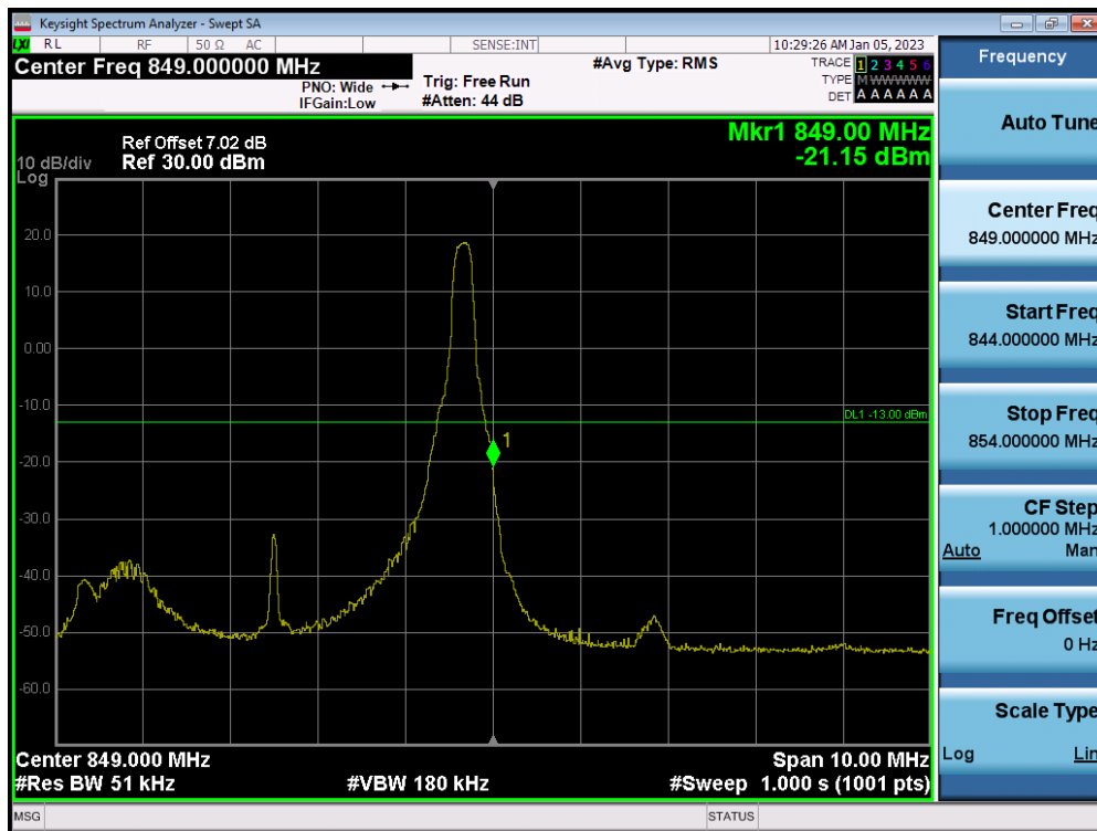
LTE Band 5 / 5MHz / QPSK - RB Size/Offset (1/24)
