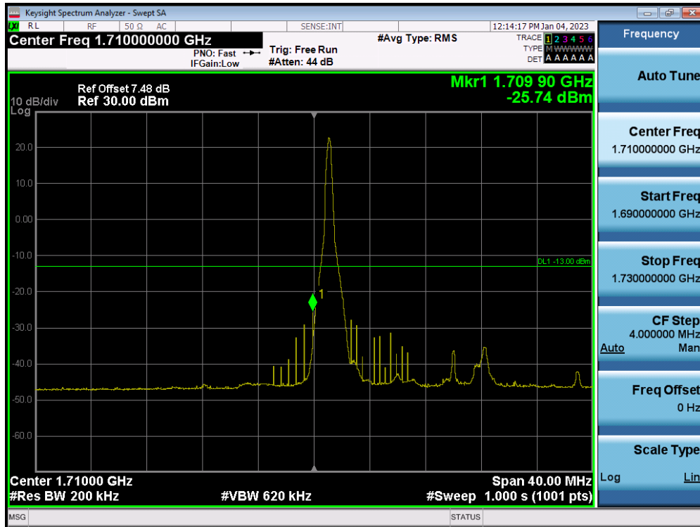
LTE Band 66(4) / 20MHz / QPSK - RB Size/Offset (1/0)
