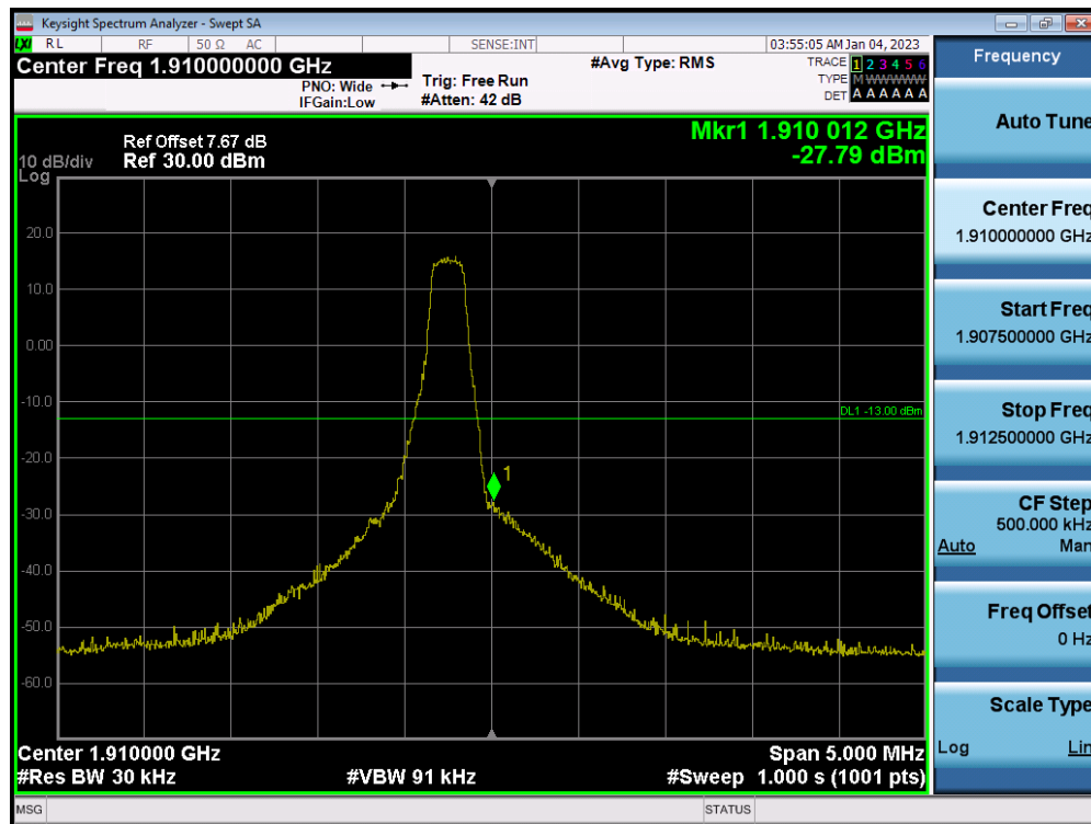
LTE Band 2 / 1.4MHz / 64QAM - RB Size/Offset (1/5)
