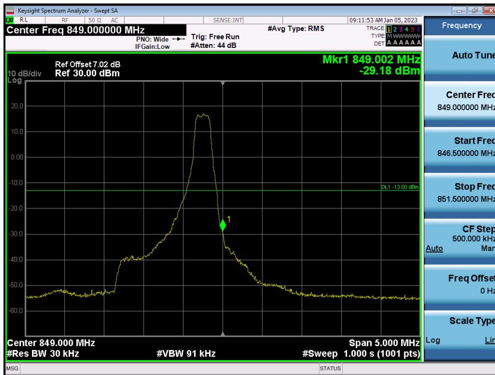
LTE Band 5 / 1.4MHz / QPSK - RB Size/Offset (1/5)
