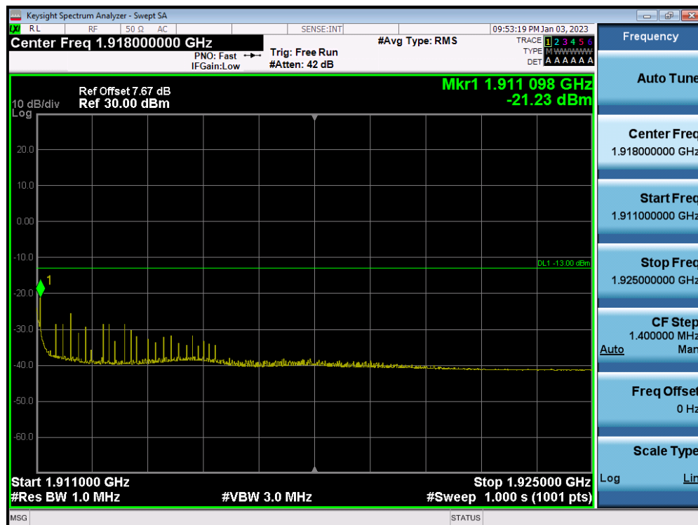
LTE Band 2 / 15MHz / QPSK - RB Size/Offset (1/74)
