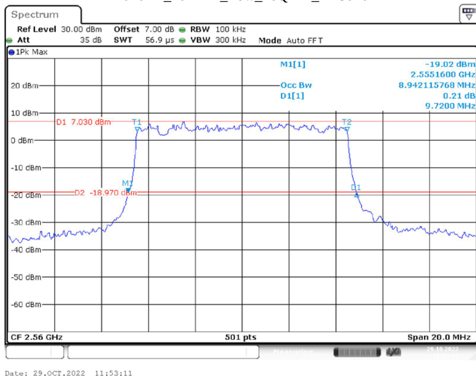
Band 41_10 MHz_Low_16QAM_RB50#0
