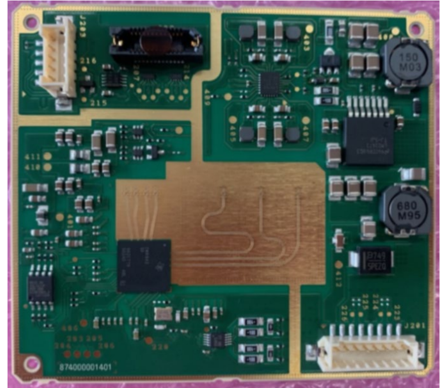
Back (Component side)
