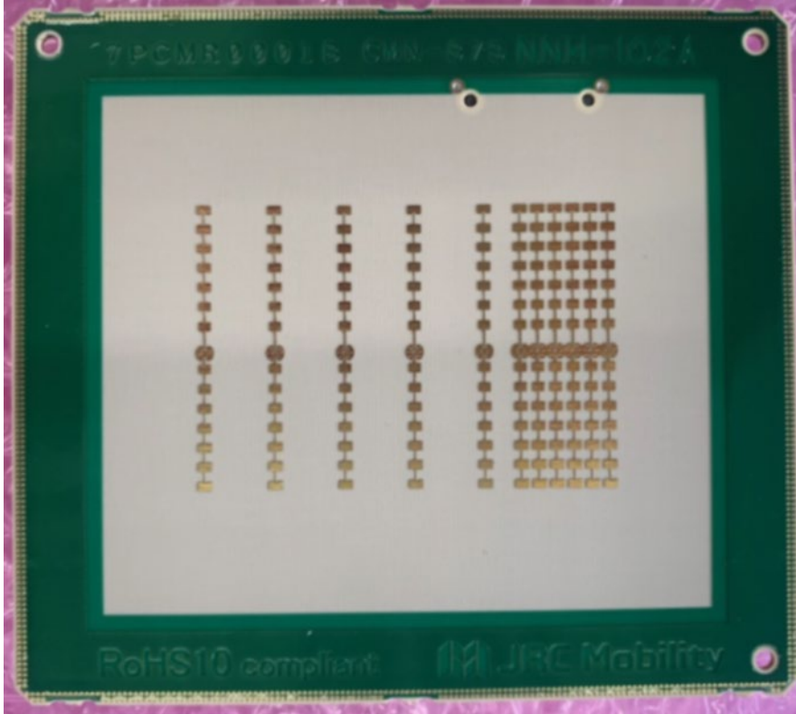
Front (Antenna side)
