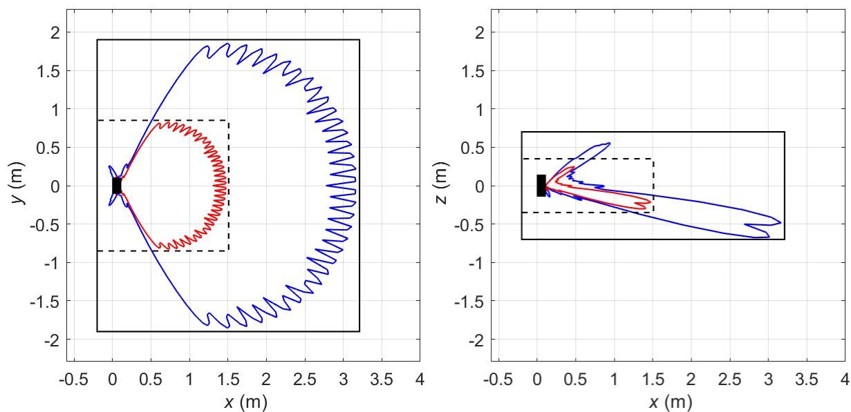
Figure 18 Compliance boundaries for general public (black solid line) and workers (black dashed line) exposure for markets where the FCC exposure limits apply for Macro7 (tilt 11.25°) sector shape (Configuration Mode 2). The blue solid lines correspond to compliance distance results for general public exposure obtained using the spherical models. The solid red lines indicate the corresponding compliance distance results for workers exposure. The EUT is shown from above (left) and from the side (right) with its backplane located at x = 0 m. Mode: B260 (39 GHz) (NR). Total EIRP of the radio: 61.2 dBm.
