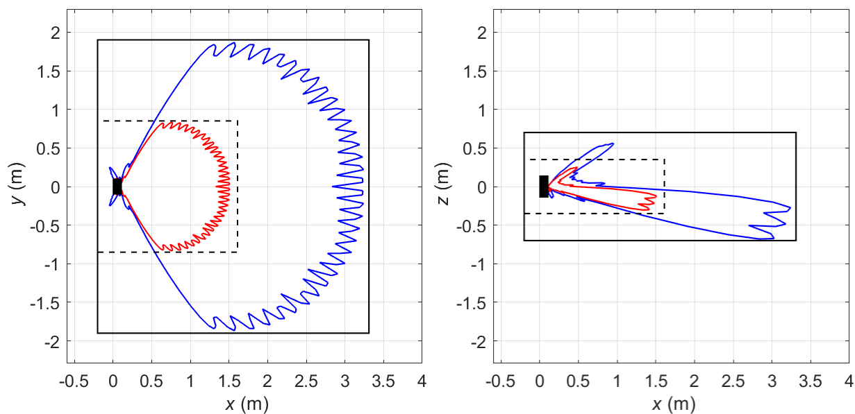
Figure 20 Compliance boundaries for general public (black solid line) and workers (black dashed line) exposure for markets where the FCC exposure limits apply for Macro13 (tilt 7.5°) sector shape (Configuration Mode 2). The blue solid lines correspond to compliance distance results for general public exposure obtained using the spherical models. The solid red lines indicate the corresponding compliance distance results for workers exposure. The EUT is shown from above (left) and from the side (right) with its backplane located at x = 0 m. Mode: B260 (39 GHz) (NR). Total EIRP of the radio: 61.2 dBm.
