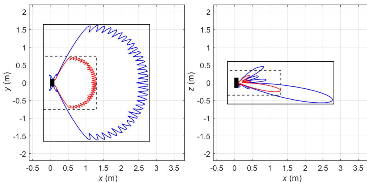
Figure 10 Compliance boundaries for general public (black solid line) and workers (black dashed line) exposure for markets where the FCC exposure limits apply for Macro9 (tilt 7.5°) sector shape (Configuration Mode 1). The blue solid lines correspond to compliance distance results for general public exposure obtained using the spherical models. The solid red lines indicate the corresponding compliance distance results for workers exposure. The EUT is shown from above (left) and from the side (right) with its backplane located at x = 0 m. Mode: B260 (39 GHz) (NR). Total EIRP of the radio: 60.2 dBm.
