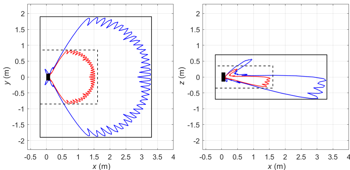
Figure 16 Compliance boundaries for general public (black solid line) and workers (black dashed line) exposure for markets where the FCC exposure limits apply for Macro5 (tilt 7.5°) sector shape (Configuration Mode 2). The blue solid lines correspond to compliance distance results for general public exposure obtained using the spherical models. The solid red lines indicate the corresponding compliance distance results for workers exposure. The EUT is shown from above (left) and from the side (right) with its backplane located at x = 0 m. Mode: B260 (39 GHz) (NR). Total EIRP of the radio: 61.2 dBm.
