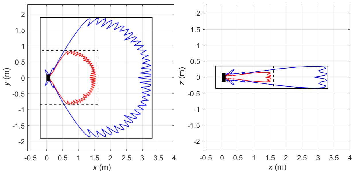
Figure 15 Compliance boundaries for general public (black solid line) and workers (black dashed line) exposure for markets where the FCC exposure limits apply for Macro5 sector shape (Configuration Mode 2). The blue solid lines correspond to compliance distance results for general public exposure obtained using the spherical models. The solid red lines indicate the corresponding compliance distance results for workers exposure. The EUT is shown from above (left) and from the side (right) with its backplane located at x = 0 m. Mode: B260 (39 GHz) (NR). Total EIRP of the radio: 61.2 dBm.
