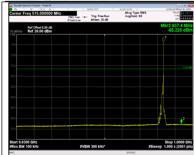
5-5-10MHz-10MHz-64QAM-64QAM-20501-20600-1RB#4 9-0RB#0-30~1000MHz-PASS
