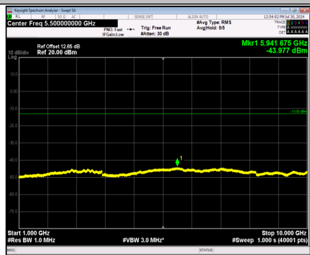
5-5-10MHz-10MHz-64QAM-64QAM-20501-20600-50RB#0- 50RB#0-1000~10000MHz-PASS
