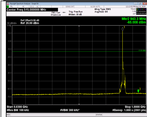
5-5-10MHz-10MHz-16QAM-16QAM-20501-20600-1RB#0 -ORB#0-30~1000MHz-PASS
