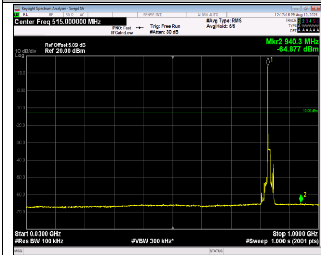
5-5-10MHz-10MHz-QPSK-QPSK-20501-20600-1RB#0-0 RB#0-30~1000MHz-PASS
