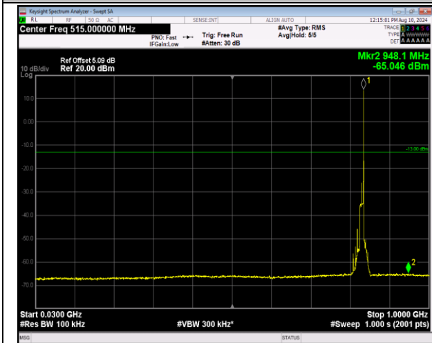
5-5-10MHz-10MHz-16QAM-16QAM-20501-20600-1RB#4 9-ORB#0-30~1000MHz-PASS
