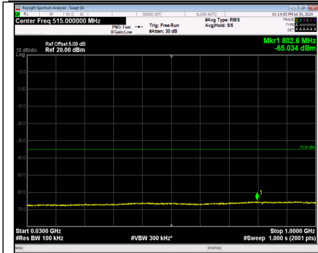
7-7-10MHz-20MHz-64QAM-64QAM-20805-20949-1RB#4 9-0RB#0-30~1000MHz-PASS
