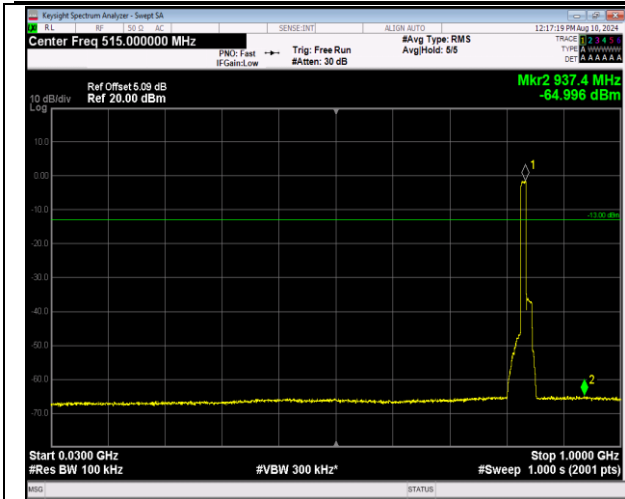
5-5-10MHz-10MHz-16QAM-16QAM-20501-20600-50RB# 0-50RB#0-30~1000MHz-PASS
