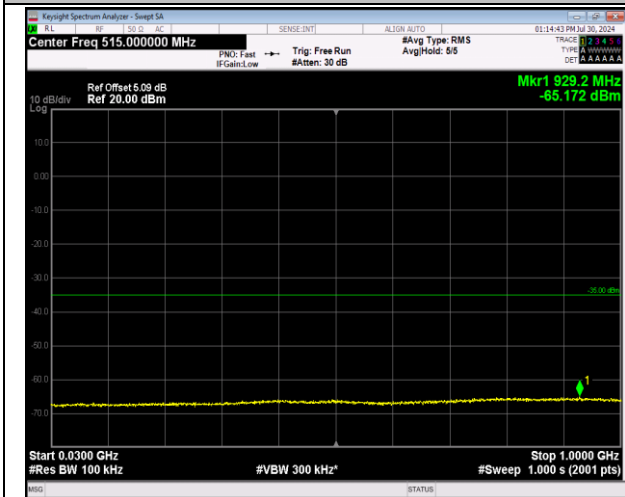
7-7-10MHz-20MHz-64QAM-64QAM-20805-20949-1RB#0 -1RB#99-30~1000MHz-PASS
