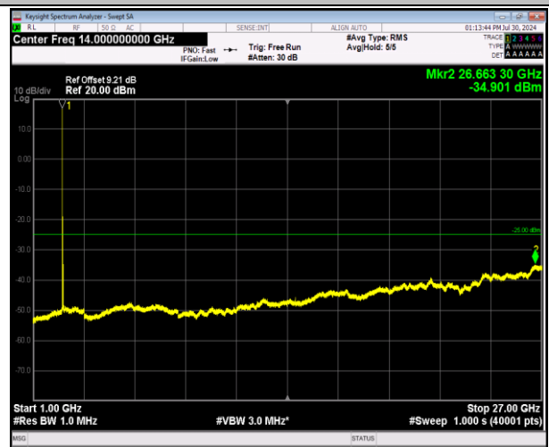
7-7-10MHz-20MHz-64QAM-64QAM-20805-20949-1RB#0-0 RB#0-1000~27000MHz-PASS
