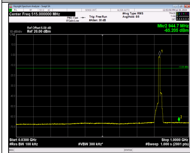
5-5-10MHz-10MHz-64QAM-64QAM-20501-20600-50RB#- 0-50RB#0-30~1000MHz-PASS
