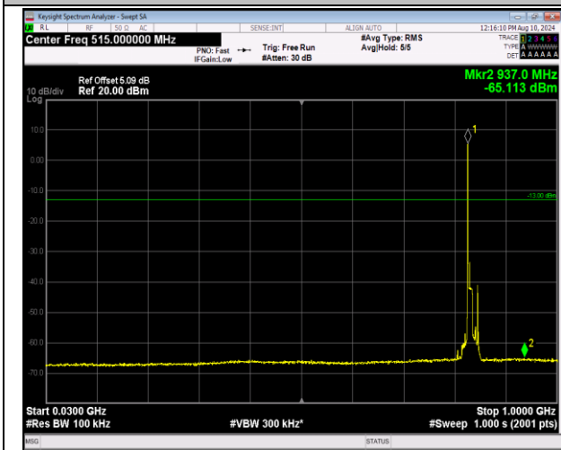
5-5-10MHz-10MHz-16QAM-16QAM-20501-20600-1RB#0 -1RB#49-30~1000MHz-PASS
