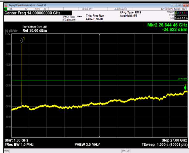
7-7-10MHz-20MHz-QPSK-QPSK-21006-21150-50RB#0-10 ORB#0-1000~27000MHz-PASS
