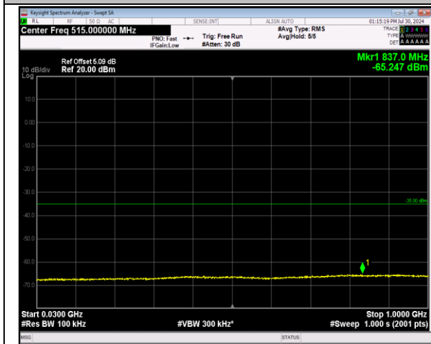
7-7-10MHz-20MHz-64QAM-64QAM-20805-20949-50RB#- 0-100RB#0-30~1000MHz-PASS
