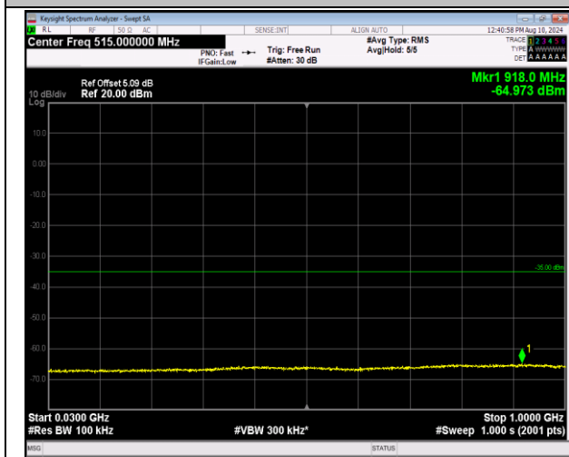
7-7-10MHz-20MHz-QPSK-QPSK-20805-20949-1RB#49- 0RB#0-30~1000MHz-PASS
