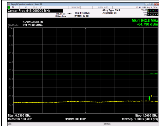
7-7-10MHz-20MHz-16QAM-16QAM-20805-20949-1RB#49 9-ORB#0-30~1000MHz-PASS
