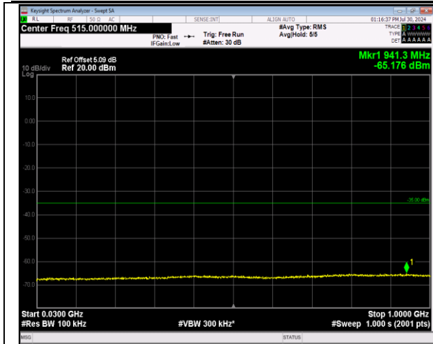
7-7-10MHz-20MHz-64QAM-64QAM-21006-21150-1RB#4 9-0RB#0-30~1000MHz-PASS
