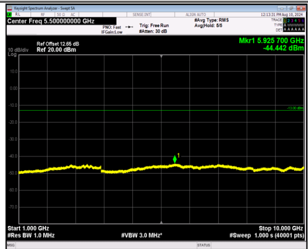
5-5-10MHz-10MHz-QPSK-QPSK-20501-20600-1RB#0-0RB #0-1000~10000MHz-PASS
