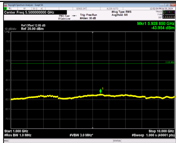
5-5-10MHz-10MHz-64QAM-64QAM-20501-20600-1RB#49- 0RB#0-1000~10000MHz-PASS
