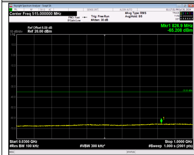
7-7-10MHz-20MHz-64QAM-64QAM-21006-21150-50RB#- 0-100RB#0-30~1000MHz-PASS
