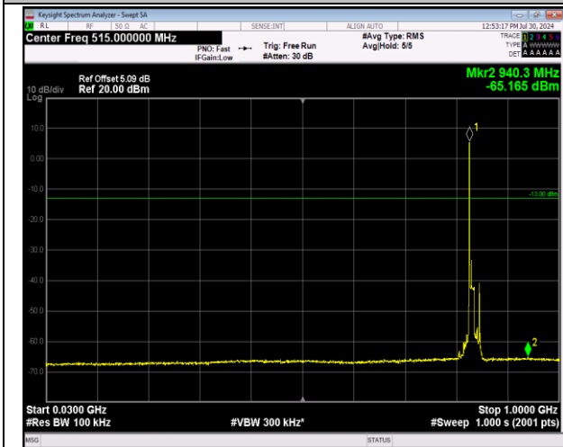
5-5-10MHz-10MHz-64QAM-64QAM-20501-20600-1RB#0 -1RB#49-30~1000MHz-PASS
