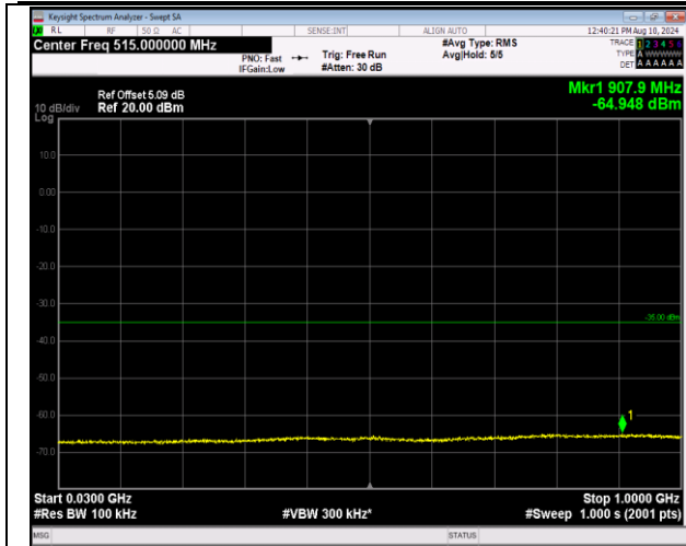
7-7-10MHz-20MHz-16QAM-16QAM-20805-20949-1RB#0 -ORB#0-30~1000MHz-PASS
