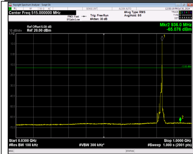
5-5-10MHz-10MHz-64QAM-64QAM-20476-20575-1RB#4 9-0RB#0-30~1000MHz-PASS
