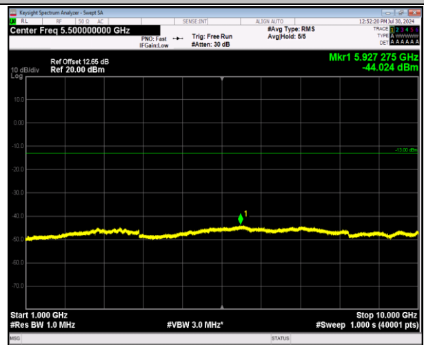
5-5-10MHz-10MHz-64QAM-64QAM-20501-20600-1RB#0-0 RB#0-1000~10000MHz-PASS
