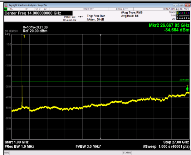
7-7-10MHz-20MHz-16QAM-16QAM-21006-21150-1RB#49- 0RB#0-1000~27000MHz-PASS
