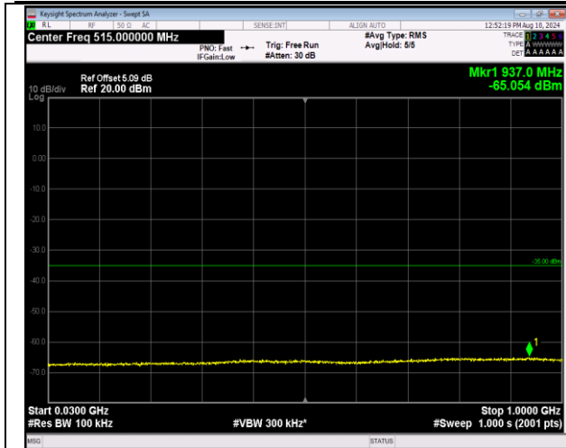
7-7-10MHz-20MHz-QPSK-QPSK-21206-21350-1RB#0-1 RB#99-30~1000MHz-PASS
