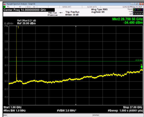
7-7-10MHz-20MHz-16QAM-16QAM-20805-20949-1RB#49- ORB#0-1000~27000MHz-PASS
