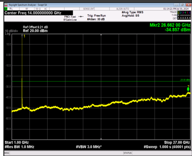
7-7-10MHz-20MHz-64QAM-64QAM-20805-20949-1RB#49- 0RB#0-1000~27000MHz-PASS
