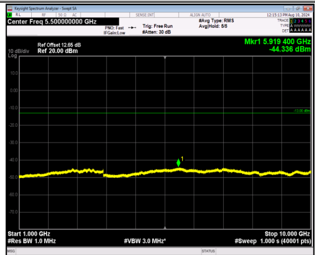
5-5-10MHz-10MHz-16QAM-16QAM-20501-20600-1RB#49- ORB#0-1000~10000MHz-PASS
