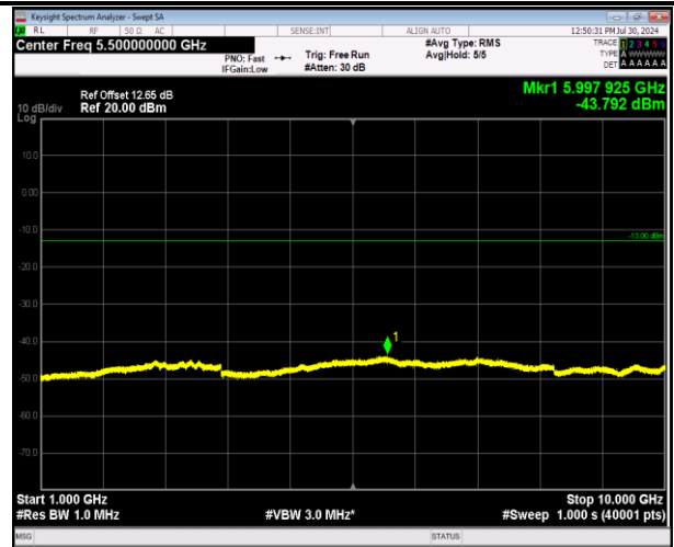
5-5-10MHz-10MHz-64QAM-64QAM-20476-20575-1RB#49- 0RB#0-1000~10000MHz-PASS
