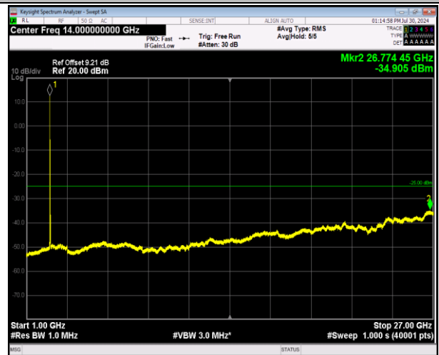
7-7-10MHz-20MHz-64QAM-64QAM-20805-20949-1RB#0-1 RB#99-1000~27000MHz-PASS
