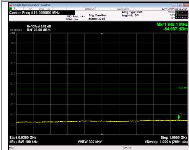
7-7-10MHz-20MHz-16QAM-16QAM-21006-21150-1RB#4 9-0RB#0-30~1000MHz-PASS
