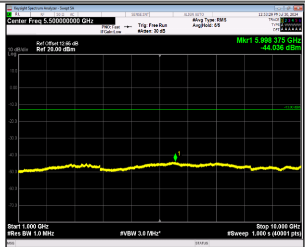
5-5-10MHz-10MHz-64QAM-64QAM-20501-20600-1RB#0-1 RB#49-1000~10000MHz-PASS
