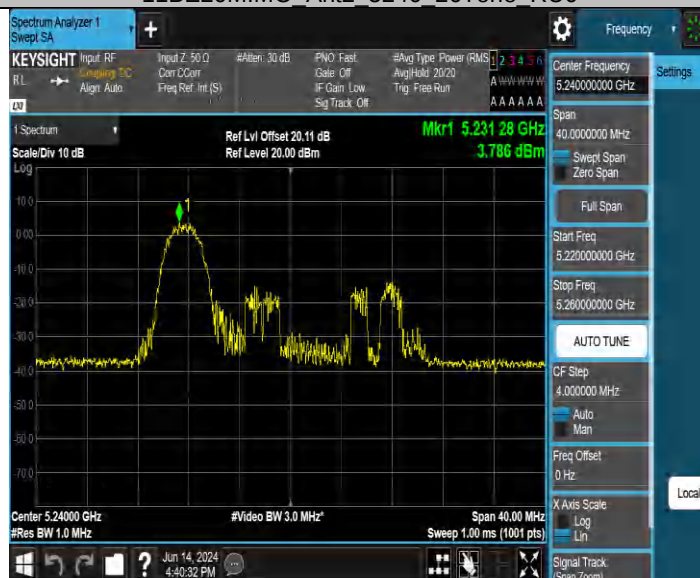
11BE20MIMO Ant2 5240 106Tone RU53
