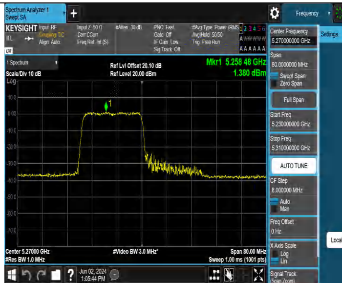
11BE40MIMO Ant4 5270 26Tone RU0
