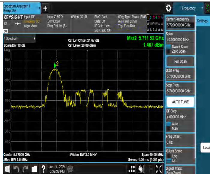
11BE20MIMO Ant3 5720 UNII-2C 106Tone RU53
