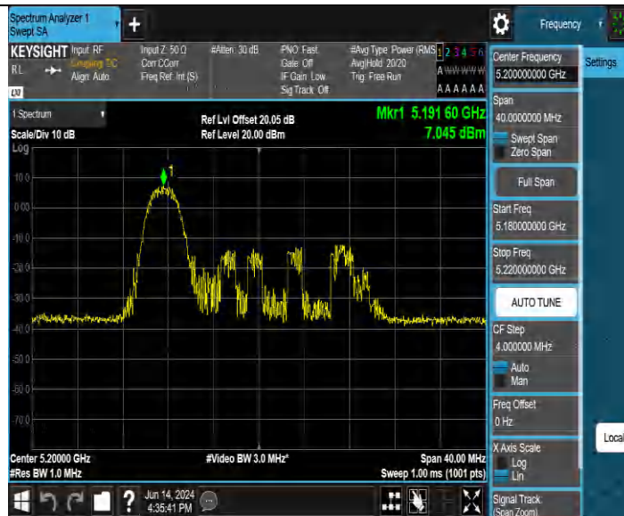
11BE20MIMO Ant2 5200 106Tone RU53
