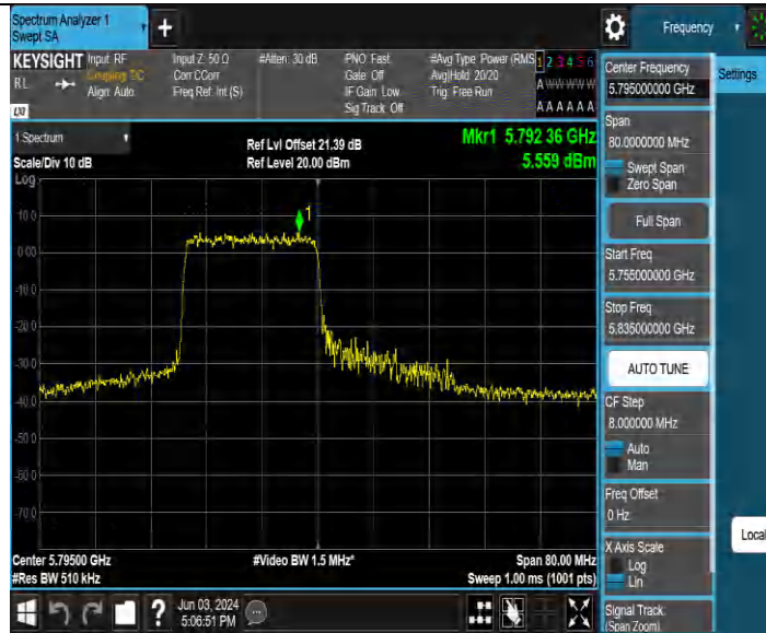
11BE40MIMO Ant2 5795 26Tone RU0
