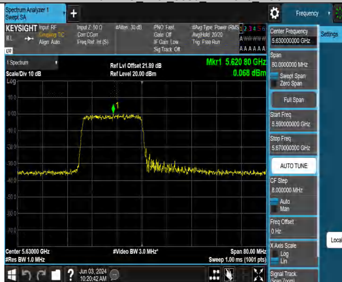
11BE40MIMO Ant3 5630 26Tone RU0
