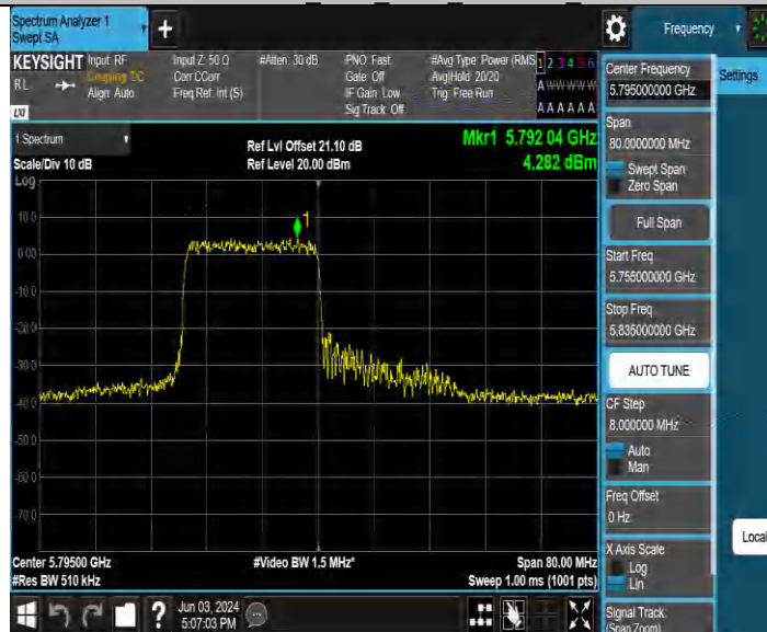
11BE40MIMO Ant3 5795 26Tone RU0
