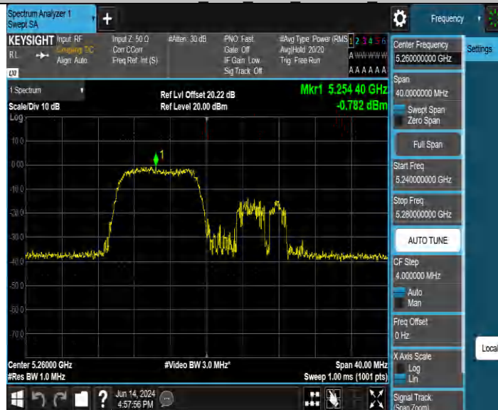
11BE20MIMO Ant3 5260 26Tone RU0
