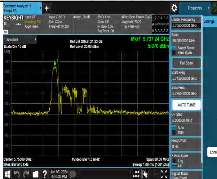
11BE40MIMO Ant2 5755 242Tone RU61
