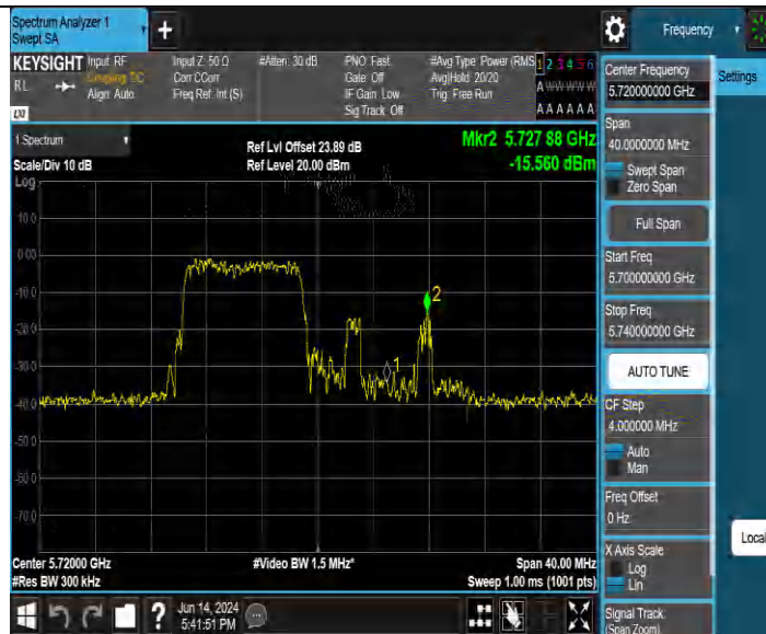
11BE20MIMO Ant4 5720 UNII-3 26Tone RU0
