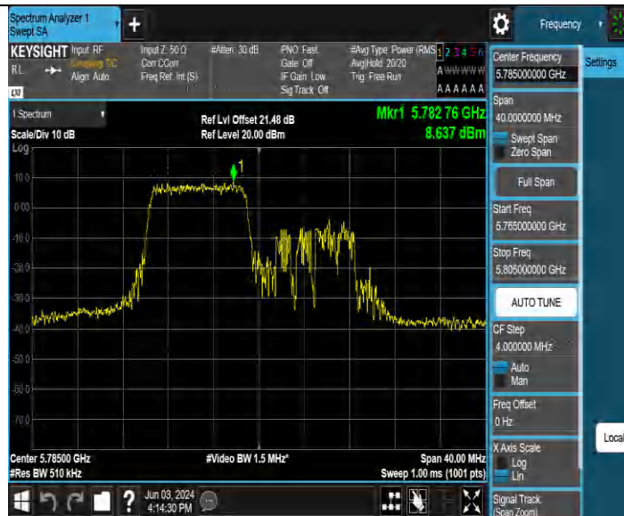
11BE20MIMO Ant2 5785 26Tone RU0
