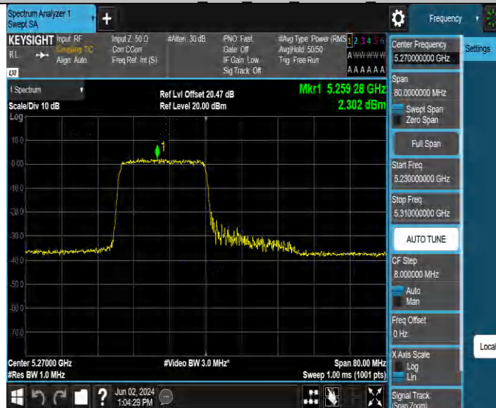
11BE40MIMO Ant2 5270 26Tone RU0
