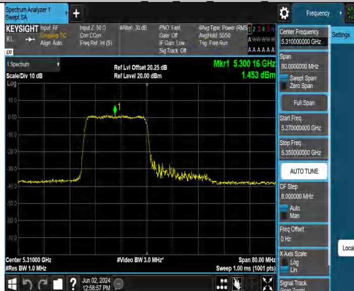
11BE40MIMO Ant4 5310 26Tone RU0
