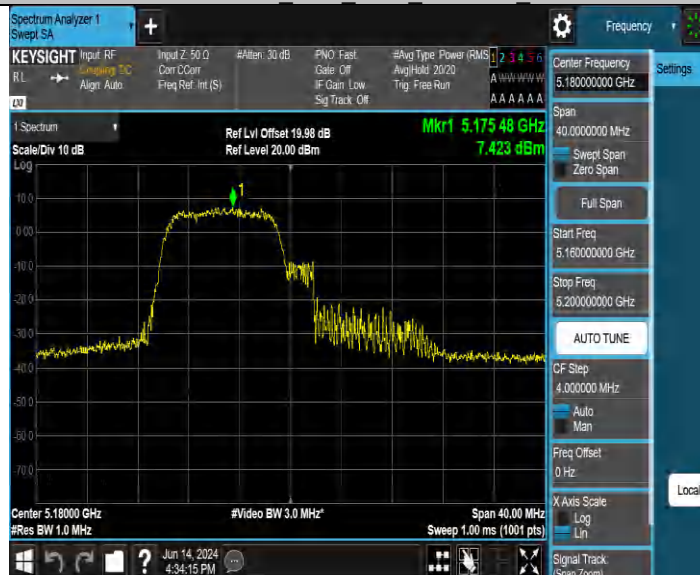
11BE20MIMO Ant3 5180 26Tone RU0
