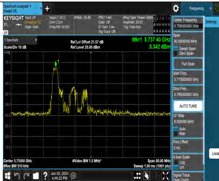
11BE40MIMO Ant1 5755 242Tone RU61
