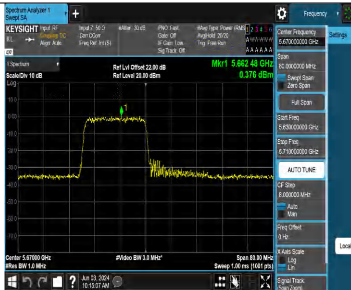
11BE40MIMO Ant3 5670 26Tone RU0
