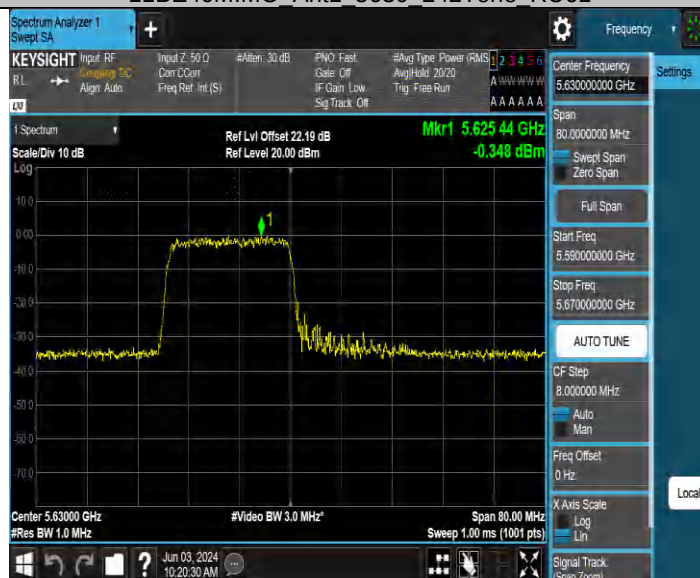
11BE40MIMO Ant2 5630 26Tone RU0
