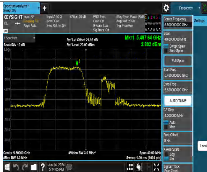
11BE20MIMO Ant2 5500 26Tone RU0
