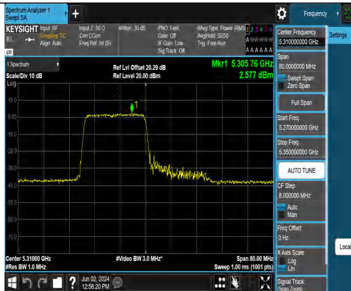
11BE40MIMO Ant3 5310 26Tone RU0
