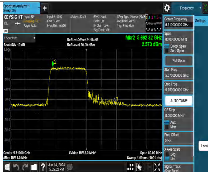
11BE40MIMO Ant1 5710 UNII-3 26Tone RU0
