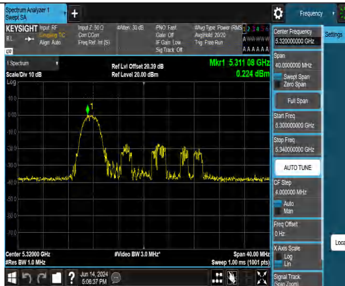
11BE20MIMO Ant4 5320 106Tone RU53
