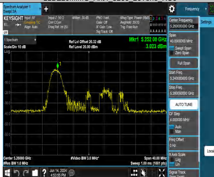
11BE20MIMO Ant4 5260 106Tone RU53
