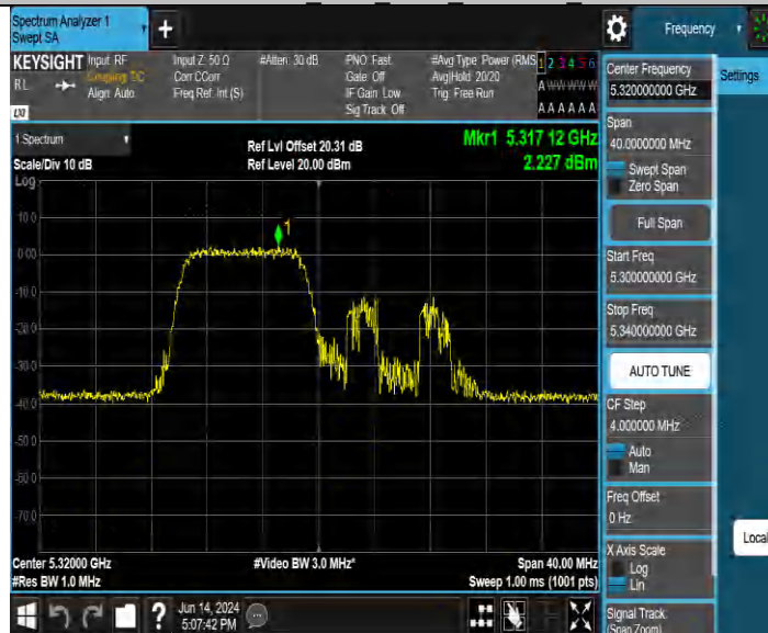
11BE20MIMO Ant4 5320 26Tone RU0
