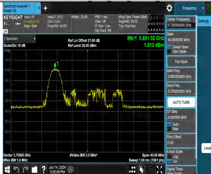
11BE20MIMO Ant3 5700 106Tone RU53
