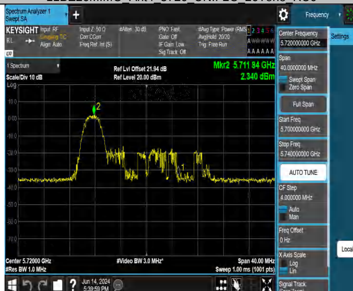
11BE20MIMO Ant4 5720 UNII-2C 106Tone RU53
