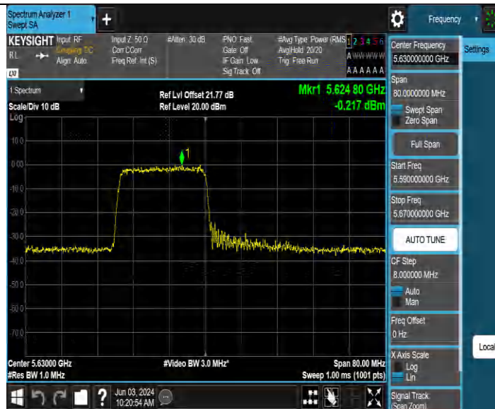
11BE40MIMO Ant4 5630 26Tone RU0
