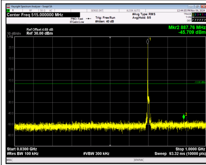
Band17-10MHz-QPSK-23780-1RB#0-Range1:30~100 OMHz
