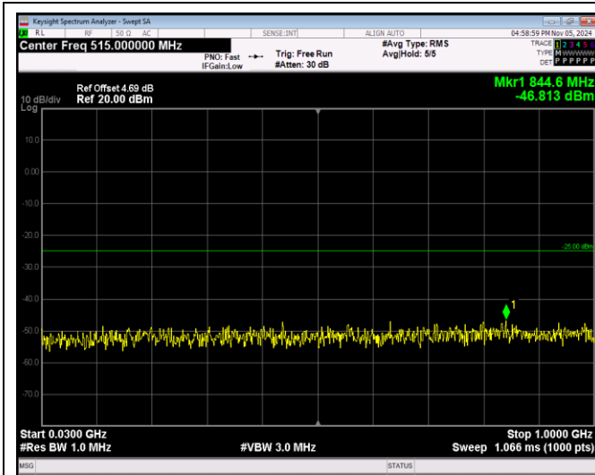
Band38-5MHz-16QAM-38225-1RB#0-Range1:30~100 OMHz
