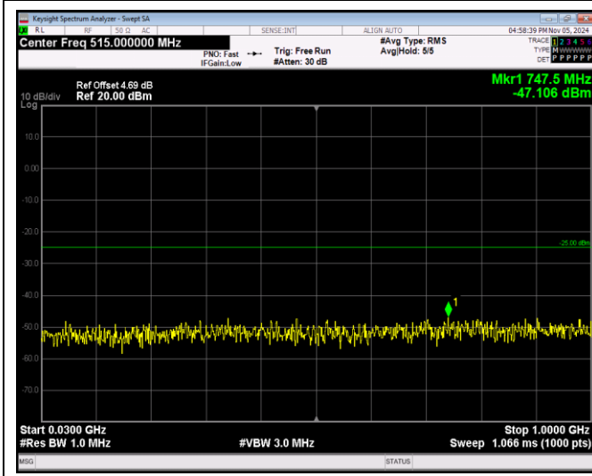
Band38-5MHz-QPSK-38000-1RB#0-Range1:30~1000 MHz
