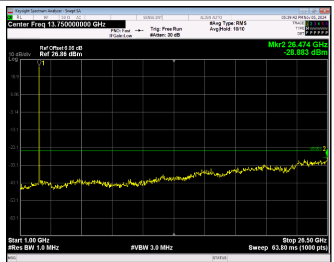
Band38-20MHz-16QAM-38150-1RB#0-Range2:1000~26500MHz
