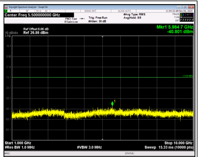
Band12-10MHz-64QAM-23095-1RB#0-Range2:1000~10000MHz
