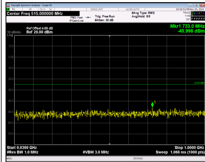
Band38-5MHz-64QAM-37775-1RB#0-Range1:30~100 OMHz
