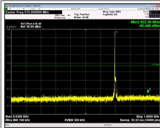
Band17-10MHz-16QAM-23790-1RB#0-Range1:30~1000MHz
