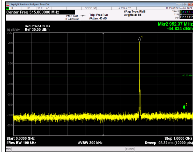
Band17-10MHz-QPSK-23780-1RB#0-Range1:30~100 OMHz
