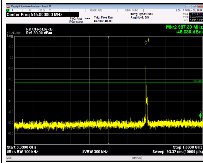
Band12-10MHz-64QAM-23130-1RB#0-Range1:30~1000MHz
