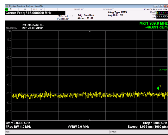
Band38-20MHz-64QAM-37850-1RB#0-Range1:30~1000MHz
