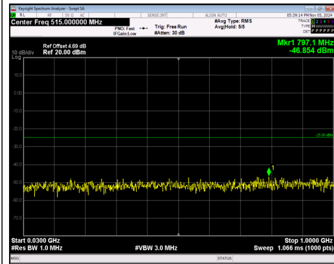
Band38-20MHz-QPSK-38150-1RB#0-Range1:30~100 OMHz
