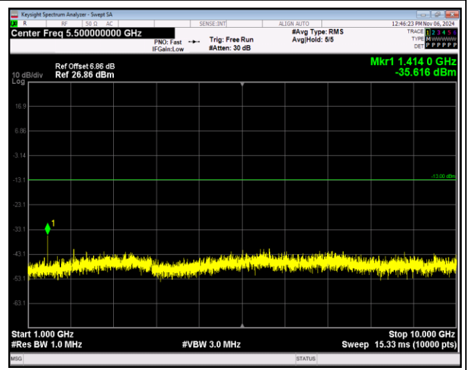
Band17-10MHz-16QAM-23800-1RB#0-Range2:1000~10000MHz
