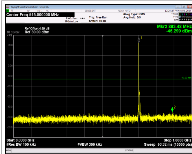
Band17-5MHz-16QAM-23755-1RB#0-Range1:30~100 OMHz
