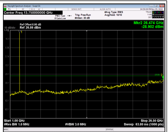
Band38-5MHz-16QAM-38225-1RB#0-Range2:1000~2 6500MHz
