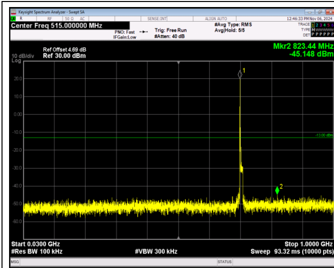
Band38-5MHz-QPSK-37775-1RB#0-Range1:30~1000 MHz
