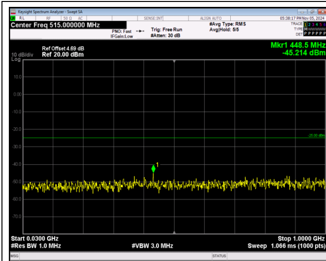
Band38-20MHz-QPSK-38000-1RB#0-Range1:30~100 OMHz
