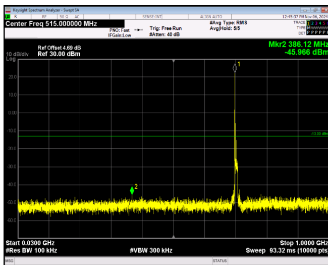
Band17-10MHz-64QAM-23800-1RB#0-Range1:30~1000MHz
