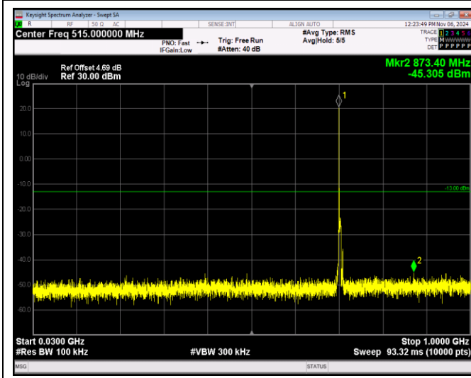
Band17-5MHz-16QAM-23790-1RB#0-Range1:30~100 OMHz
