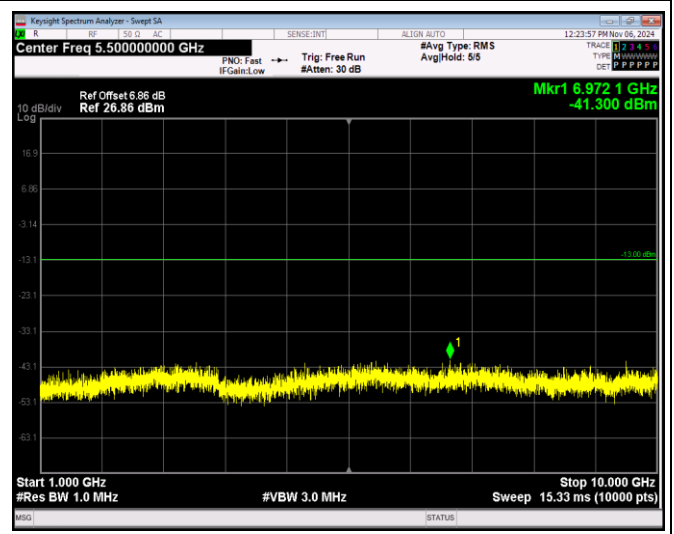
Band17-5MHz-16QAM-23790-1RB#0-Range2:1000~1 0000MHz
