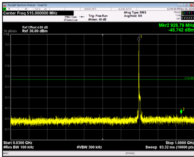
Band17-10MHz-64QAM-23790-1RB#0-Range1:30~1000MHz
