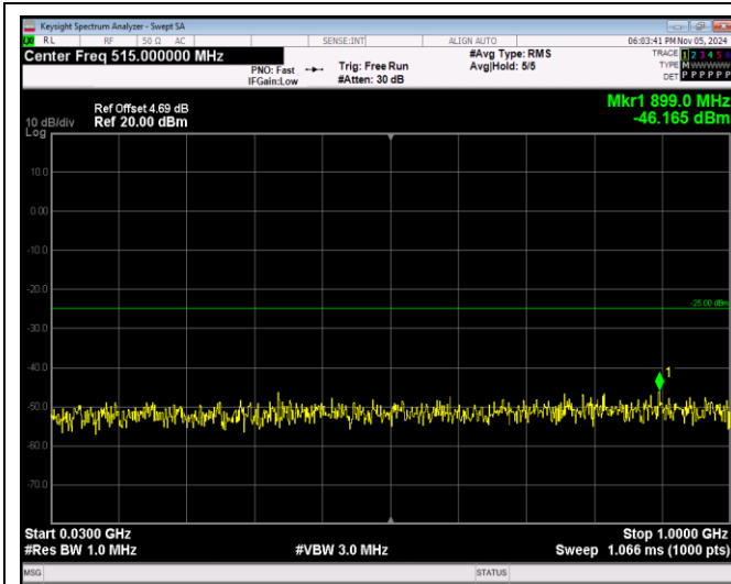
Band41-5MHz-QPSK-41215-1RB#0-Range1:30~1000 MHz
