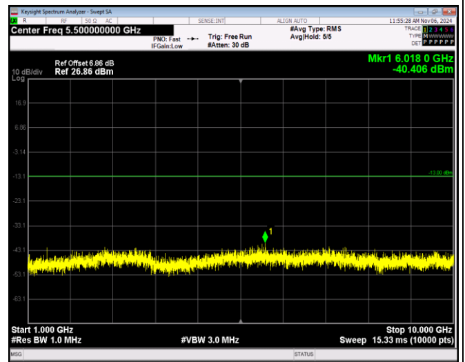
Band12-10MHz-64QAM-23130-1RB#0-Range2:1000~10000MHz
