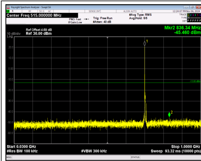
Band17-5MHz-64QAM-23825-1RB#0-Range1:30~100 OMHz
