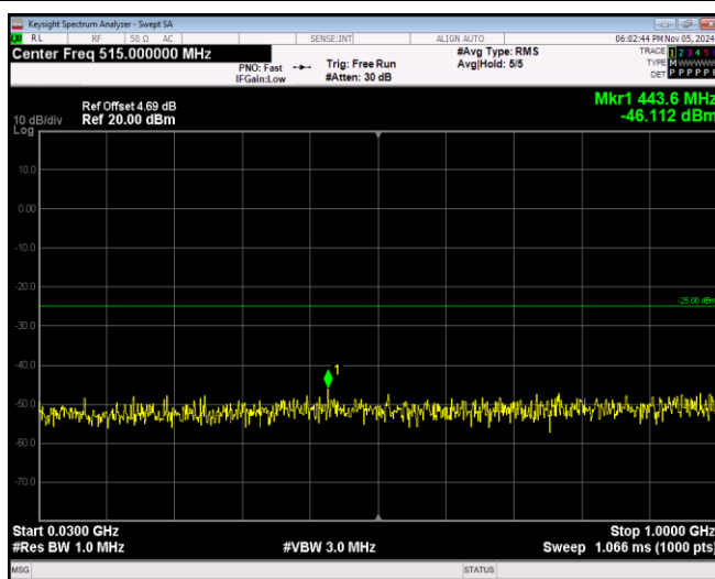
Band41-5MHz-QPSK-40640-1RB#0-Range1:30~1000MHz
