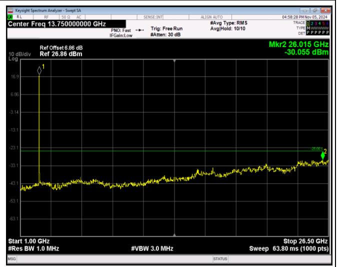
Band38-5MHz-64QAM-37775-1RB#0-Range2:1000~2 6500MHz
