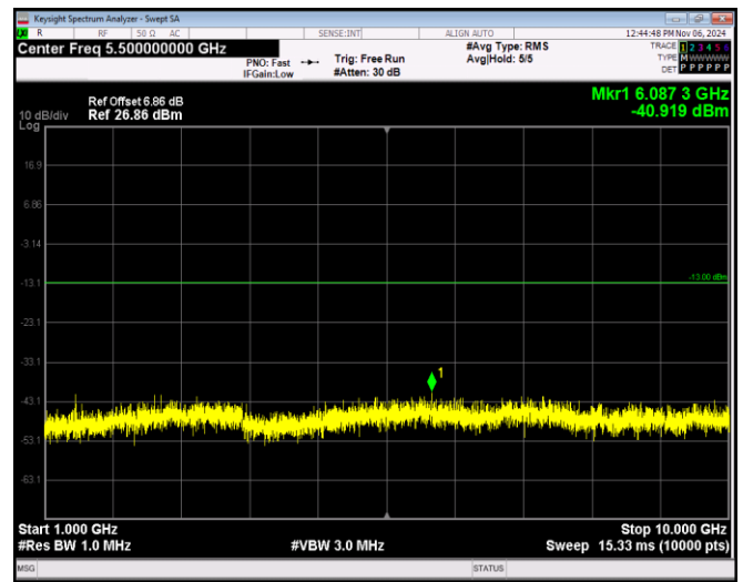
Band17-10MHz-64QAM-23790-1RB#0-Range2:1000~10000MHz
