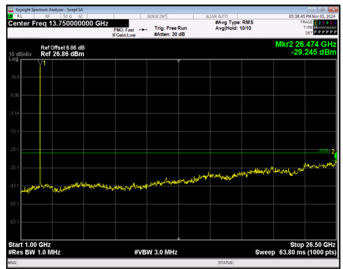
Band38-20MHz-16QAM-38000-1RB#0-Range2:1000~26500MHz
