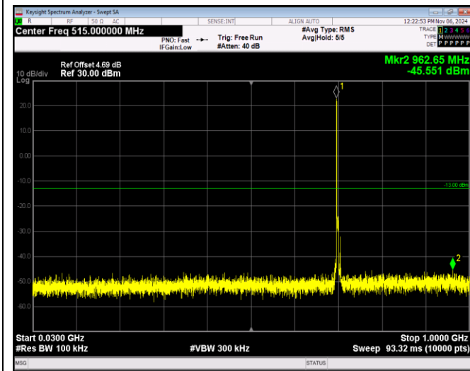
Band17-5MHz-16QAM-23790-1RB#0-Range1:30~100 OMHz
