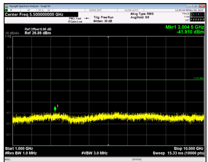
Band17-10MHz-64QAM-23800-1RB#0-Range2:1000~10000MHz
