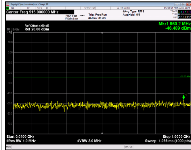
Band38-20MHz-64QAM-38000-1RB#0-Range1:30~1000MHz
