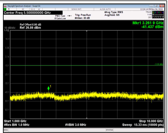
Band17-5MHz-64QAM-23825-1RB#0-Range2:1000~1 0000MHz
