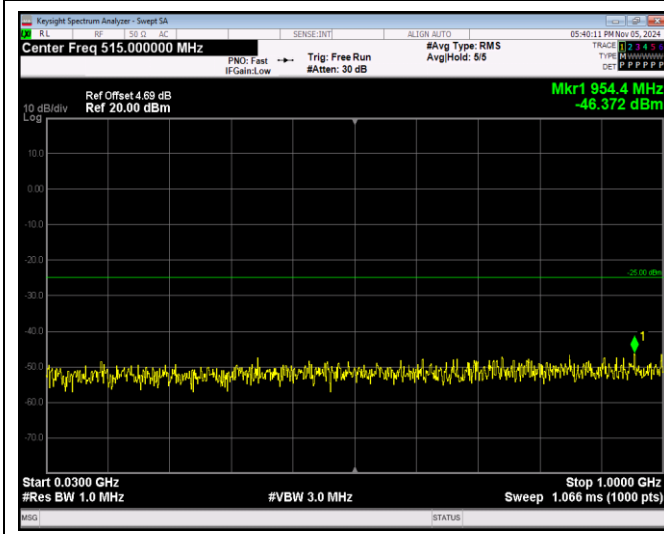
Band38-20MHz-QPSK-38150-1RB#0-Range1:30~100 OMHz
