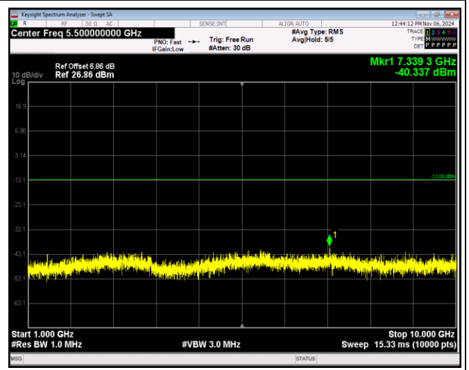
Band17-10MHz-QPSK-23780-1RB#0-Range2:1000~1 0000MHz
