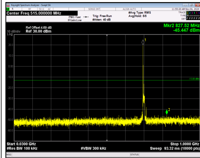
Band12-10MHz-64QAM-23130-1RB#0-Range1:30~1000MHz
