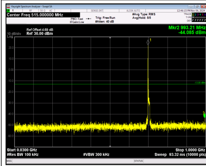
Band17-10MHz-16QAM-23800-1RB#0-Range1:30~1000MHz
