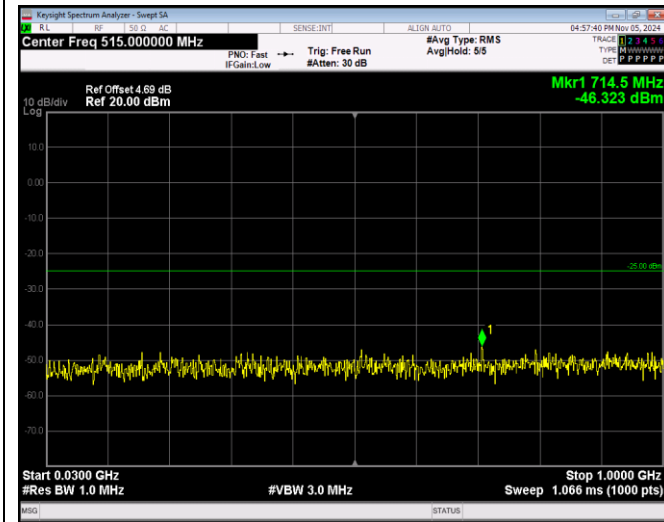
Band38-5MHz-QPSK-38000-1RB#0-Range1:30~1000 MHz
