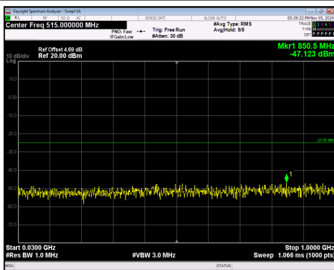
Band38-20MHz-16QAM-38150-1RB#0-Range1:30~1000MHz
