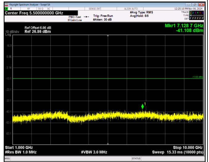
Band17-10MHz-QPSK-23780-1RB#0-Range2:1000~1 0000MHz
