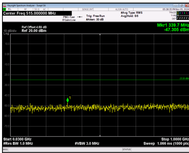
Band38-20MHz-16QAM-38000-1RB#0-Range1:30~1000MHz
