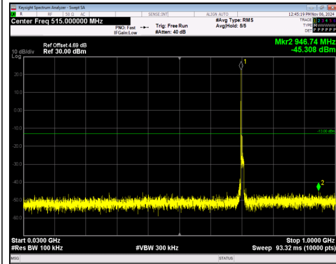
Band17-10MHz-16QAM-23800-1RB#0-Range1:30~1000MHz
