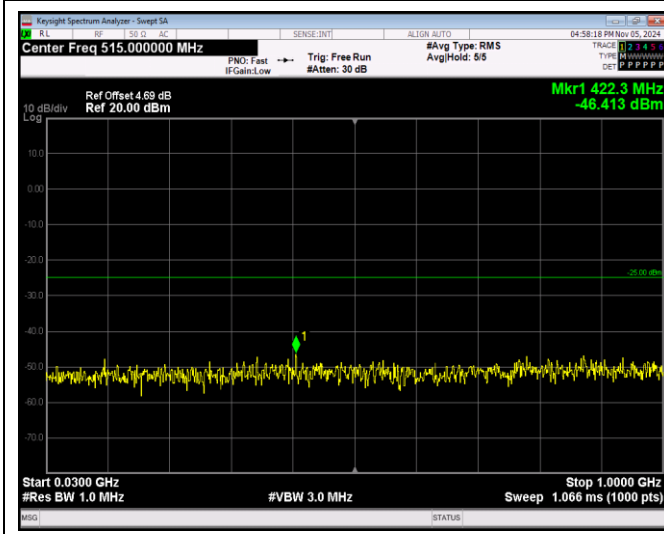
Band38-5MHz-64QAM-37775-1RB#0-Range1:30~100 OMHz
