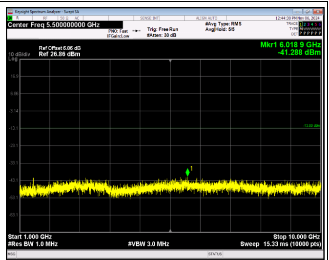
Band17-10MHz-16QAM-23790-1RB#0-Range2:1000~10000MHz
