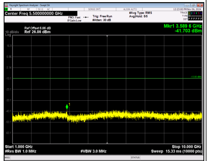
Band17-5MHz-16QAM-23790-1RB#0-Range2:1000~1 0000MHz
