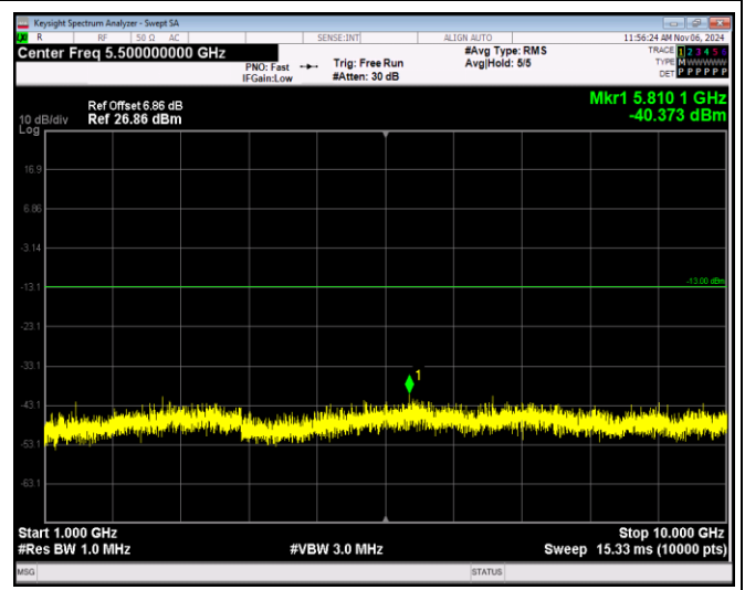
Band12-10MHz-64QAM-23130-1RB#0-Range2:1000~10000MHz
