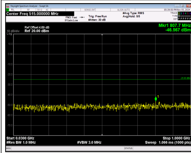
Band38-20MHz-64QAM-38000-1RB#0-Range1:30~1000MHz
