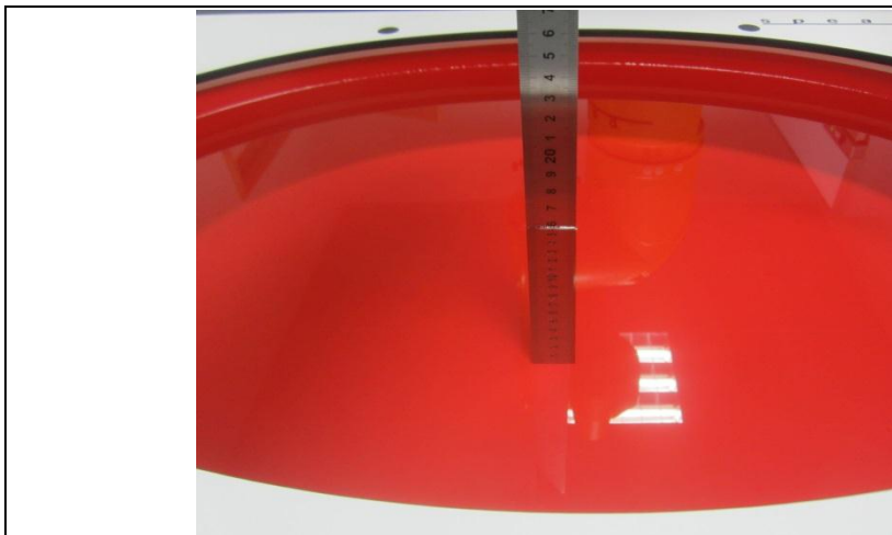
Liquid depth in the ELI Phantom
