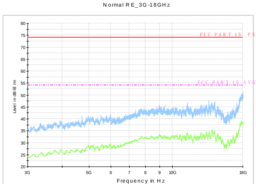
Fig.A.6.2.13 Radiated Spurious Emission (802.11g, Ch1, 3 GHz-18 GHz)
