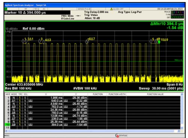
Pulse T_{on}
