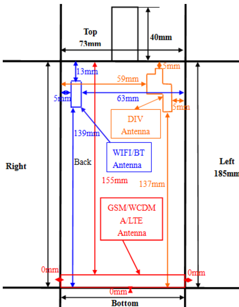
Antenna Configuration 2- LT60H
