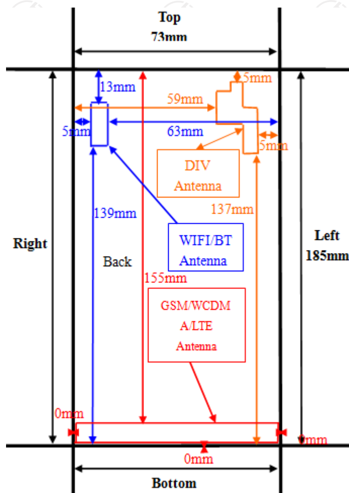
Antenna Configuration 1- LT60
