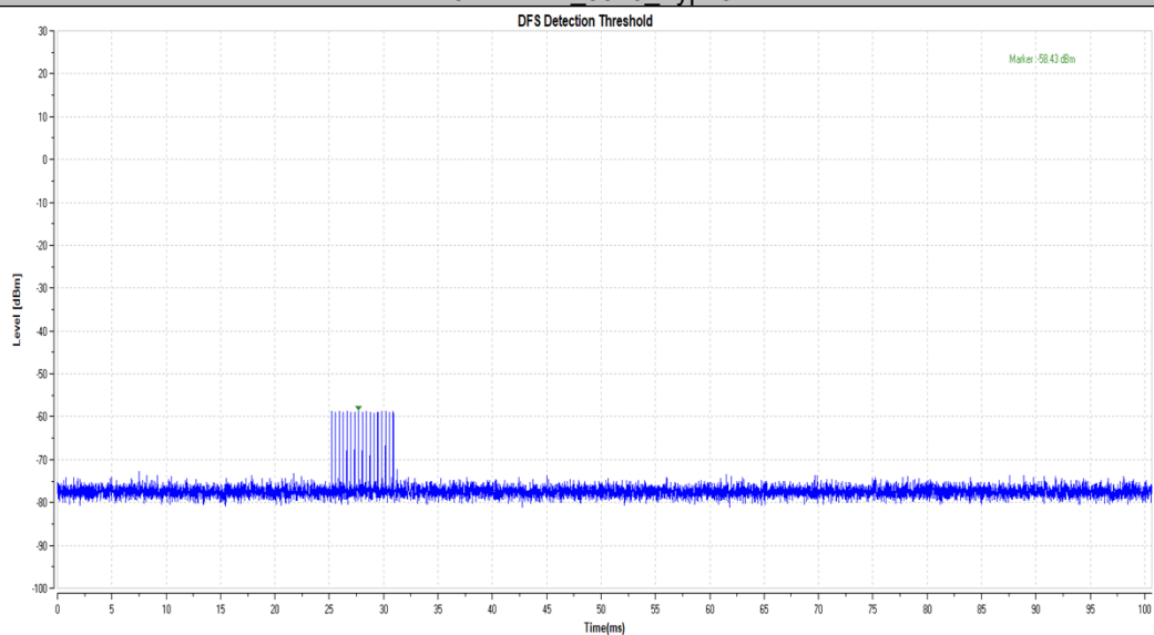
40MHz BW_5510_Type4
