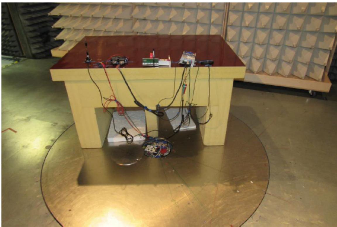
FCC part 24E - near view
