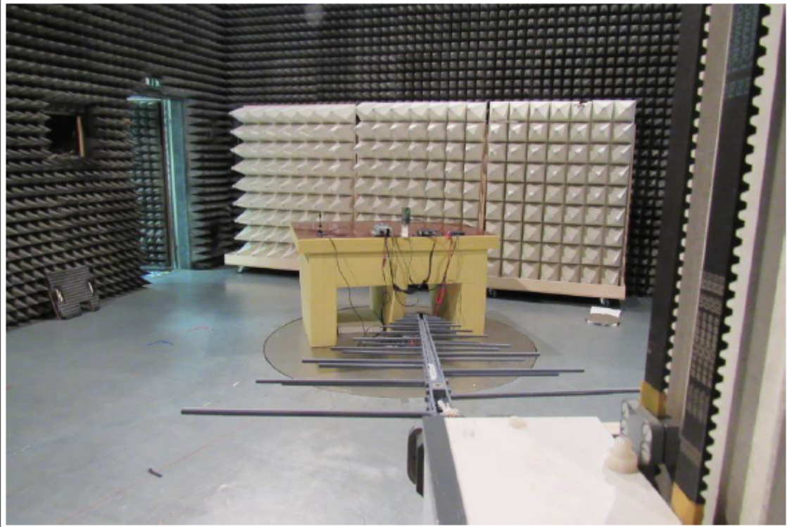
FCC part 22H - Testsetup
