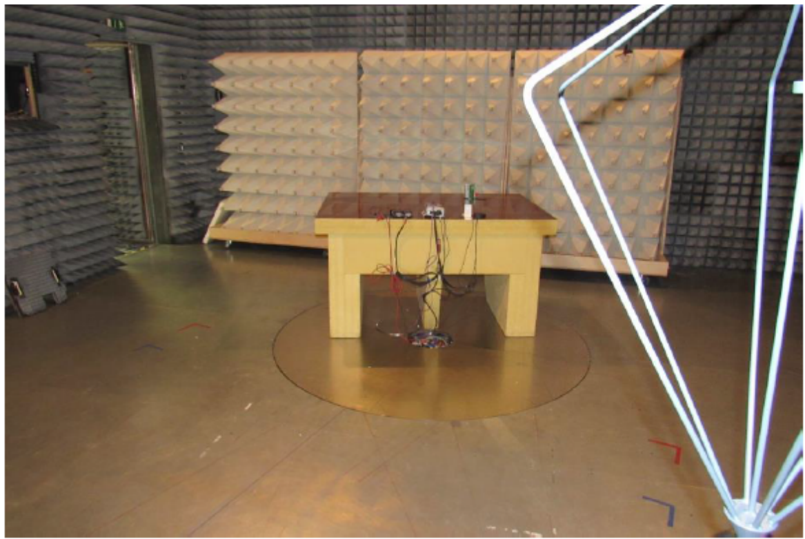
Test setup view from measurement-antenna
