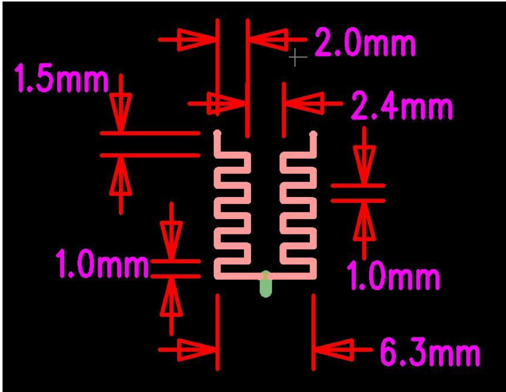
Antenna Photo & Length (mm)
