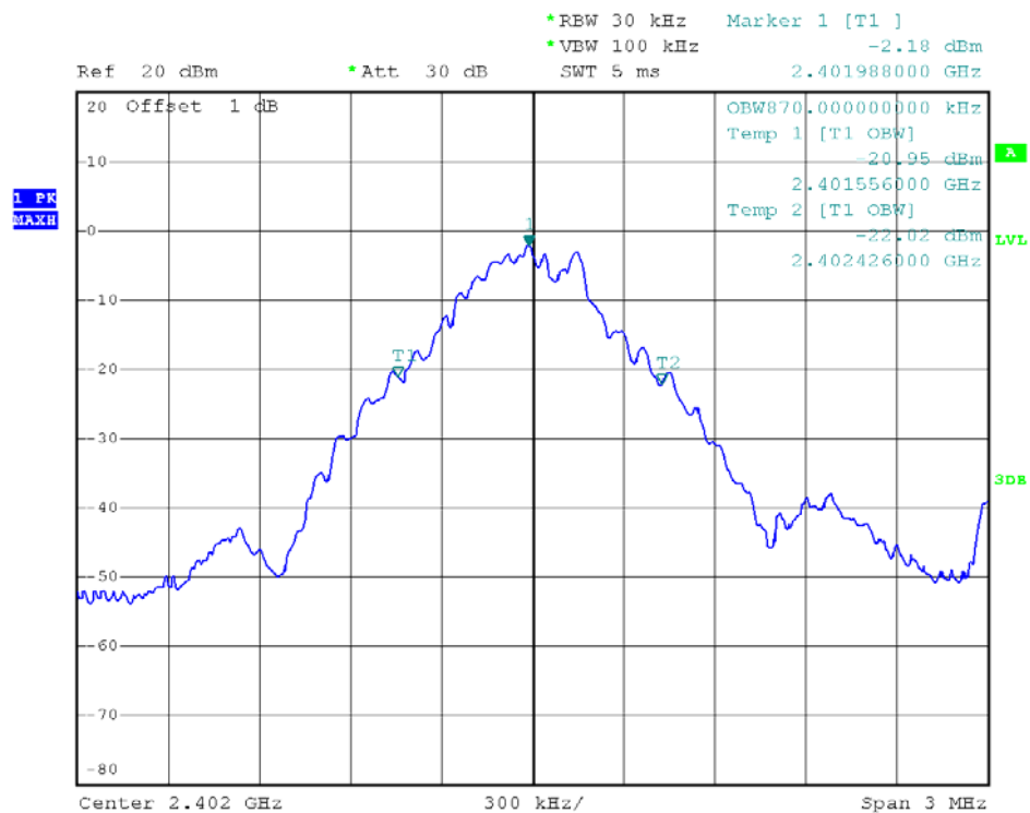
0 Channel @ GFSK
