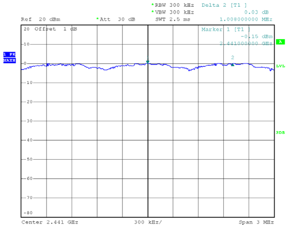
8-DPSK Mode
