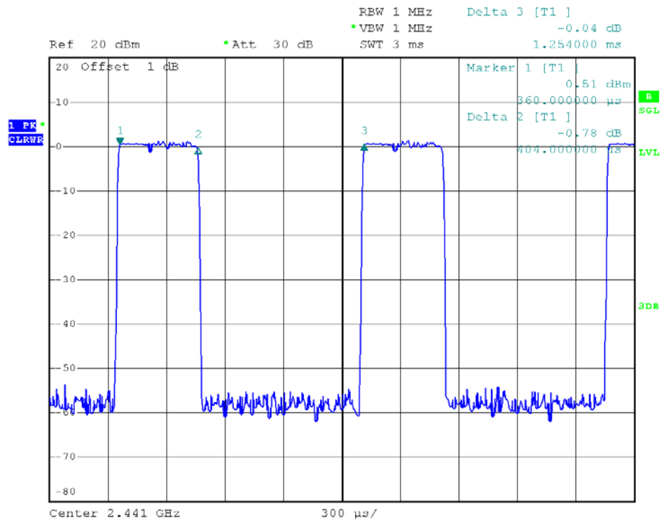
39 Channel @ 3DH1
