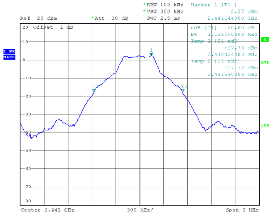
39 Channel @ GFSK
