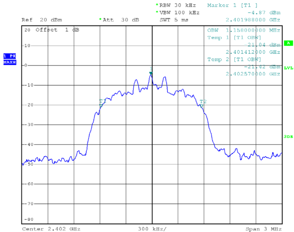
0 Channel @ 8-DPSK
