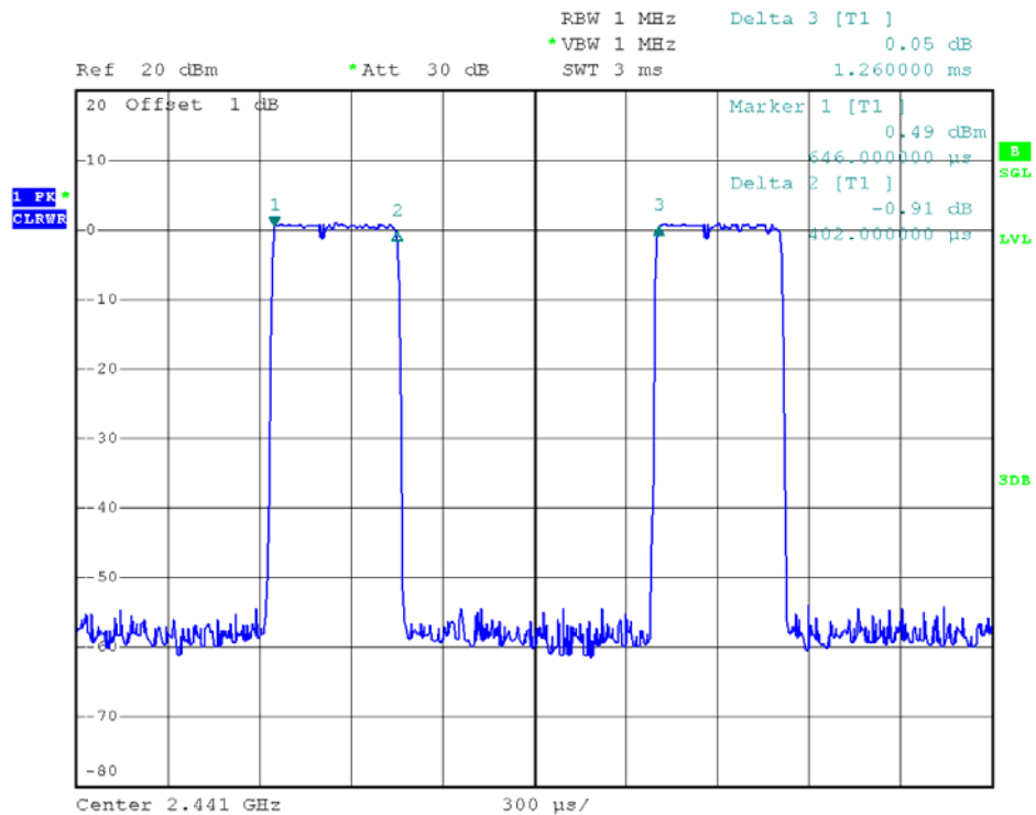
39 Channel @ 2DH1
