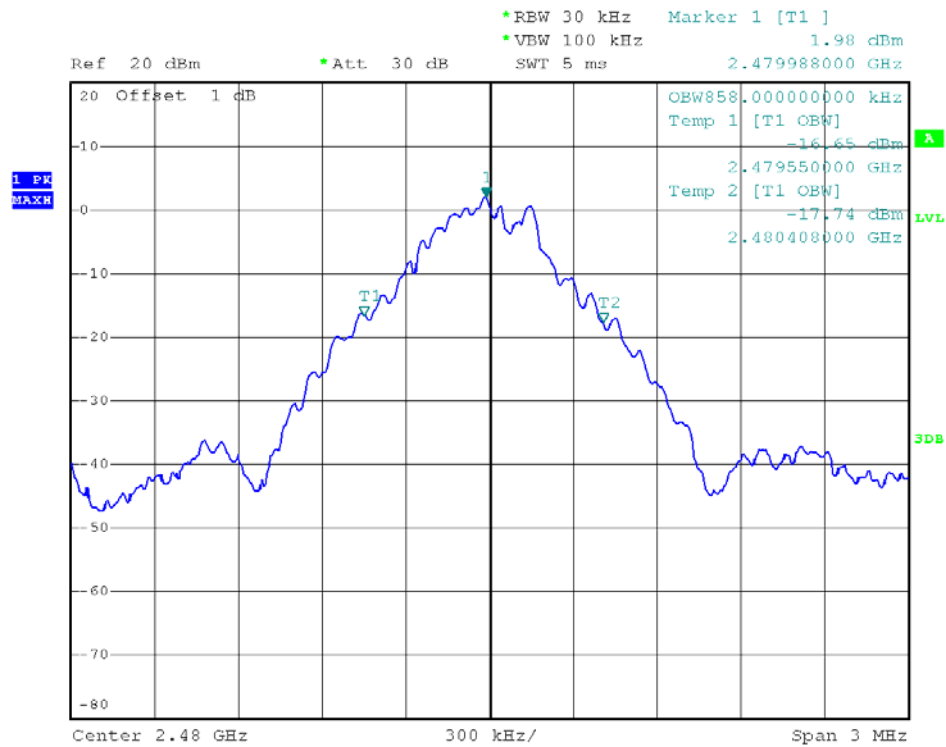
78 Channel @ GFSK
