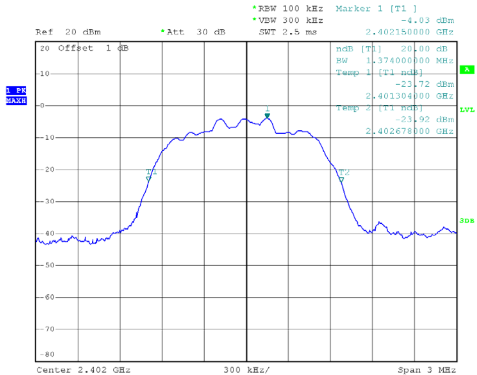
0 Channel @ 8-DPSK
