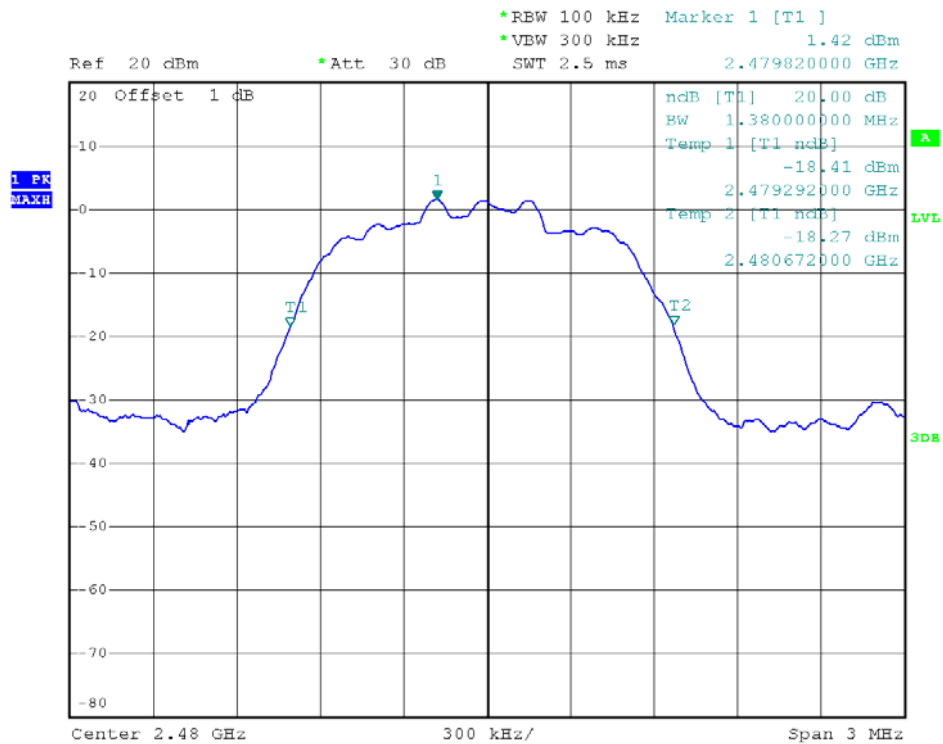
78 Channel @ 8-DPSK
