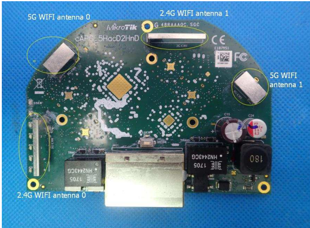
WIFI ANTENNA
