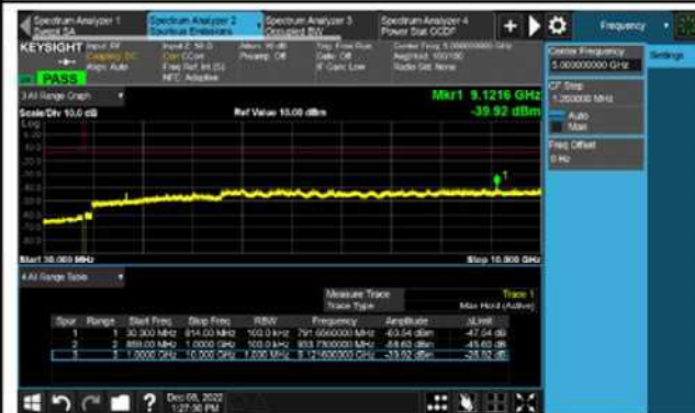
Channel 27025 (847.5MHz)
