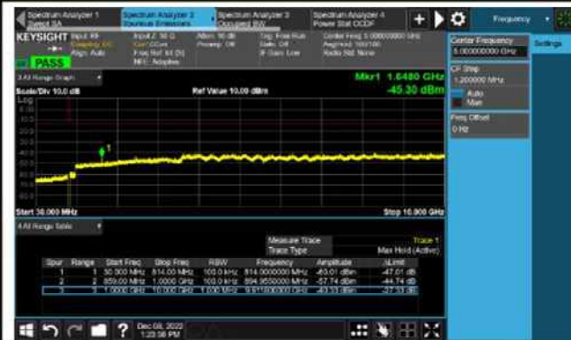
Channel 27033 (848.3MHz)
