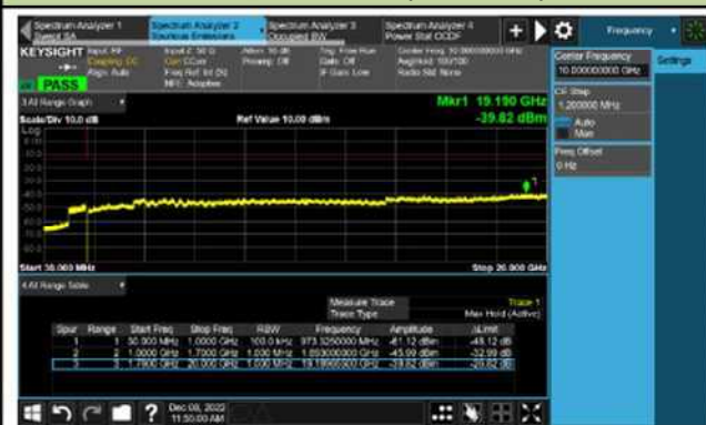
Channel 132622 (1775MHz)
