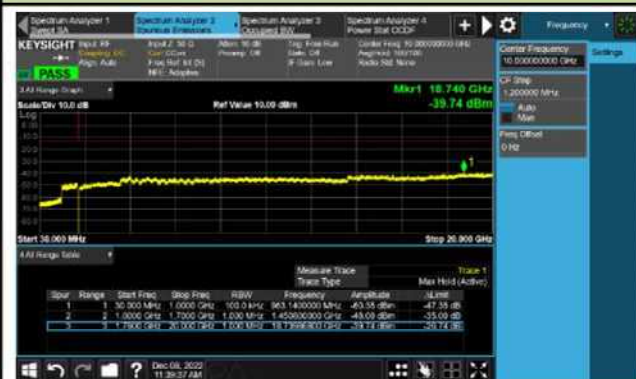
Channel 132665 (1779.3MHz)
