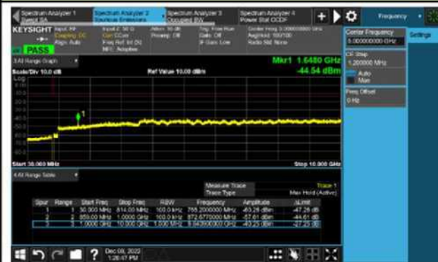
Channel 27025 (847.5MHz)
