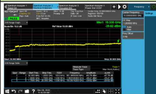
Channel 132657 (1778.5MHz)
