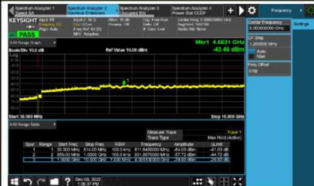
Channel 26965 (841.5MHz)
