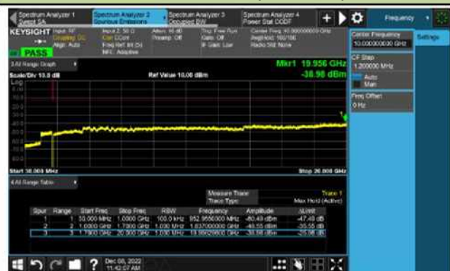
Channel 132322 (1745MHz)
