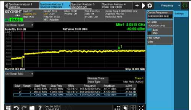
Channel 26915 (836.5MHz)
