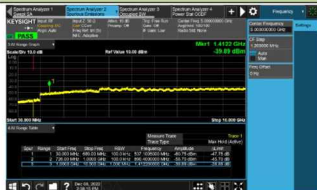
Channel 23095 (707.5MHz)
