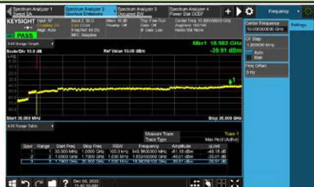
Channel 132322 (1745MHz)
