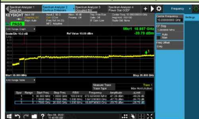
Channel 132665 (1779.3MHz)
