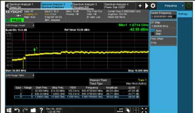
Channel 26915 (836.5MHz)
