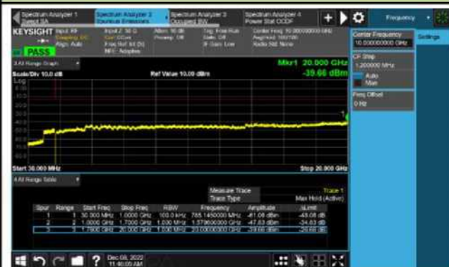
Channel 132647 (1777.5MHz)
