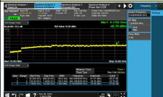
Channel 23165 (714.5MHz)
