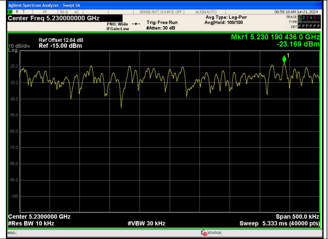
NT/NV_Antenna 0 IEEE 802.11ac_Channel 46_40MHz
