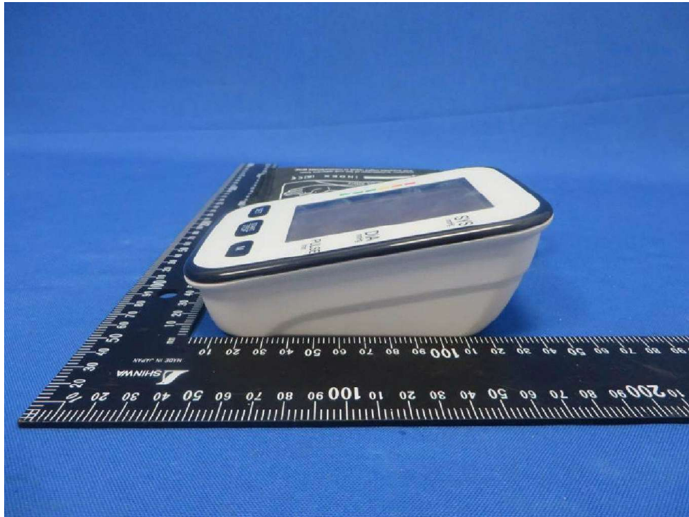
(11) EUT Photo (Model: DBP-1332b)
