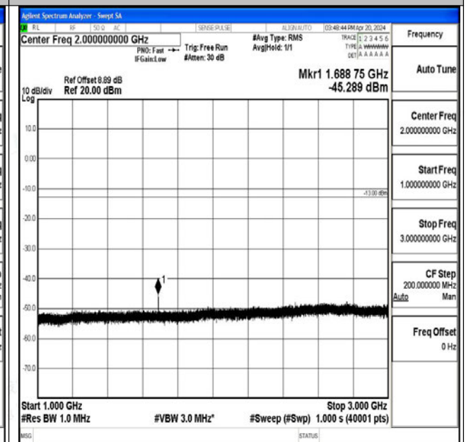
Band26_5MHz_QPSK_27015_1RB#0_1000~3000_1000~3000
