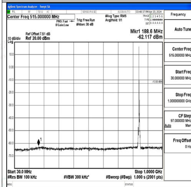
Band26_5MHz_QPSK_27015_1RB#0_30~1000_30~1000
