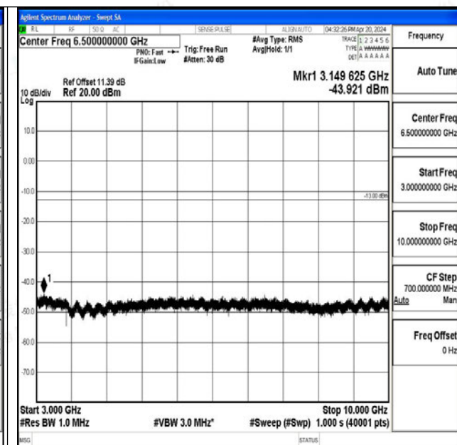
Band26_15MHz_16QAM_26865_1RB#0_3000~10000_3000~10000
