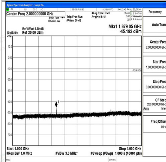
Band26_10MHz_16QAM_26990_1RB#0_1000~3000_1000~3000
