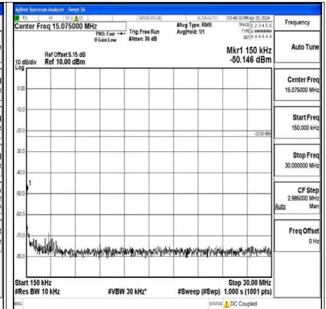
Band26_5MHz_QPSK_27015_1RB#0_0.15~30_0.15~30
