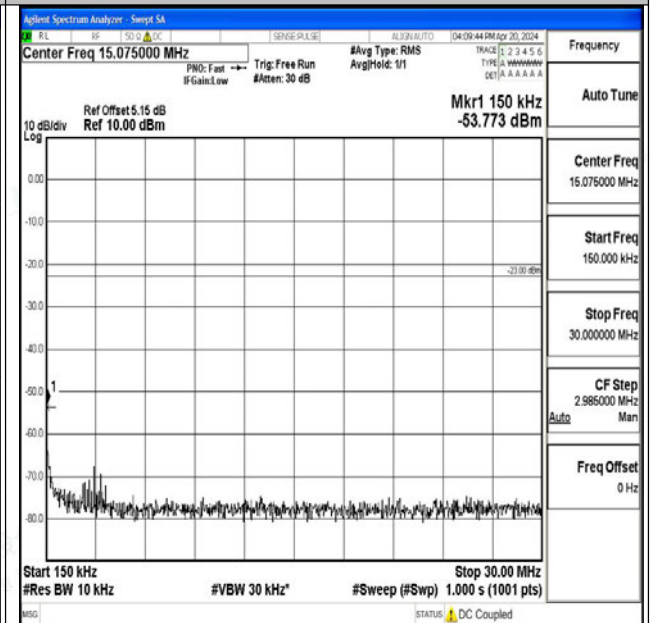
Band26_10MHz_QPSK_26840_1RB#0_0.15~30_0.15~3 0
