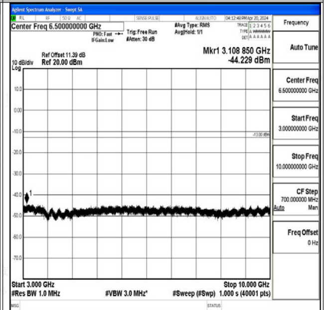
Band26_10MHz_16QAM_26990_1RB#0_3000~10000_3000~10000
