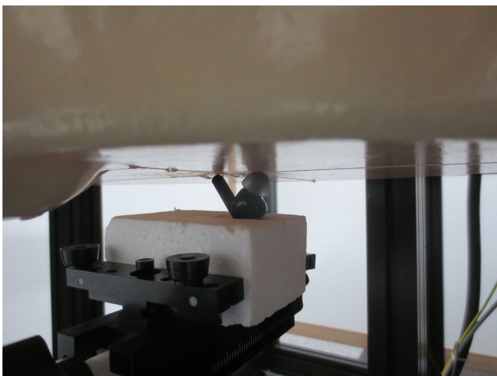
Left Touch & Rear from Flat Phantom (Separation Distance: 0 cm) – Left Ear
