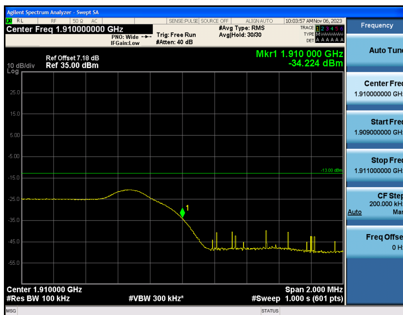
Band2-5MHz-16QAM-19175-1RB#24
