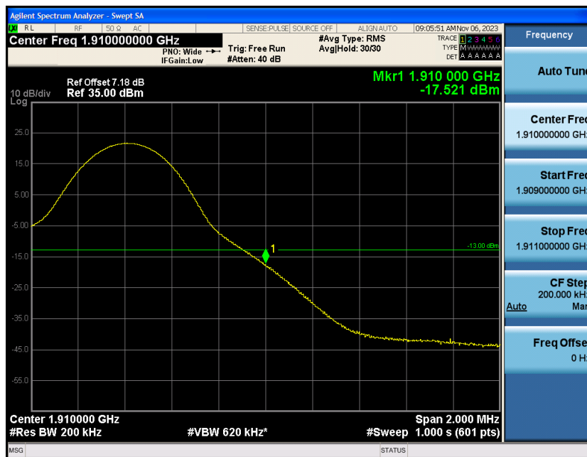
Band2-10MHz-16QAM-19150-50RB#0
