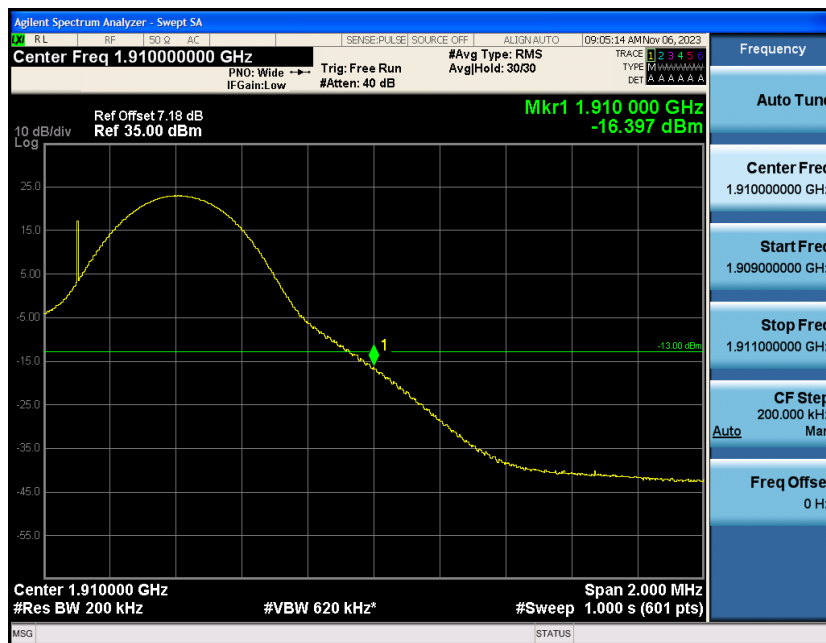
Band2-10MHz-QPSK-19150-50RB#0
