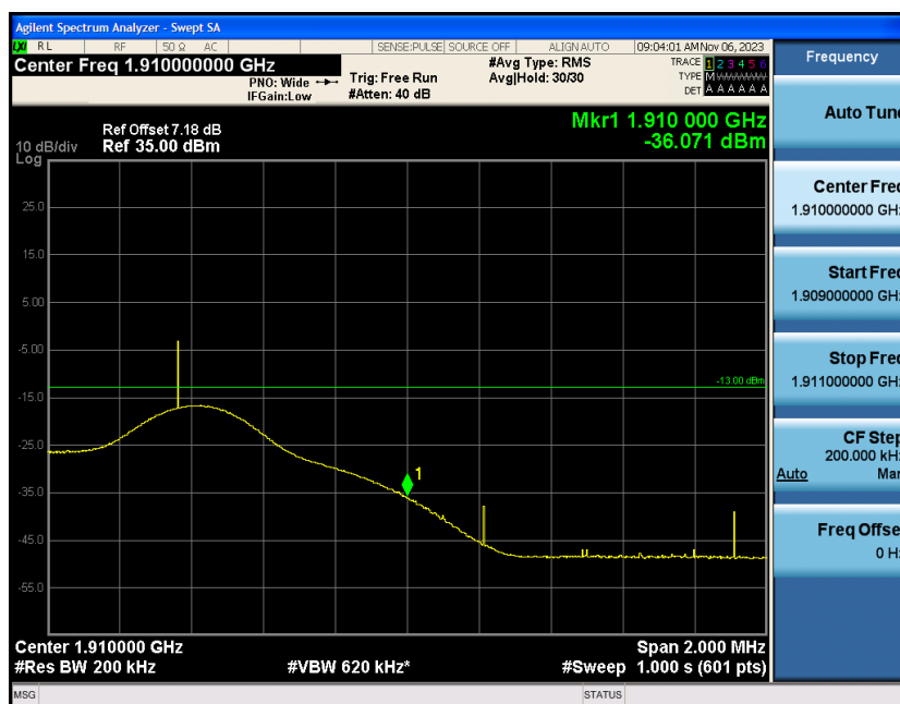
Band2-10MHz-QPSK-19150-1RB#49
