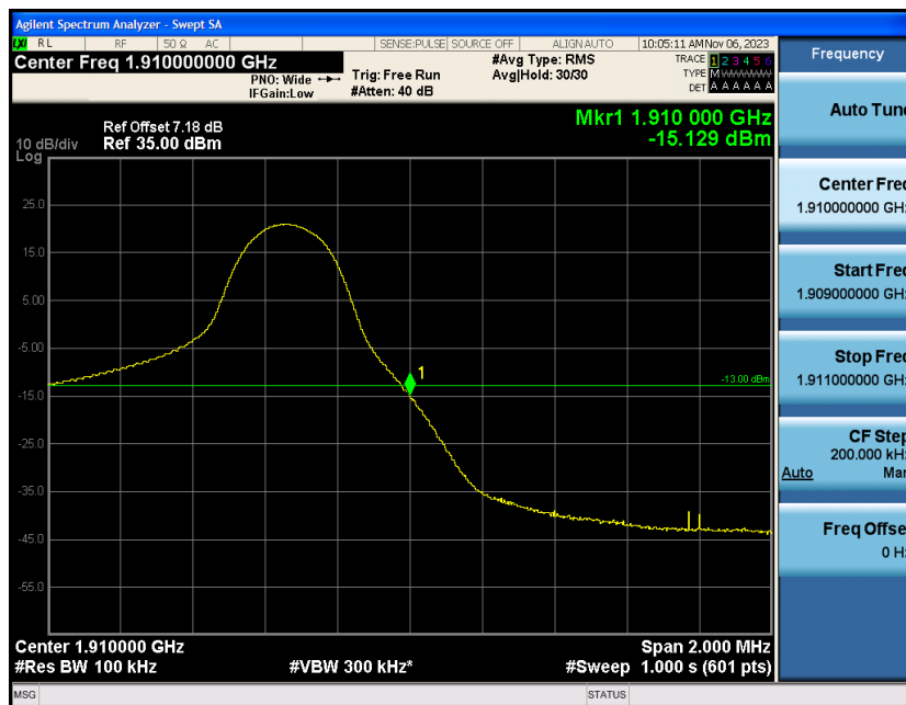
Band2-5MHz-16QAM-19175-25RB#0
