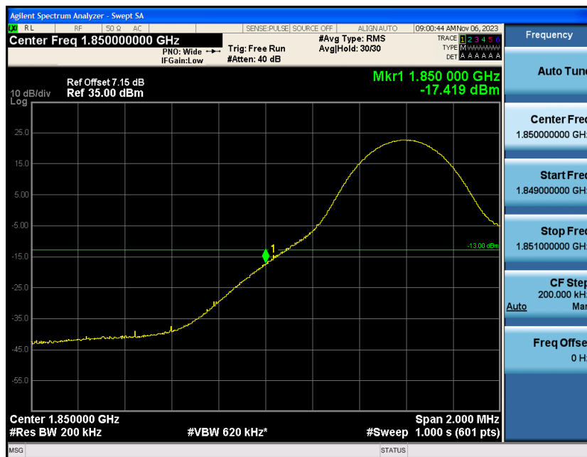
Band2-10MHz-16QAM-18650-1RB#49
