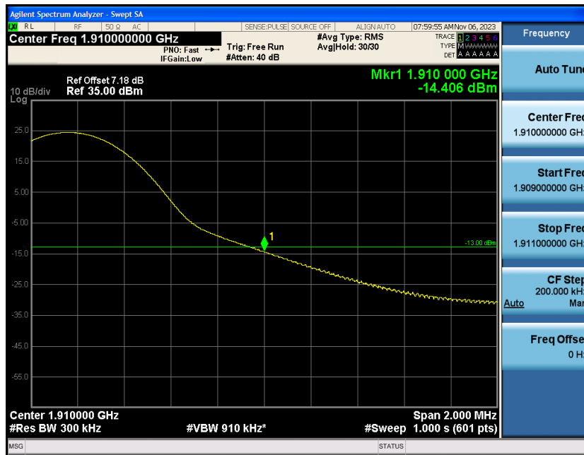
Band2-15MHz-16QAM-19125-75RB#0
