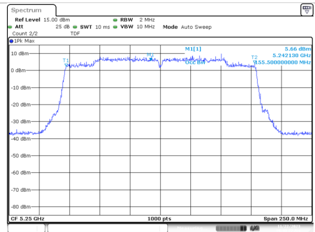
MIMO A-802.11ax/be-160MHz-50-5250-MCS0 99%
