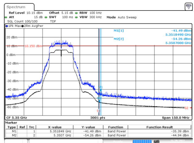
BE-R-HIGH, SISO-A, 802.11ax/be20-MCS0, Ch64
