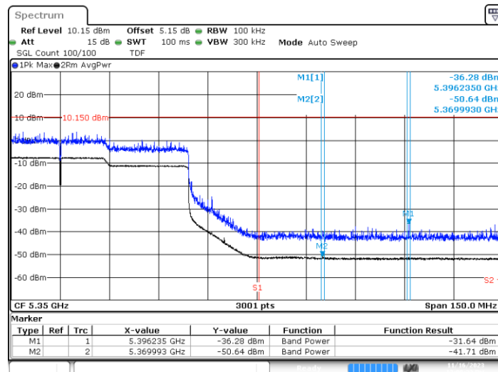
BE-R-HIGH, SISO-B, 802.11ax/be160-MCS0, Ch50
