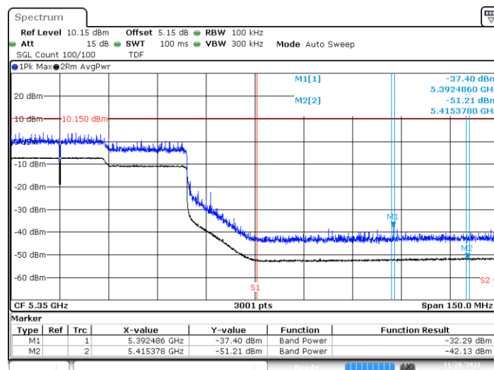
BE-R-HIGH, SISO-A, 802.11ax/be80-MCS0, Ch58
