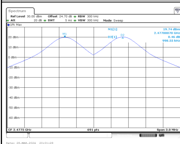
Channel Separation Plot on Channel 75 - 76
