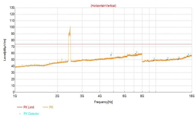
BT_2DH5_2480
