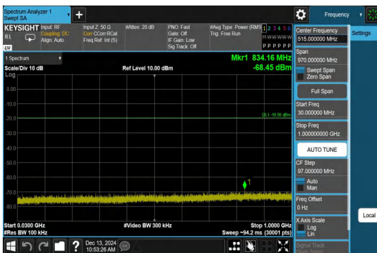
2DH5-Ant1-2441-30~1000-PASS
