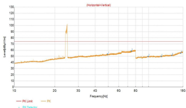
BT_2DH5_2441
