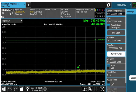
DH5-Ant1-2480-30~1000-PASS
