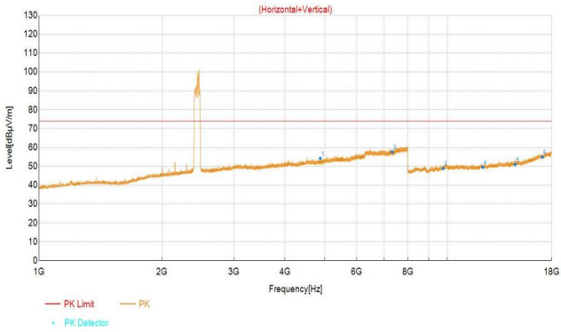
BT_3DH5_2402
