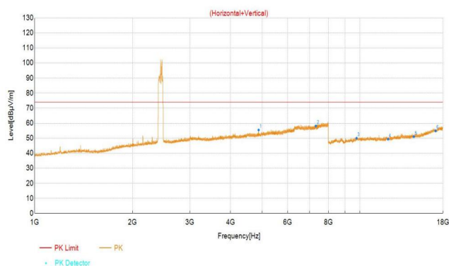
BT_2DH5_2402
