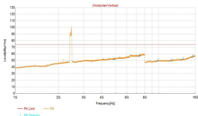
BT_2DH5_2480
