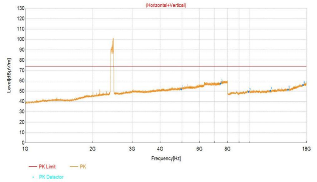
BT_3DH5_2441
