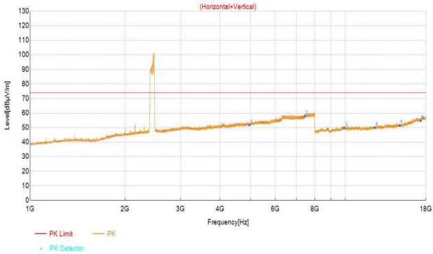
BT_3DH5_2480
