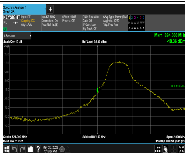
Band26-3MHz-QPSK-26805-1RB#14
