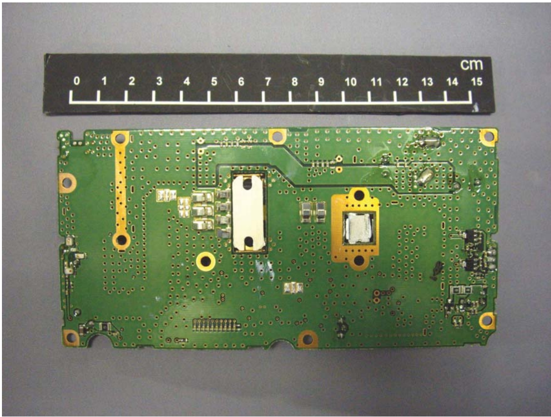
Final A Foil Side View
