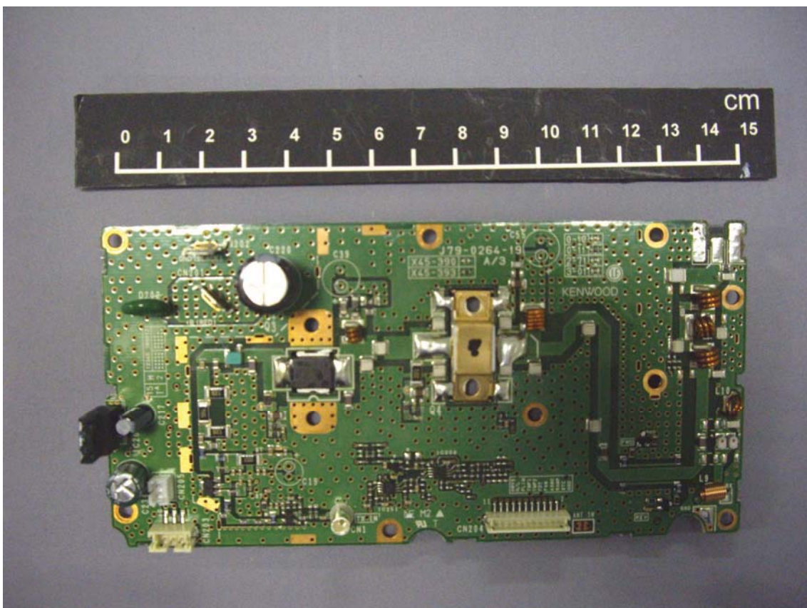
Final A Component Side View
