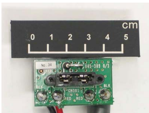
Final B Component Side View
