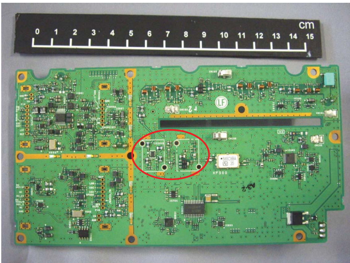
TX-RX Foil Side without Shield View
