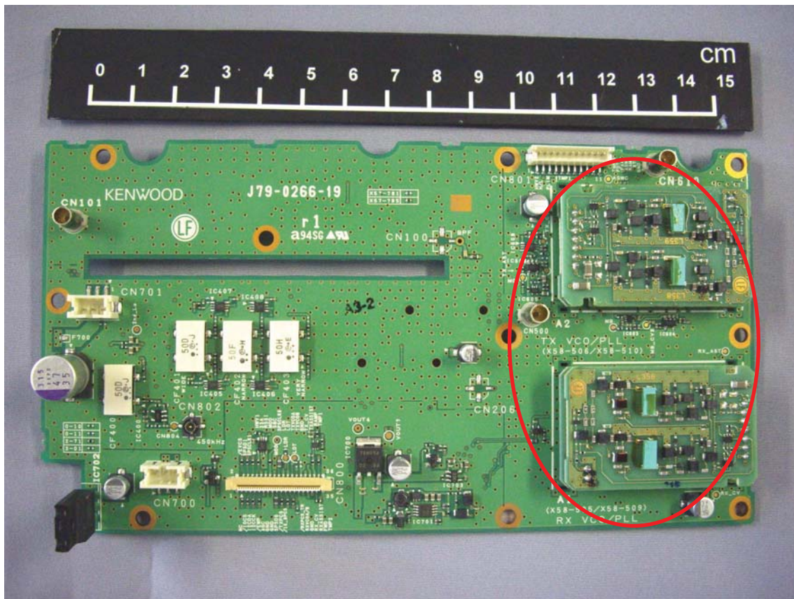
TX-RX Component Side without Shield View
