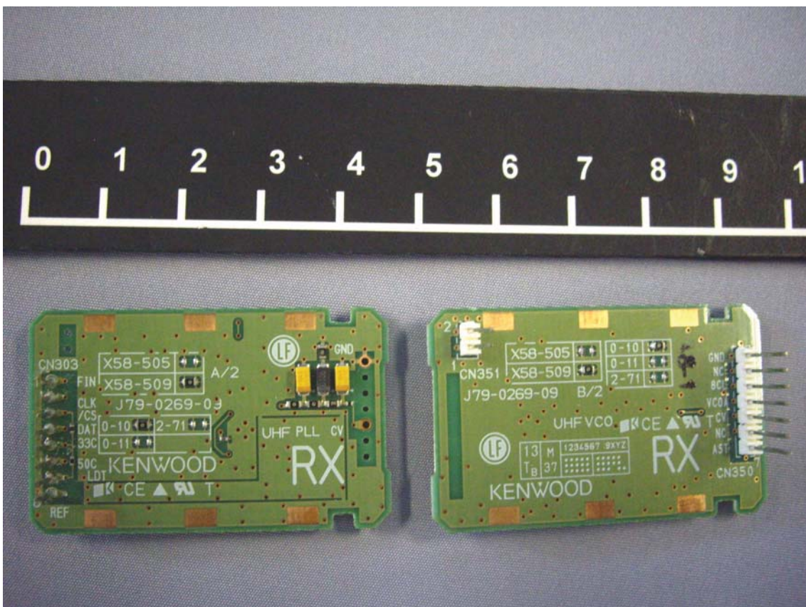
SUB RX VCO/PLL Foil Side View
