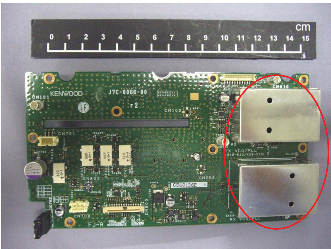
TX-RX Component Side with Shield View
