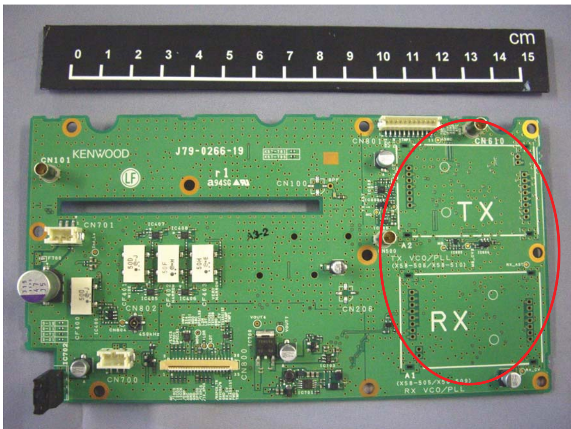
TX-RX Component Side without Shield and SUB Unit (RX/TX) View
