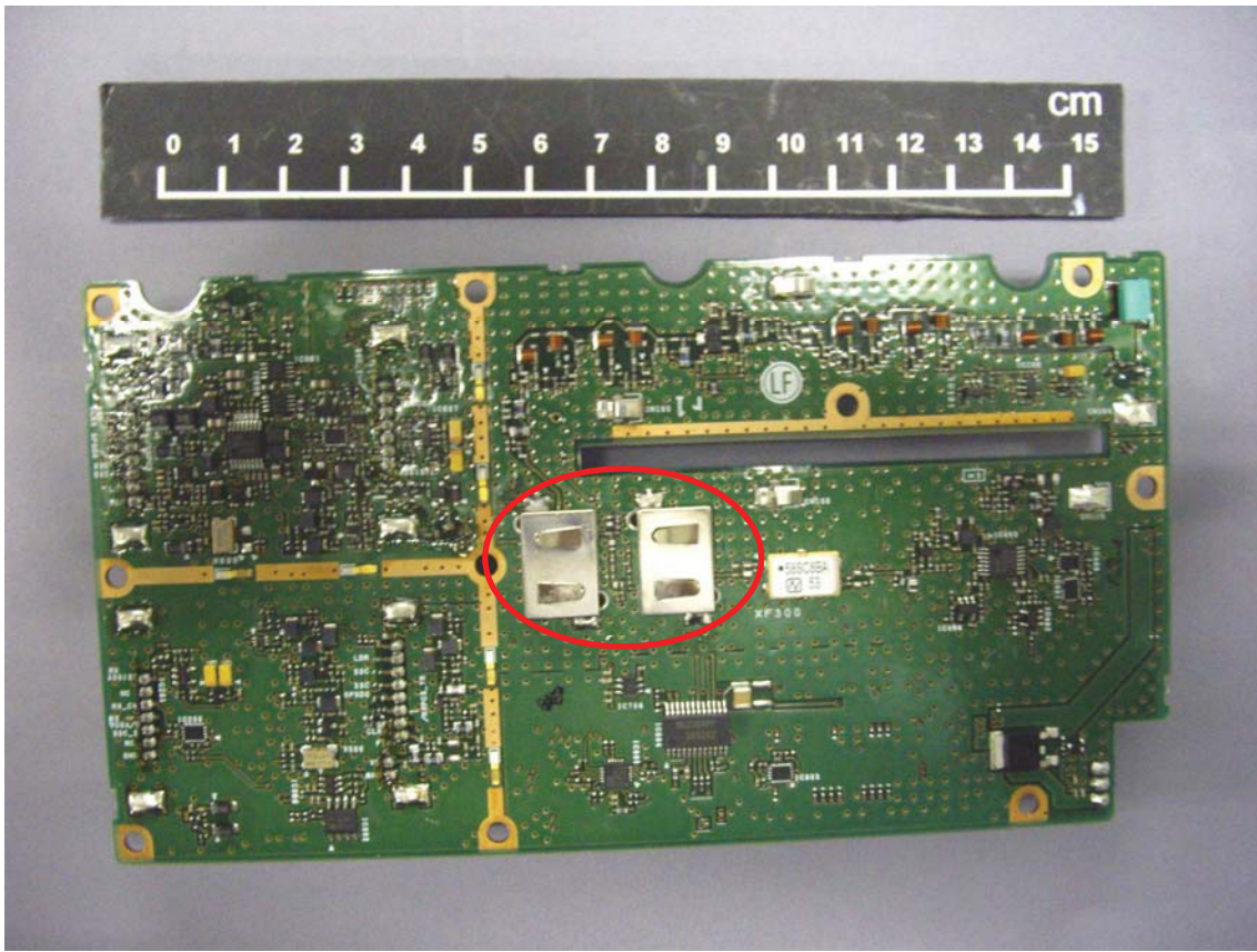
TX-RX Foil Side with Shield View
