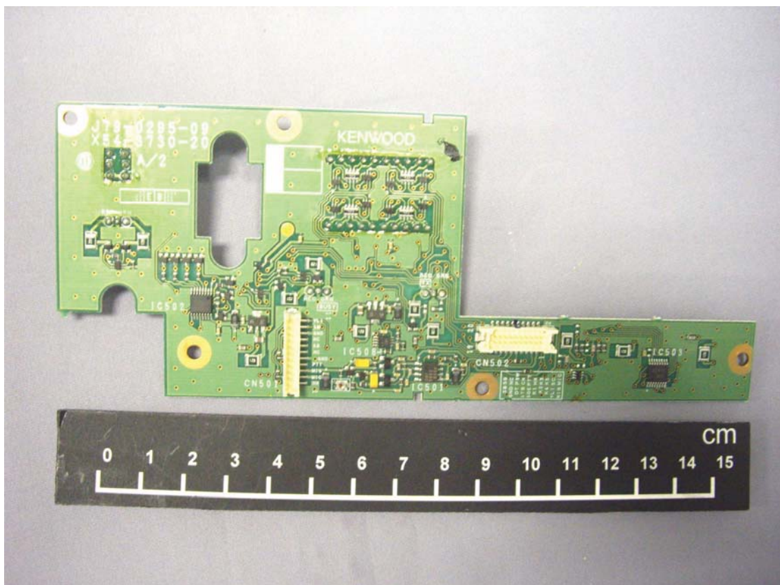
Display A Component Side View
