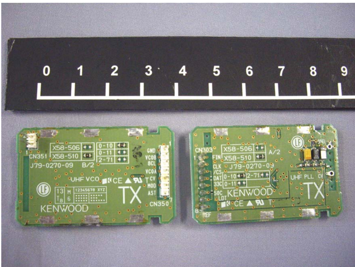
SUB TX VCO/PLL Foil Side View
