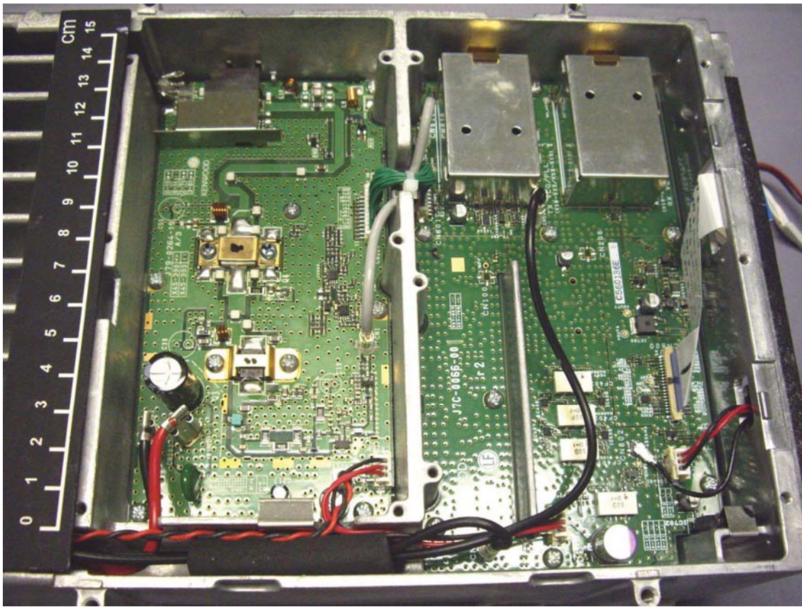
Final A Unit / TX-RX Unit
