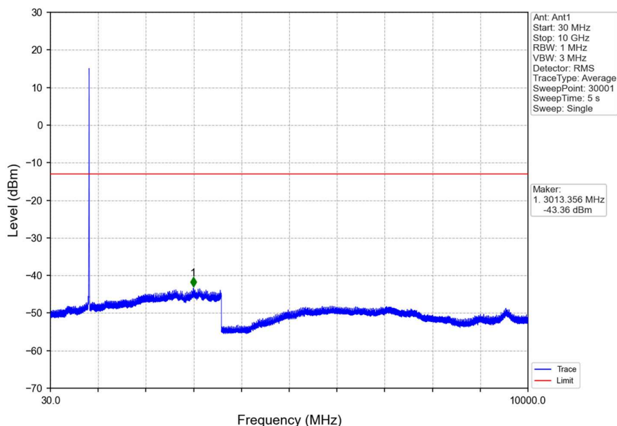
Band5_RMC_MCH_836.6MHz_12.2kbps RMC_NTNV
