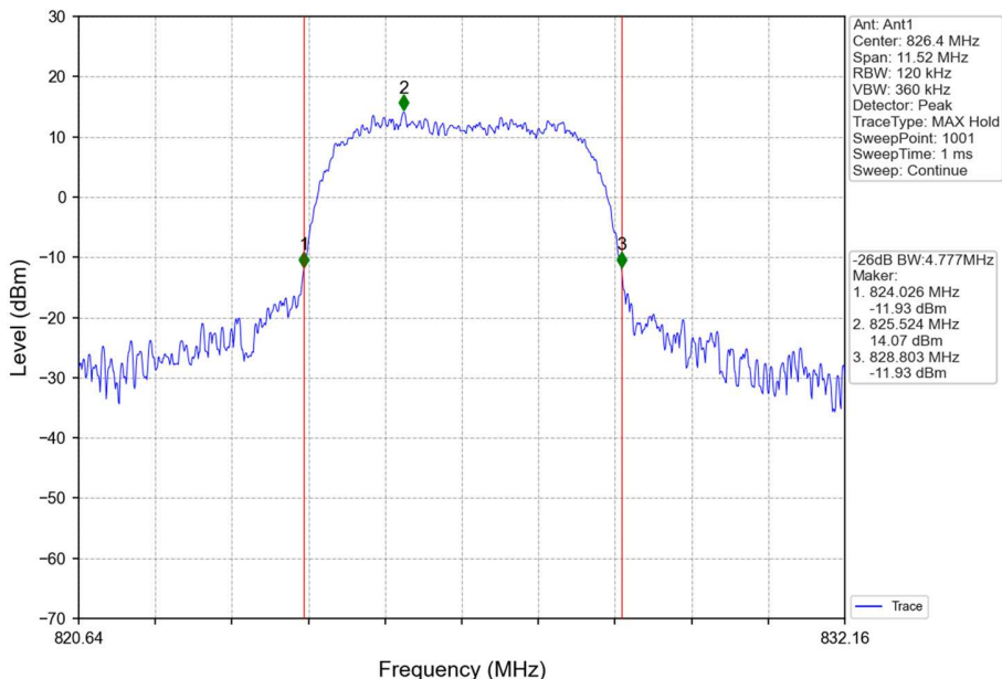
Band5_HSUPA_LCH_826.4MHz_Subtest 1_NTNV
