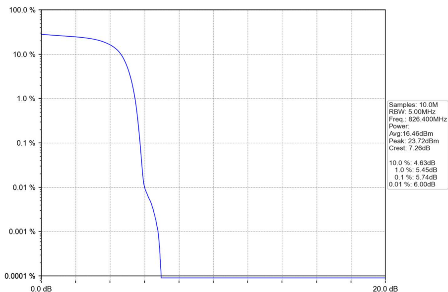
Band5_HSUPA_LCH_826.4MHz_Subtest 1_NTNV
