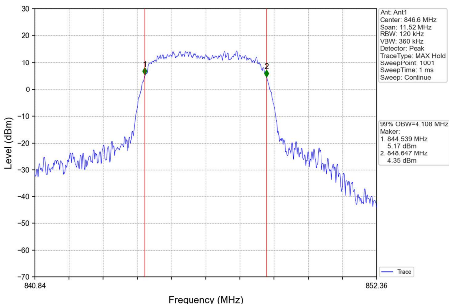
Band5_HSUPA_HCH_846.6MHz_Subtest 1_NTNV
