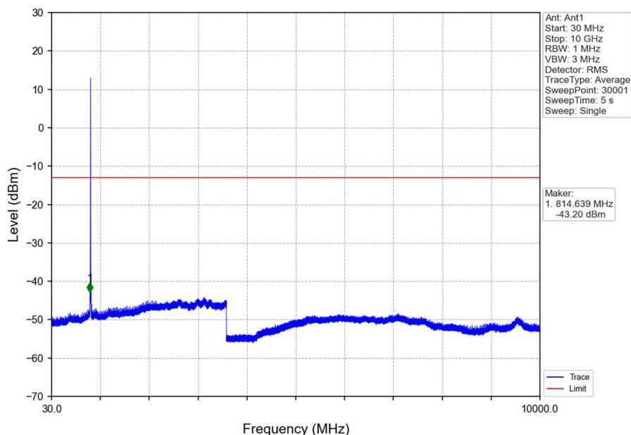
Band5_HSDPA_LCH_826.4MHz_Subtest 1_NTNV
