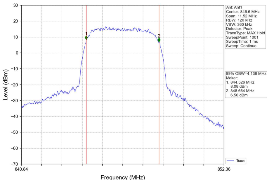
Band5_RMC_HCH_846.6MHz_12.2kbps RMC_NTNV
