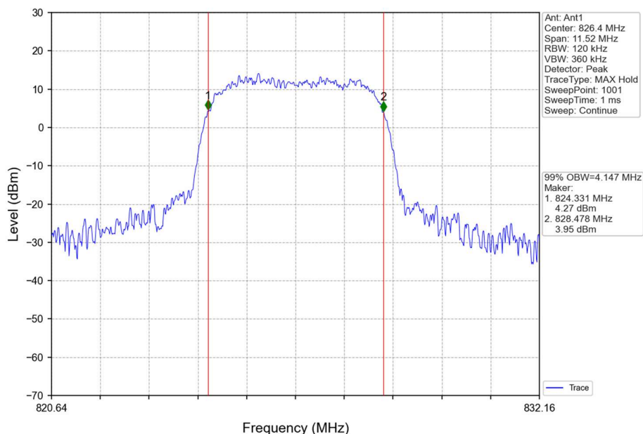
Band5_HSUPA_LCH_826.4MHz_Subtest 1_NTNV
