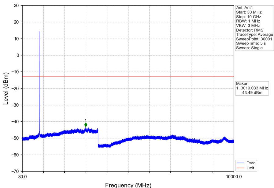
Band5_RMC_LCH_826.4MHz_12.2kbps RMC_NTNV
