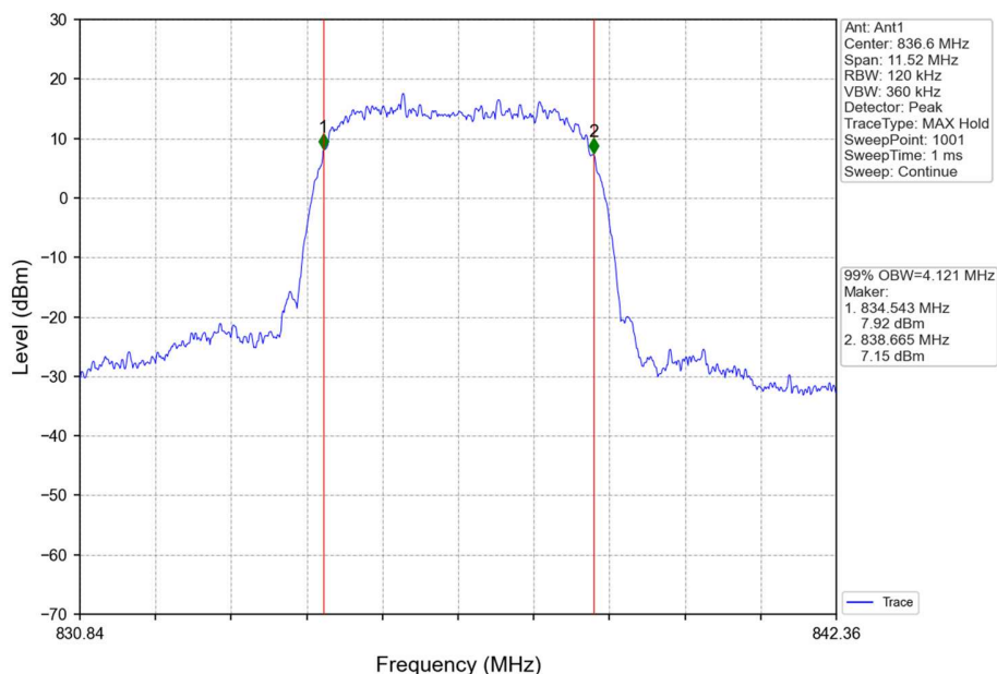
Band5_RMC_MCH_836.6MHz_12.2kbps RMC_NTNV
