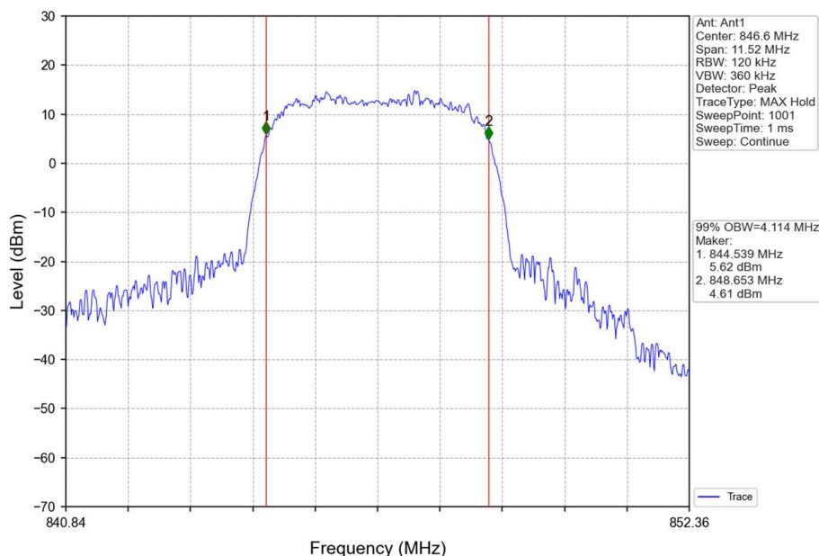
Band5_HSDPA_HCH_846.6MHz_Subtest 1_NTNV
