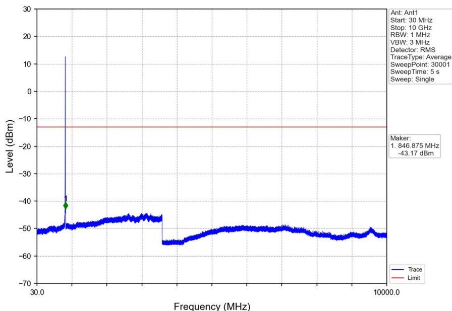
Band5_HSDPA_MCH_836.6MHz_Subtest 1_NTNV
