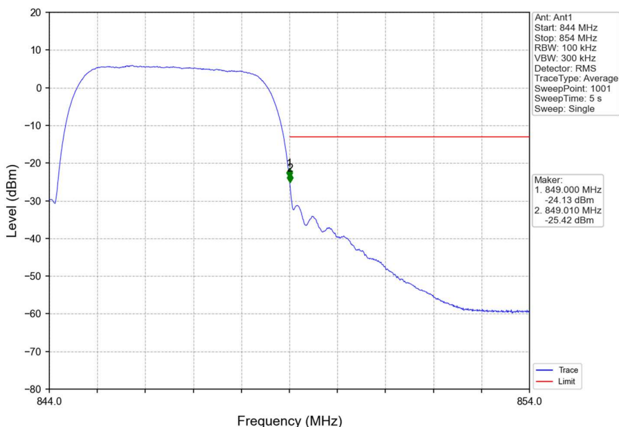
Band5_RMC_HCH_846.6MHz_12.2kbps RMC_NTNV
