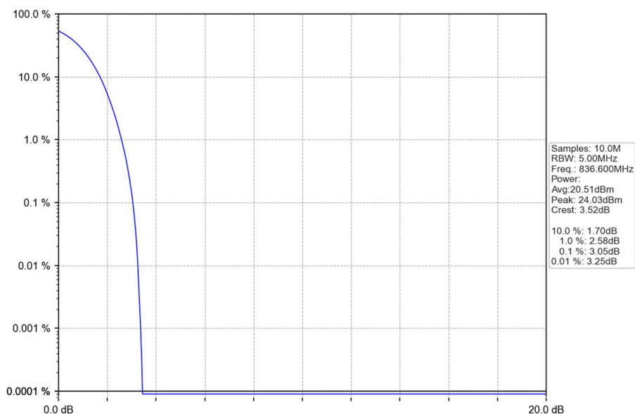
Band5_RMC_MCH_836.6MHz_12.2kbps RMC_NTNV
