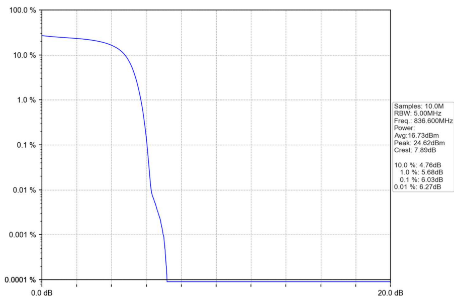
Band5_HSDPA_MCH_836.6MHz_Subtest 1_NTNV
