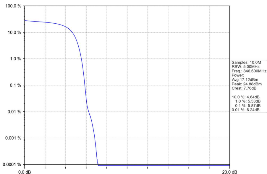
Band5_HSDPA_HCH_846.6MHz_Subtest 1_NTNV
