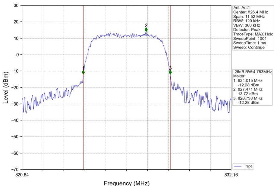
Band5_HSDPA_LCH_826.4MHz_Subtest 1_NTNV
