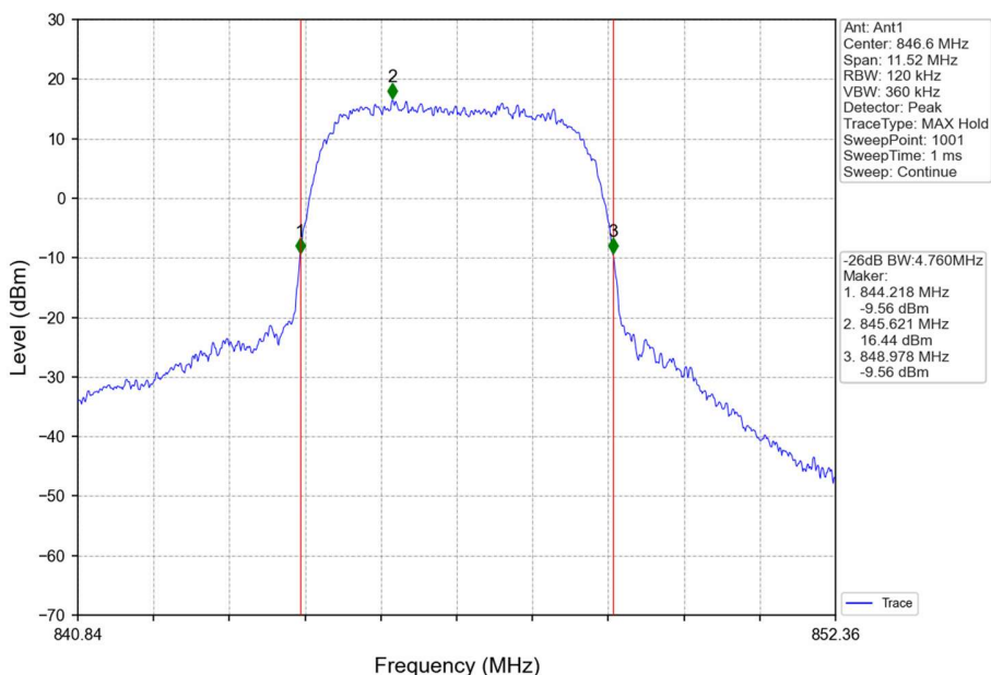
Band5_RMC_HCH_846.6MHz_12.2kbps RMC_NTNV
