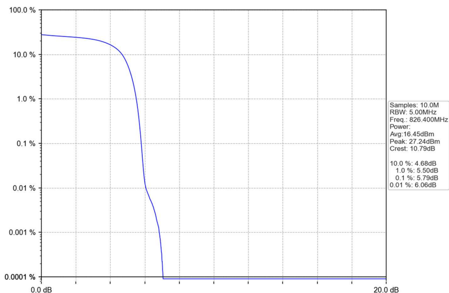
Band5_HSDPA_LCH_826.4MHz_Subtest 1_NTNV
