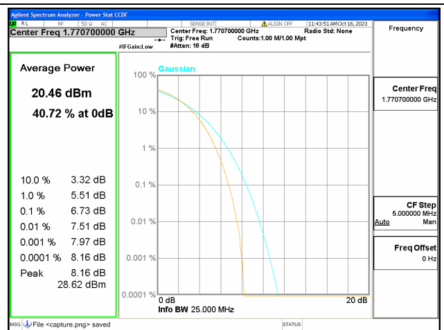
66B / 5+15MHz / High CH / 16QAM
