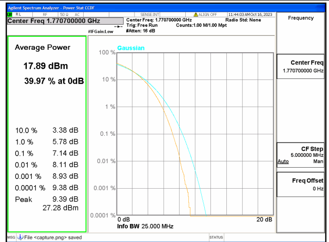
66B / 5+15MHz / High CH / 256QAM
