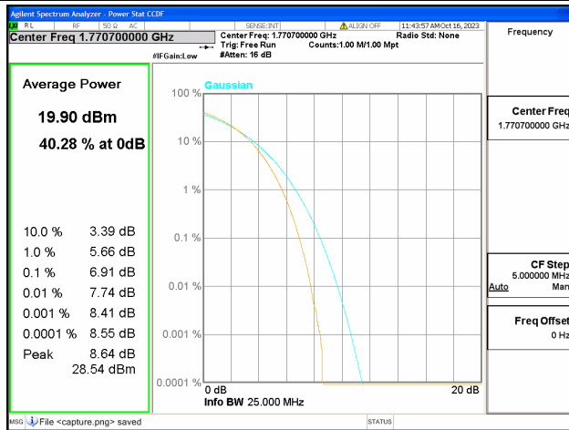
66B / 5+15MHz / High CH / 64QAM
