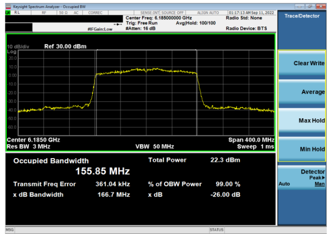
Plot 7-65. 26dB & 99% Bandwidth Plot Antenna WF5t (160MHz 802.11ax (UNII Band 5) – Ch. 47, MCS2)
