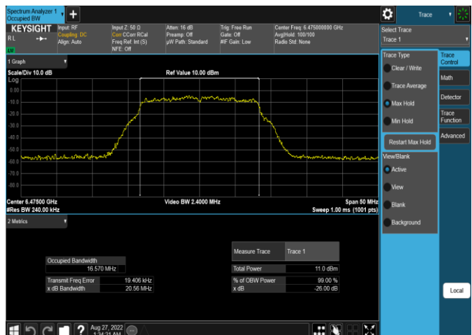
Plot 7-6. 26dB & 99% Bandwidth Plot Antenna WF5t (20MHz 802.11a (UNII Band 6) – Ch. 105, 12Mbps)
