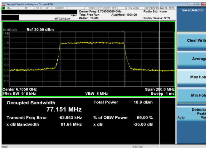
Plot 7-34. 26dB & 99% Bandwidth Plot Antenna WF5t (80MHz 802.11ax (UNII Band 7) – Ch. 151, MCS4)
