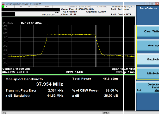
Plot 7-23. 26dB & 99% Bandwidth Plot Antenna WF5t (40MHz 802.11ax (UNII Band 5) – Ch. 43, MCS4)
