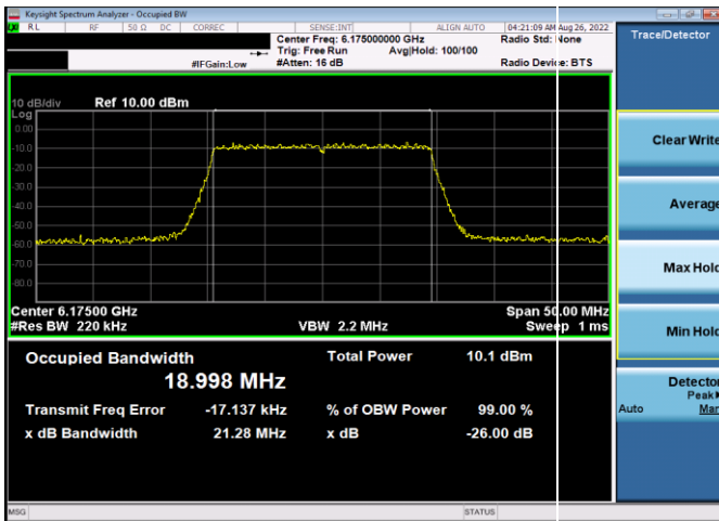
Plot 7-62. 26dB & 99% Bandwidth Plot Antenna WF5t (20MHz 802.11ax (UNII Band 5) – Ch. 45, MCS2)
