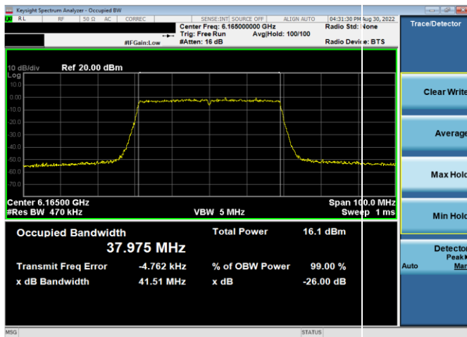
Plot 7-63. 26dB & 99% Bandwidth Plot Antenna WF5t (40MHz 802.11ax (UNII Band 5) – Ch. 43, MCS2)
