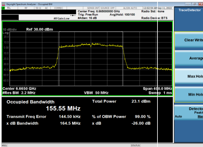
Plot 7-55. 26dB & 99% Bandwidth Plot Antenna WF5t (160MHz 802.11ax (UNII Band 7) – Ch. 143, MCS11)
