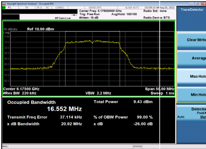
Plot 7-61. 26dB & 99% Bandwidth Plot Antenna WF5t (20MHz 802.11a (UNII Band 5) – Ch. 45, 12Mbps)
