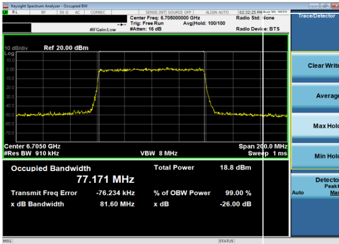
Plot 7-54. 26dB & 99% Bandwidth Plot Antenna WF5t (80MHz 802.11ax (UNII Band 7) – Ch. 151, MCS11)
