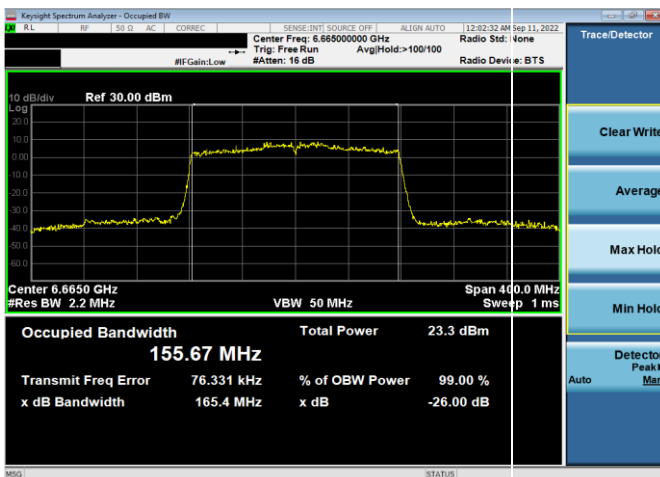
Plot 7-35. 26dB & 99% Bandwidth Plot Antenna WF5t (160MHz 802.11ax (UNII Band 7) – Ch. 143, MCS4)
