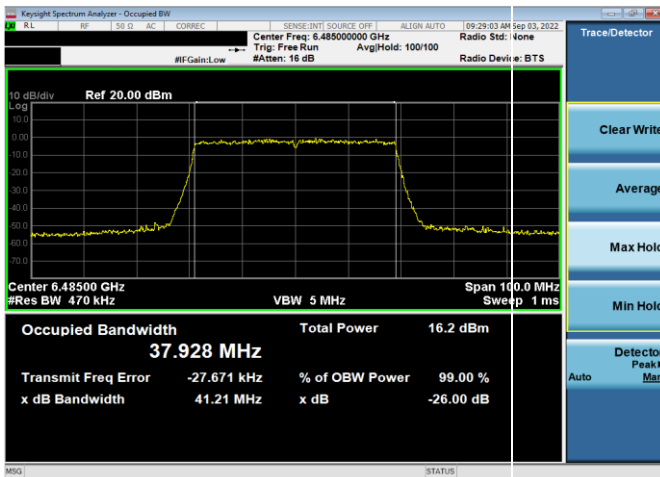
Plot 7-8. 26dB & 99% Bandwidth Plot Antenna WF5t (40MHz 802.11ax (UNII Band 6) – Ch. 107, MCS2)
