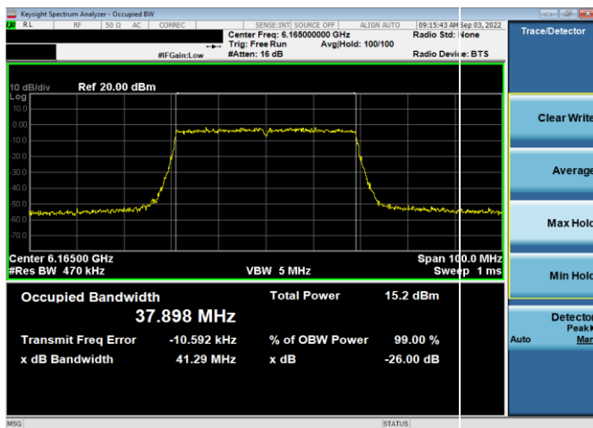
Plot 7-3. 26dB & 99% Bandwidth Plot Antenna WF5t (40MHz 802.11ax (UNII Band 5) – Ch. 43, MCS2)
