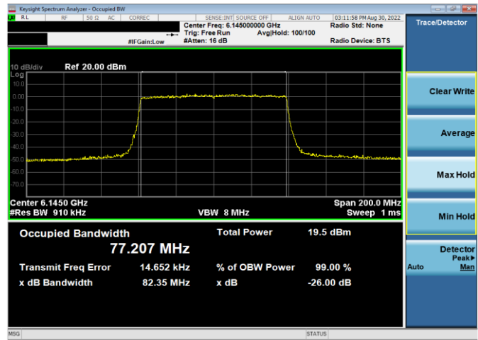
Plot 7-64. 26dB & 99% Bandwidth Plot Antenna WF5t (80MHz 802.11ax (UNII Band 5) – Ch. 39, MCS2)
