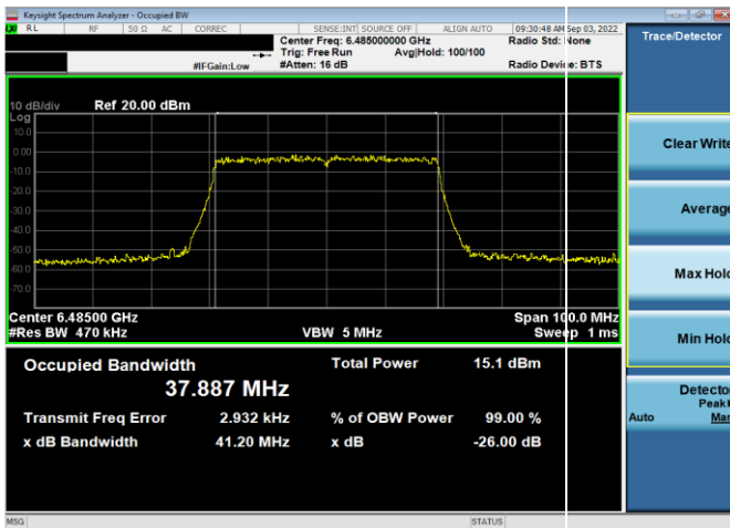
Plot 7-48. 26dB & 99% Bandwidth Plot Antenna WF5t (40MHz 802.11ax (UNII Band 6) – Ch. 107, MCS11)
