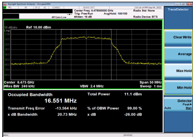
Plot 7-66. 26dB & 99% Bandwidth Plot Antenna WF5t (20MHz 802.11a (UNII Band 6) – Ch. 105, 12Mbps)
