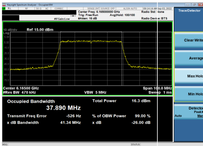
Plot 7-43. 26dB & 99% Bandwidth Plot Antenna WF5t (40MHz 802.11ax (UNII Band 5) – Ch. 43, MCS11)
