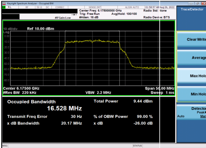
Plot 7-21. 26dB & 99% Bandwidth Plot Antenna WF5t (20MHz 802.11a (UNII Band 5) – Ch. 45, 24Mbps)
