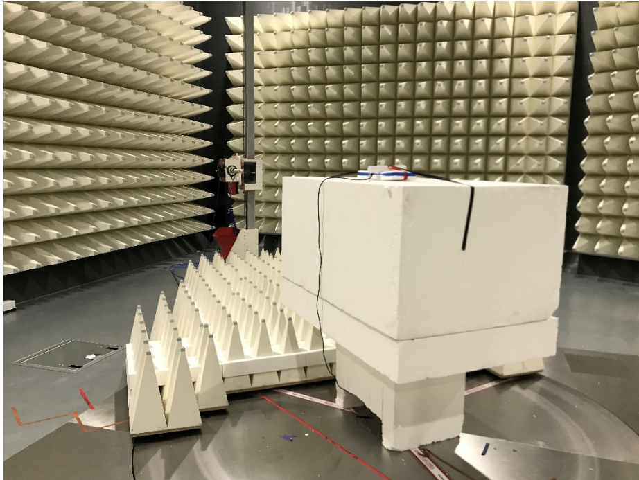
Radiated Emissions 1 GHz – 17 GHz
