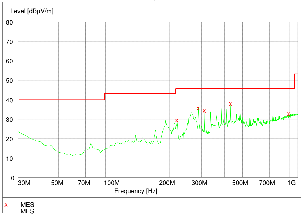
30MHz~1GHz, Horizontal
