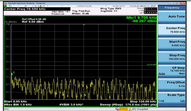
Band41_10MHz_16QAM_40290_1RB#0_0.009~0.15_0.00 9~0.15
