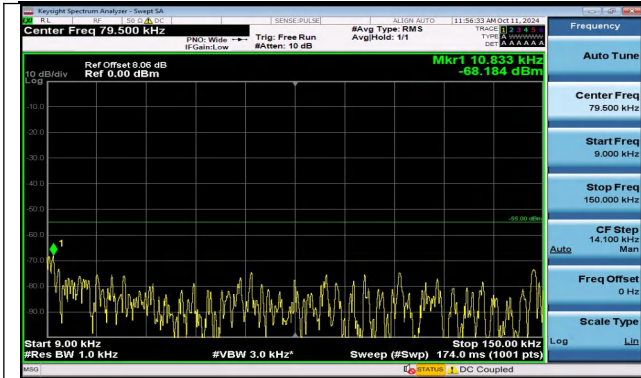
Band41_10MHz_QPSK_41190_1RB#0_0.009~0.15_0.009 ~0.15
