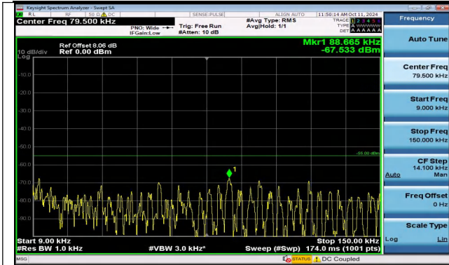
Band41_10MHz_QPSK_40290_1RB#0_0.009~0.15_0.009 ~0.15
