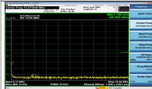
Band41_10MHz_16QAM_41190_1RB#0_0.15~30_0.15~3 0
