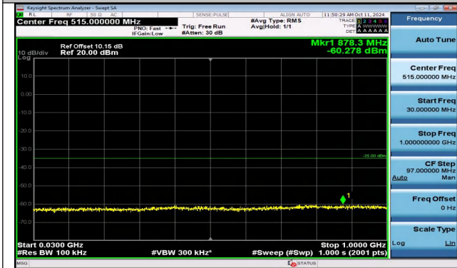
Band41_10MHz_QPSK_40290_1RB#0_30~1000_30~100 0
