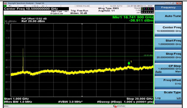
Band41_10MHz_QPSK_41190_1RB#0_1000~20000_100 0~20000
