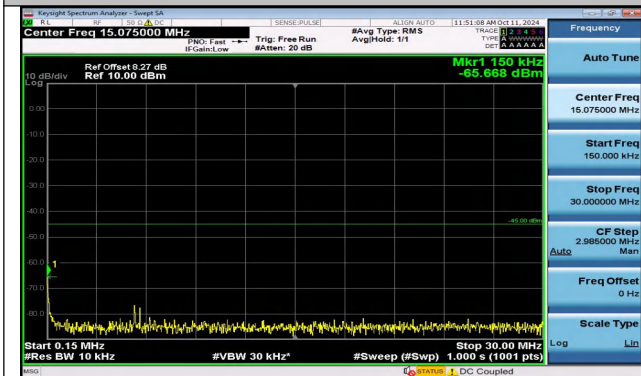
Band41_10MHz_16QAM_40290_1RB#0_0.15~30_0.15~3 0
