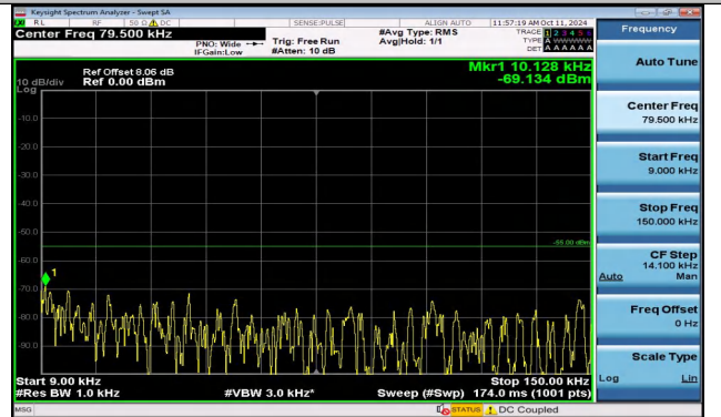
Band41_10MHz_16QAM_41190_1RB#0_0.009~0.15_0.00 9~0.15
