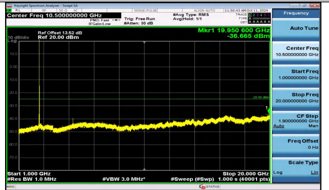
Band41_10MHz_QPSK_40290_1RB#0_1000~20000_100 0~20000
