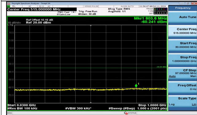
Band41_10MHz_QPSK_41190_1RB#0_30~1000_30~100 0
