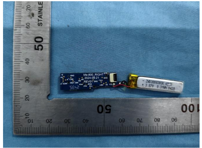
PCB and Battery Front
