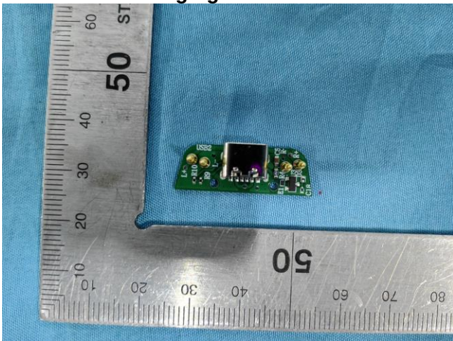
Charging dock Front
