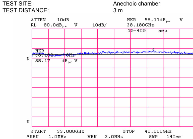
Plot 8.2.12 Radiated emission measurements 33000 -40000MHz, horizontal & vertical antenna polarization
