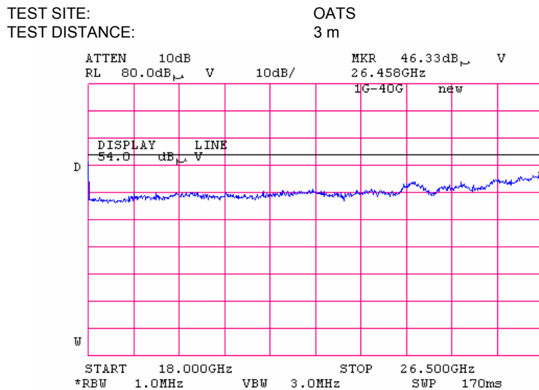
Plot 8.2.22 Radiated emission measurements 18000 -26500MHz, horizontal & vertical antenna polarization
