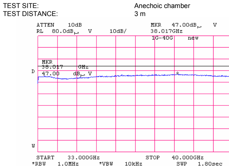
Plot 8.2.13 Radiated emission measurements 33000 -40000MHz, horizontal & vertical antenna polarization
