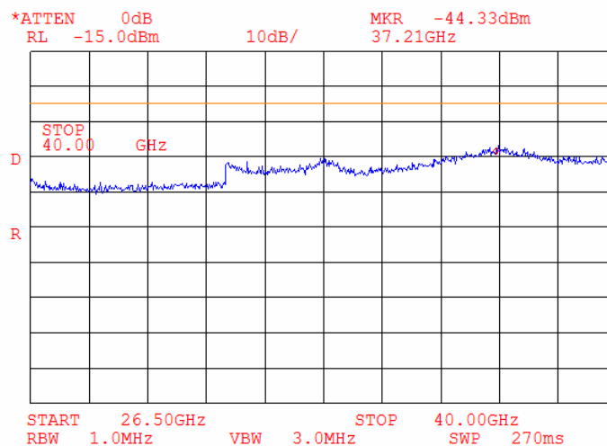
Plot 7.4.29 Spurious emission measurements in 26500 - 40000 MHz range at mid carrier frequency
