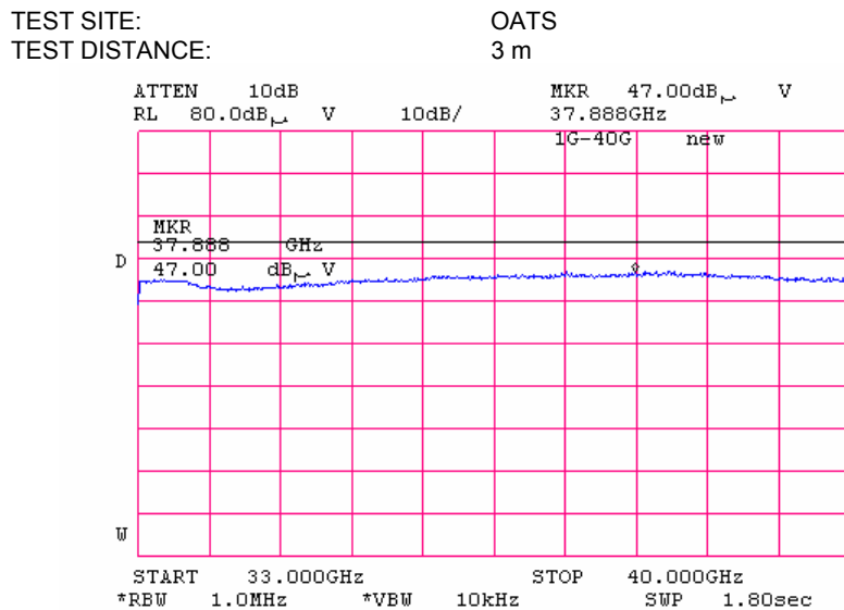
Plot 8.2.25 Radiated emission measurements 33000 -40000MHz, horizontal & vertical antenna polarization
