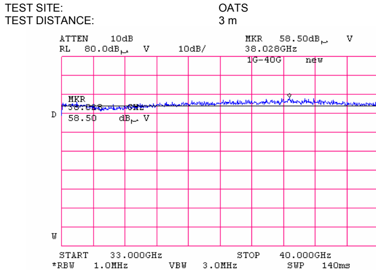
Plot 8.2.24 Radiated emission measurements 33000 -40000MHz, horizontal & vertical antenna polarization
