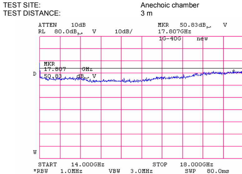
Plot 8.2.21 Radiated emission measurements 14000 -1800MHz, horizontal & vertical antenna polarization
