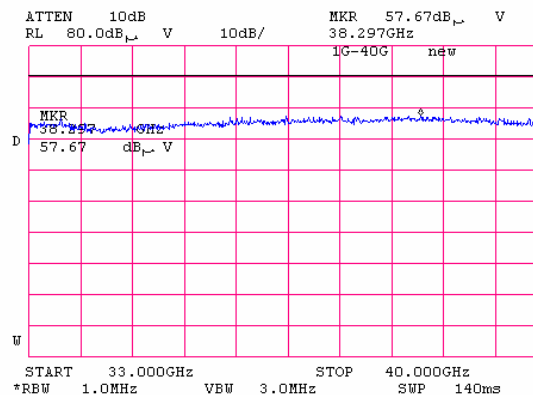
Plot 7.5.81 Radiated emission measurements in 33000 – 40000 MHz range
