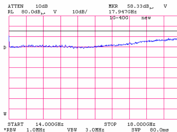
Plot 7.5.26 Radiated emission measurements in 14000 – 18000 MHz range
