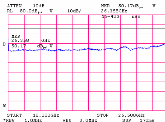
Plot 7.5.30 Radiated emission measurements in 18000 – 26500 MHz range
