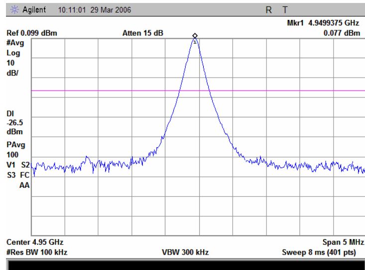
Plot 7.2.1 Unmodulated signal for reference level
