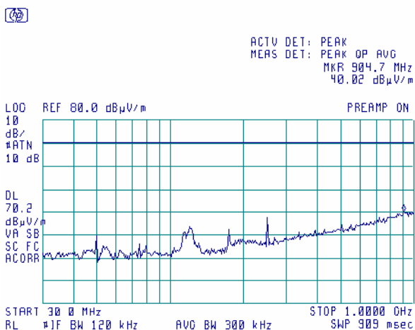
Plot 7.5.53 Radiated emission measurements in 30 - 1000 MHz range
