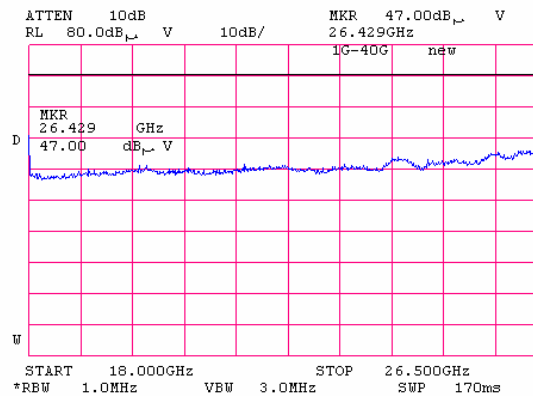
Plot 7.5.75 Radiated emission measurements in 18000 – 26500 MHz range
