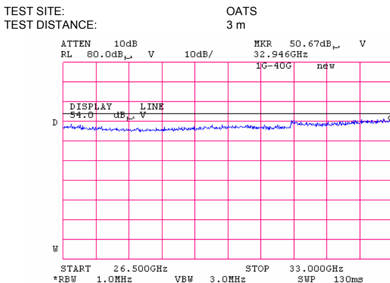
Plot 8.2.23 Radiated emission measurements 26500 -33000MHz, horizontal & vertical antenna polarization
