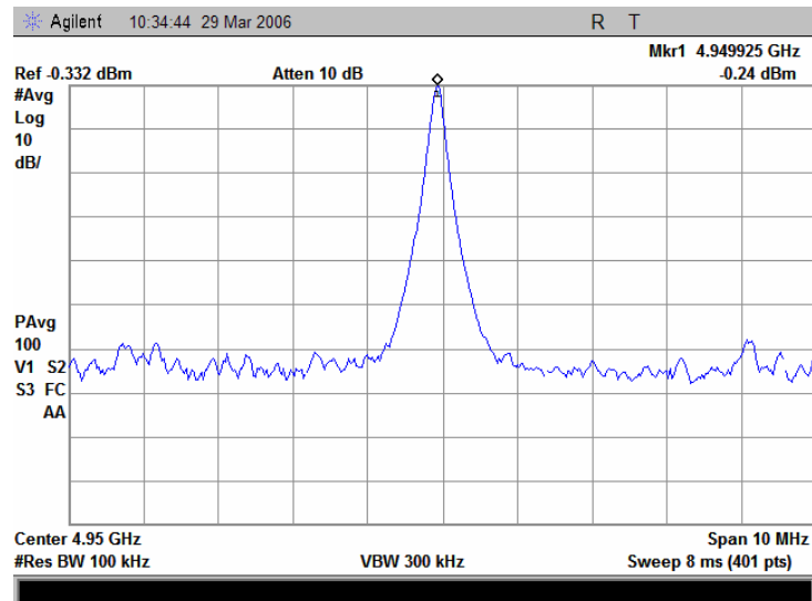
Plot 7.2.14 Unmodulated signal for reference level
