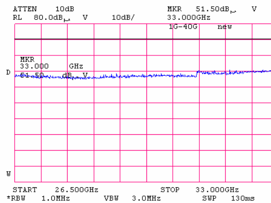
Plot 7.5.77 Radiated emission measurements in 26500 – 33000 MHz range
