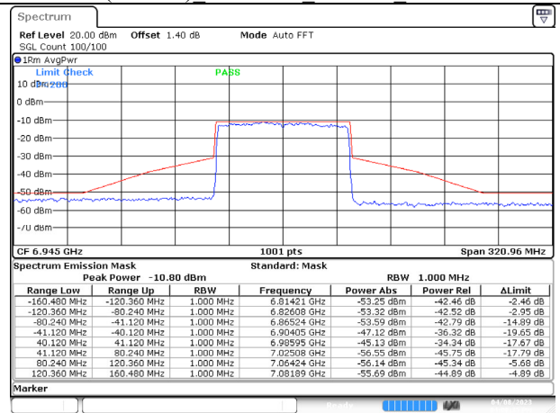
802.11ax (80MHz) 6945MHz Chain B NSS-1
