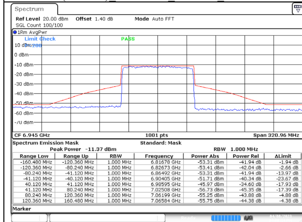
802.11ax (80MHz) 6945MHz Chain A NSS-1
