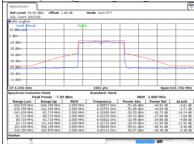
802.11ax (160MHz) 6345MHz Chain A NSS-1
