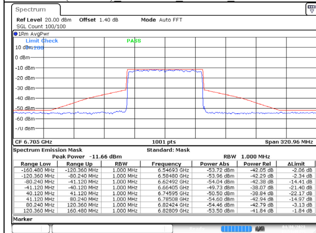
802.11ax (80MHz) 6705MHz Chain A NSS-1
