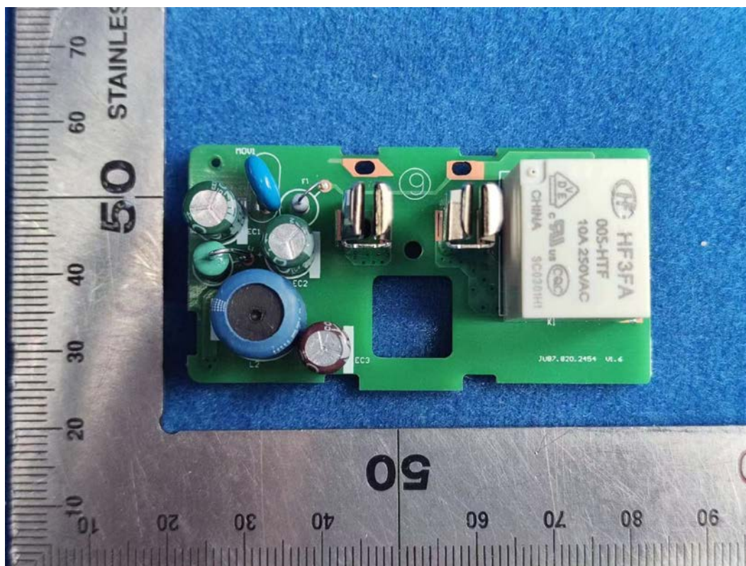
FIGURE 4 SMART PLUG (M/N: CPLGSTDBLW1) MAIN BOARD FRONT
