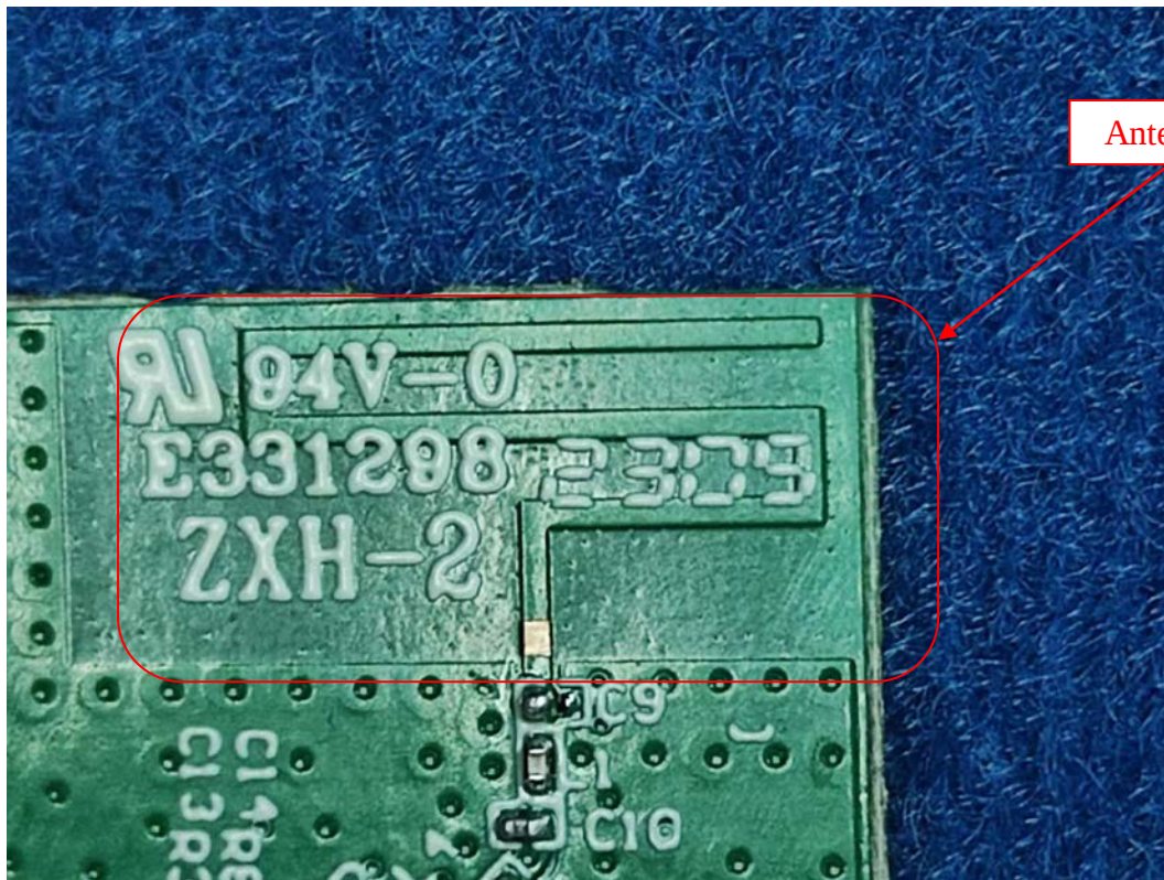
FIGURE 9 SMART PLUG (M/N: CPLGSTDBLW1) ANTENNA
