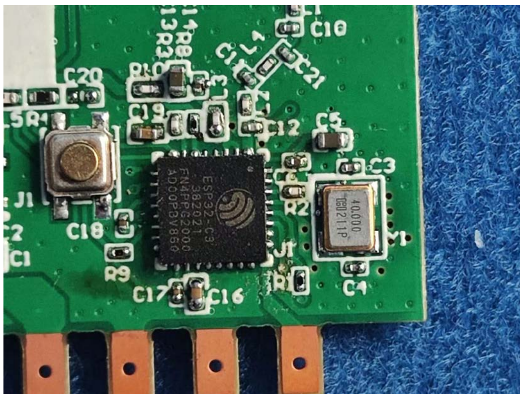
FIGURE 8 SMART PLUG (M/N: CPLGSTDBLW1) CHIP&CRYSTAL ON RFBOARD
