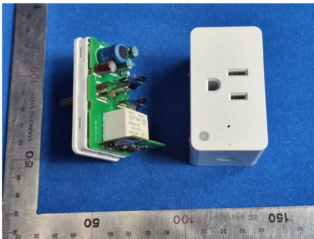
FIGURE 3 SMART PLUG (M/N: CPLGSTDBLW1) REMOVE COVER
