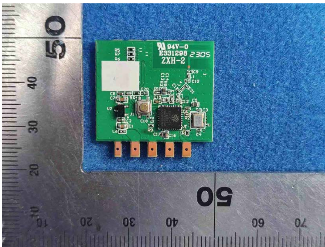
FIGURE 6 SMART PLUG (M/N: CPLGSTDBLW1) RF BORAD FRONT
