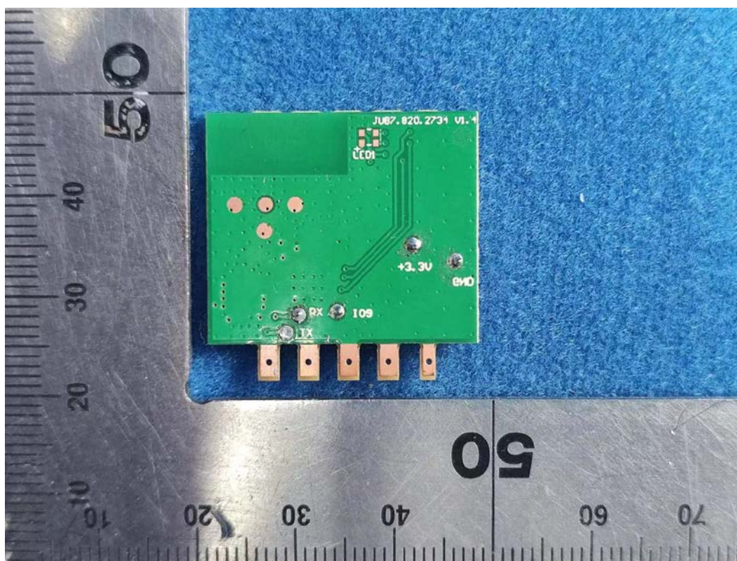
FIGURE 7 SMART PLUG (M/N: CPLGSTDBLW1) RF BOARD BACK
