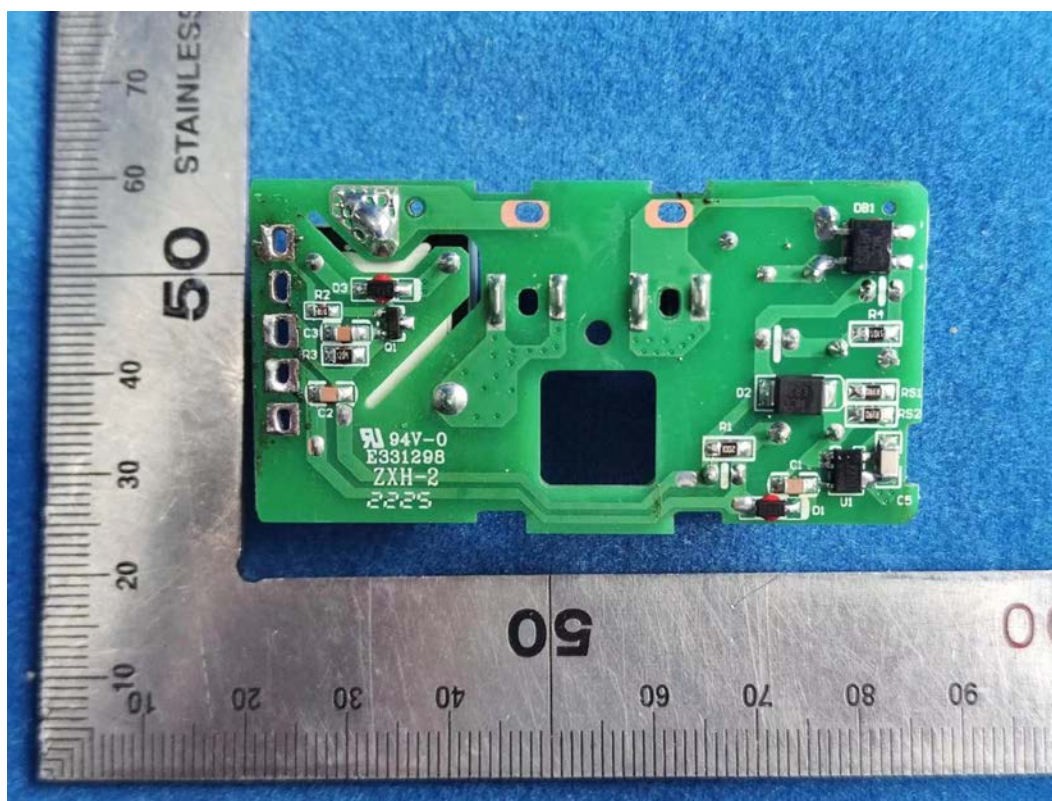
FIGURE 5 SMART PLUG (M/N: CPLGSTDBLW1) MAIN BORAD BACK
