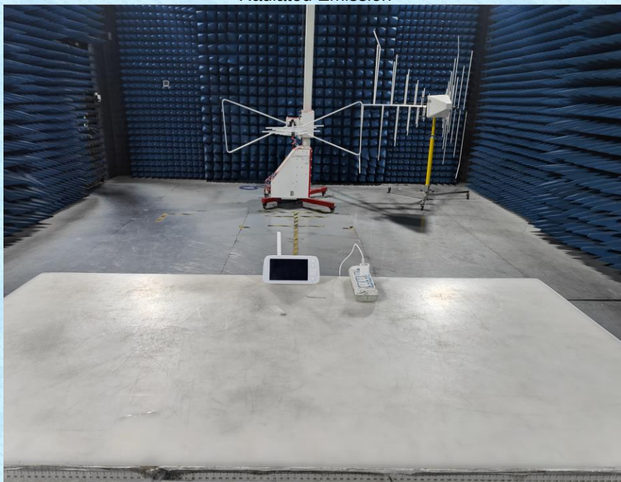
Radiated Emission
