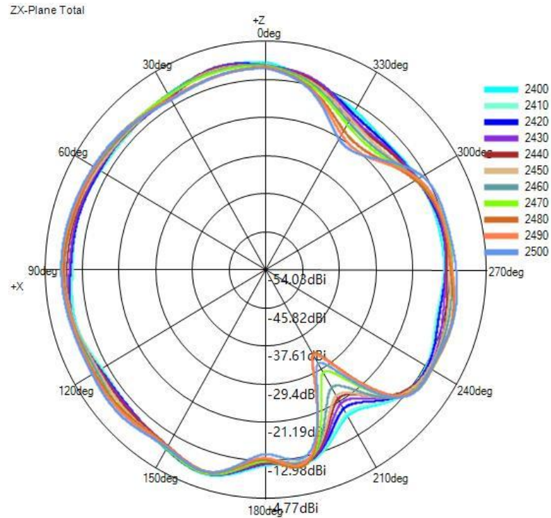
(1) X-Z Plane(unit:dBi):
