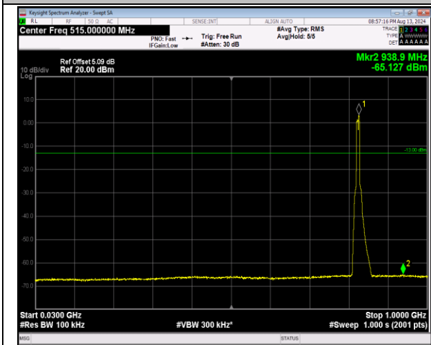
5-5-5MHz-3MHz-16QAM-16QAM-20425-20464-25RB#0-15RB#0-30~1000MHz-PASS
