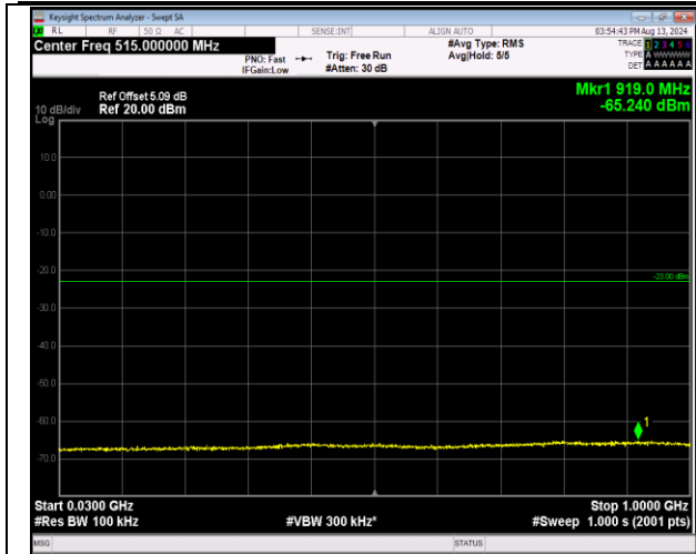
2-2-20MHz-20MHz-16QAM-16QAM-18902-19100-1RB#9 9-ORB#0-30~1000MHz-PASS
