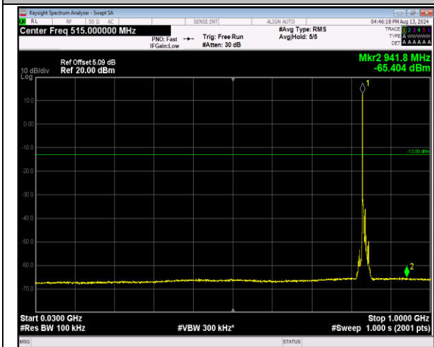
5-5-3MHz-5MHz-16QAM-16QAM-20501-20540-1RB#0-0-1 RB#24-30~1000MHz-PASS
