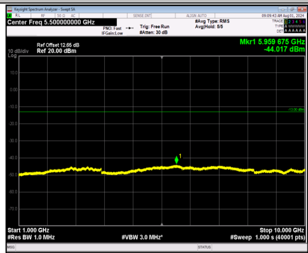
5-5-3MHz-5MHz-64QAM-64QAM-20416-20455-1RB#14-0R B#0-1000~10000MHz-PASS
