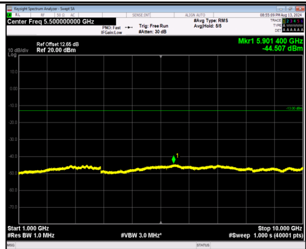
5-5-5MHz-3MHz-16QAM-16QAM-20425-20464-1RB#24-0RB#0-1000~10000MHz-PASS
