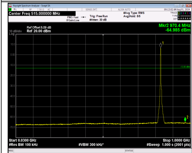
5-5-3MHz-5MHz-64QAM-64QAM-20501-20540-15RB#0-0 25RB#0-30~1000MHz-PASS
