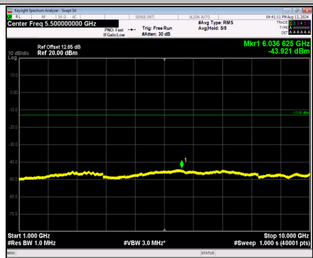
5-5-3MHz-5MHz-QPSK-QPSK-20416-20455-1RB#0-1RB#2 4-1000~10000MHz-PASS
