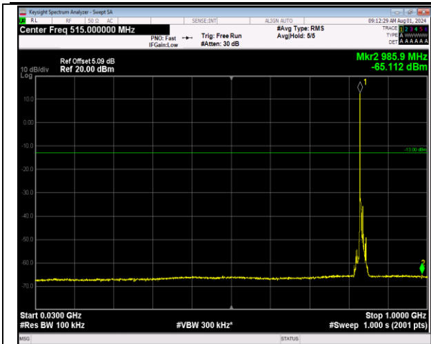
5-5-3MHz-5MHz-64QAM-64QAM-20501-20540-1RB#0-1 RB#24-30~1000MHz-PASS
