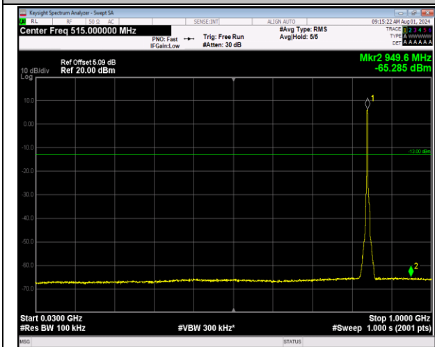
5-5-3MHz-5MHz-64QAM-64QAM-20586-20625-15RB#0-0- 25RB#0-30~1000MHz-PASS
