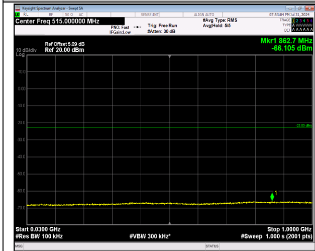
2-2-20MHz-20MHz-64QAM-64QAM-18902-19100-1RB#0 -ORB#0-30~1000MHz-PASS
