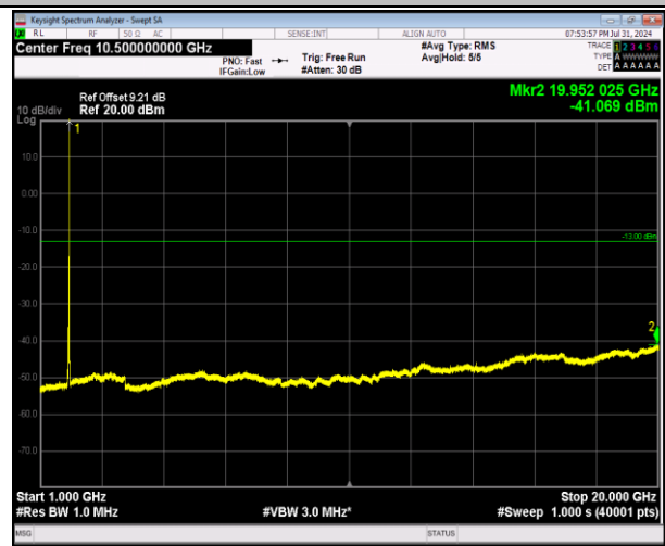
2-2-20MHz-20MHz-64QAM-64QAM-18902-19100-1RB#99- 0RB#0-1000~20000MHz-PASS
