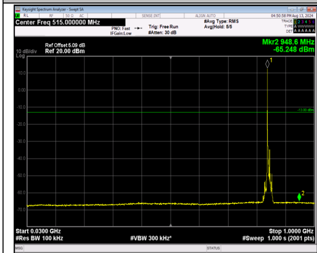
5-5-3MHz-5MHz-16QAM-16QAM-20586-20625-1RB#0-0-1 RB#24-30~1000MHz-PASS
