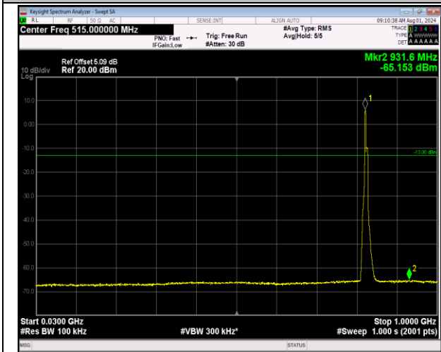
5-5-3MHz-5MHz-64QAM-64QAM-20416-20455-15RB#0-0- 25RB#0-30~1000MHz-PASS
