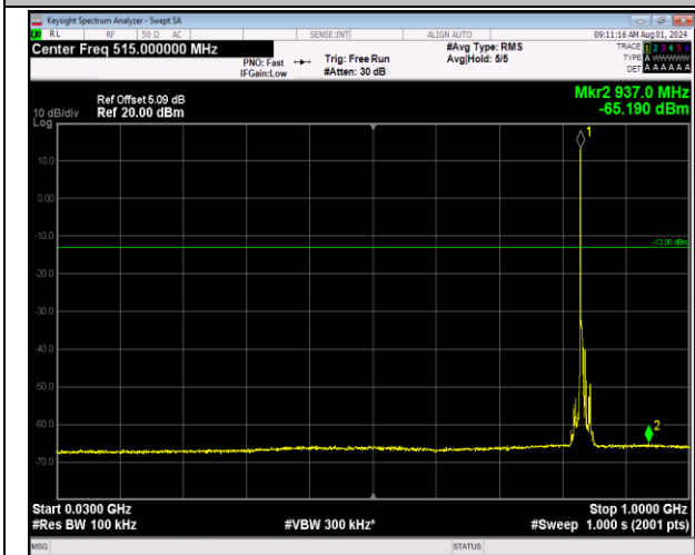
5-5-3MHz-5MHz-64QAM-64QAM-20501-20540-1RB#0-0RB#0-30~1000MHz-PASS
