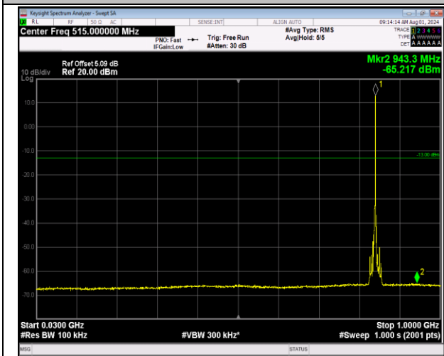
5-5-3MHz-5MHz-64QAM-64QAM-20586-20625-1RB#14- 0RB#0-30~1000MHz-PASS
