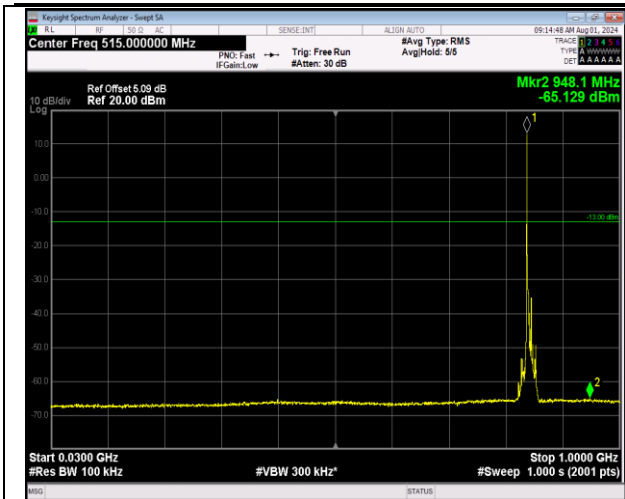
5-5-3MHz-5MHz-64QAM-64QAM-20586-20625-1RB#0-1 RB#24-30~1000MHz-PASS
