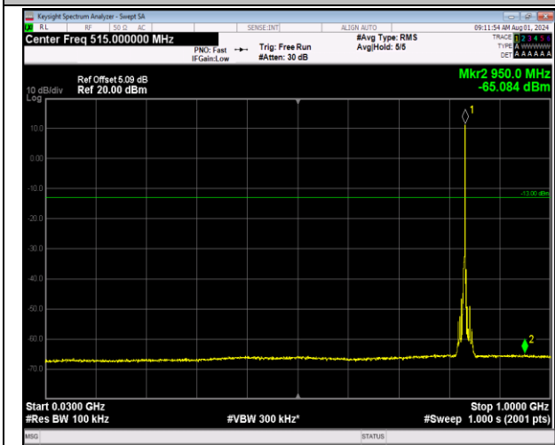
5-5-3MHz-5MHz-64QAM-64QAM-20501-20540-1RB#14- 0RB#0-30~1000MHz-PASS
