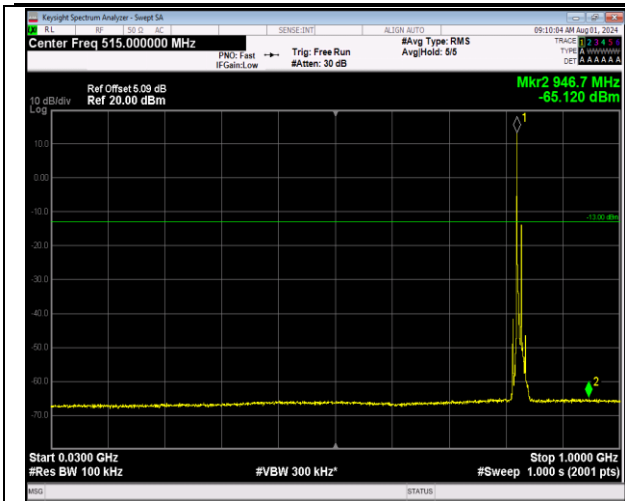
5-5-3MHz-5MHz-64QAM-64QAM-20416-20455-1RB#0-1 RB#24-30~1000MHz-PASS
