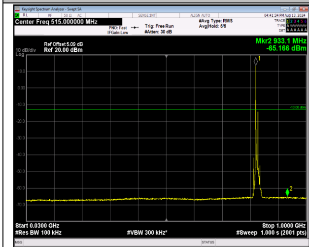
5-5-3MHz-5MHz-16QAM-16QAM-20416-20455-1RB#0-0-1 RB#24-30~1000MHz-PASS
