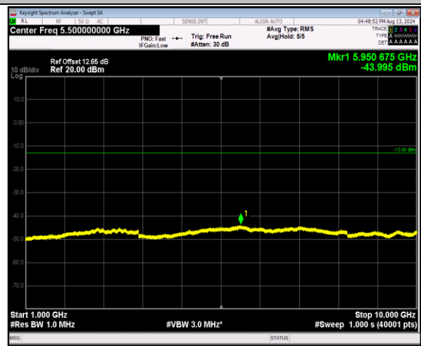
5-5-3MHz-5MHz-16QAM-16QAM-20586-20625-1RB#0-0RB #0-1000~10000MHz-PASS
