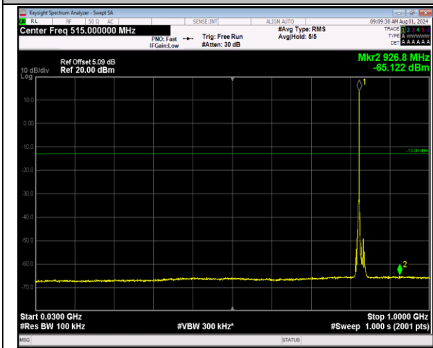
5-5-3MHz-5MHz-64QAM-64QAM-20416-20455-1RB#14- 0RB#0-30~1000MHz-PASS
