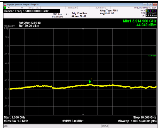
5-5-3MHz-5MHz-64QAM-64QAM-20501-20540-1RB#0-1RB #24-1000~10000MHz-PASS
