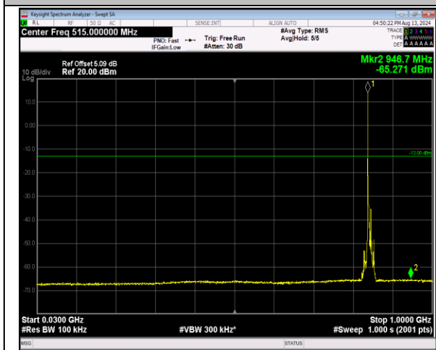
5-5-3MHz-5MHz-QPSK-QPSK-20586-20625-1RB#0-1RB #24-30~1000MHz-PASS
