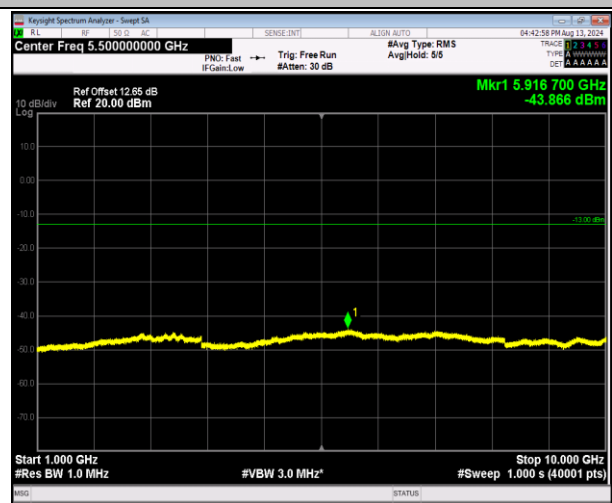
5-5-3MHz-5MHz-16QAM-16QAM-20416-20455-15RB#0-25RB#0-1000~10000MHz-PASS
