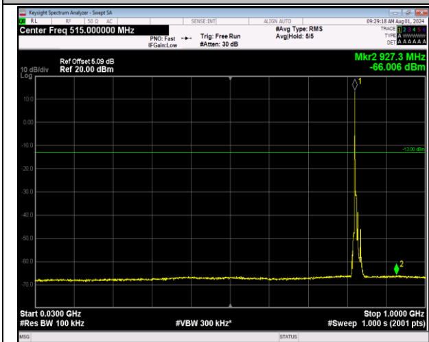
5-5-5MHz-3MHz-64QAM-64QAM-20425-20464-1RB#0-0RB#0-30~1000MHz-PASS
