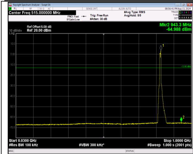
5-5-5MHz-3MHz-QPSK-QPSK-20425-20464-25RB#0-15 RB#0-30~1000MHz-PASS
