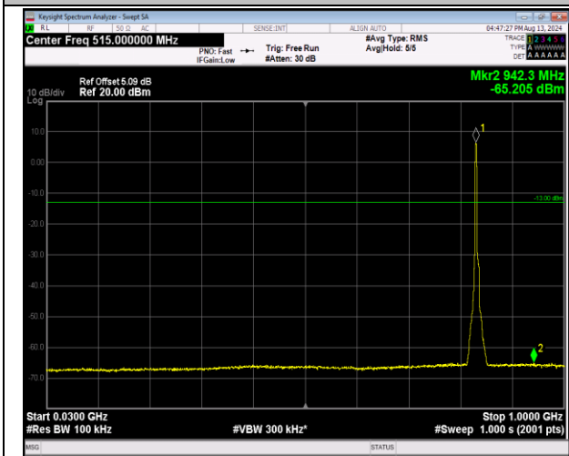
5-5-3MHz-5MHz-16QAM-16QAM-20501-20540-15RB#0-25RB#0-30~1000MHz-PASS
