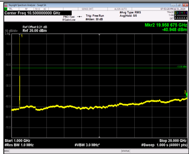
2-2-20MHz-20MHz-64QAM-64QAM-18902-19100-1RB#0-0 RB#0-1000~20000MHz-PASS
