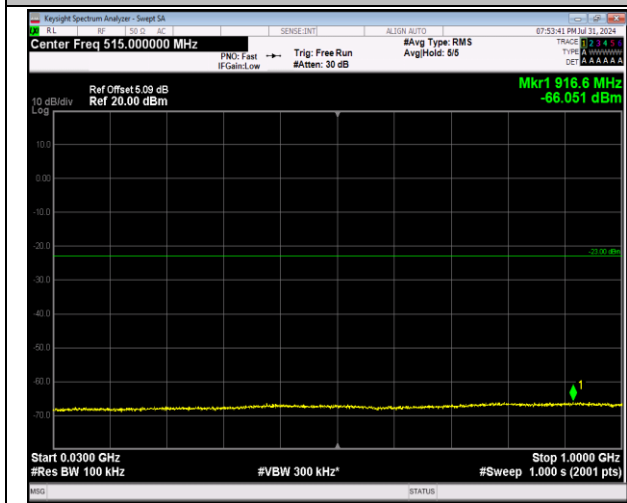
2-2-20MHz-20MHz-64QAM-64QAM-18902-19100-1RB#9 9-0RB#0-30~1000MHz-PASS
