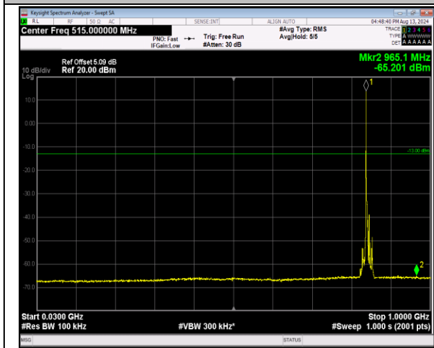
5-5-3MHz-5MHz-16QAM-16QAM-20586-20625-1RB#0-0 RB#0-30~1000MHz-PASS
