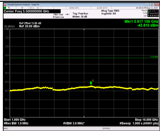
5-5-3MHz-5MHz-QPSK-QPSK-20416-20455-1RB#0-0RB#0 -1000~10000MHz-PASS
