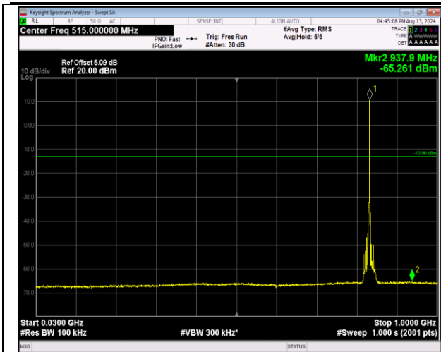
5-5-3MHz-5MHz-16QAM-16QAM-20501-20540-1RB#14-0RB#0-30~1000MHz-PASS
