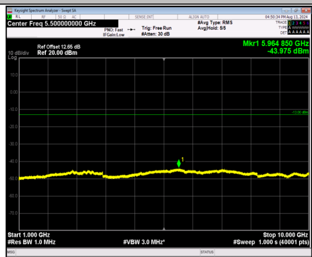
5-5-3MHz-5MHz-QPSK-QPSK-20586-20625-1RB#0-1RB#2 4-1000~10000MHz-PASS
