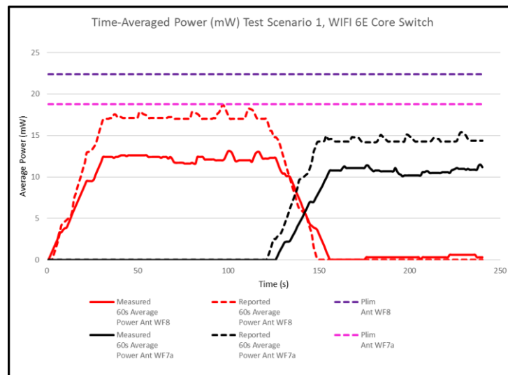
Figure I-6 60s Average Power vs. Time, 6 GHz
