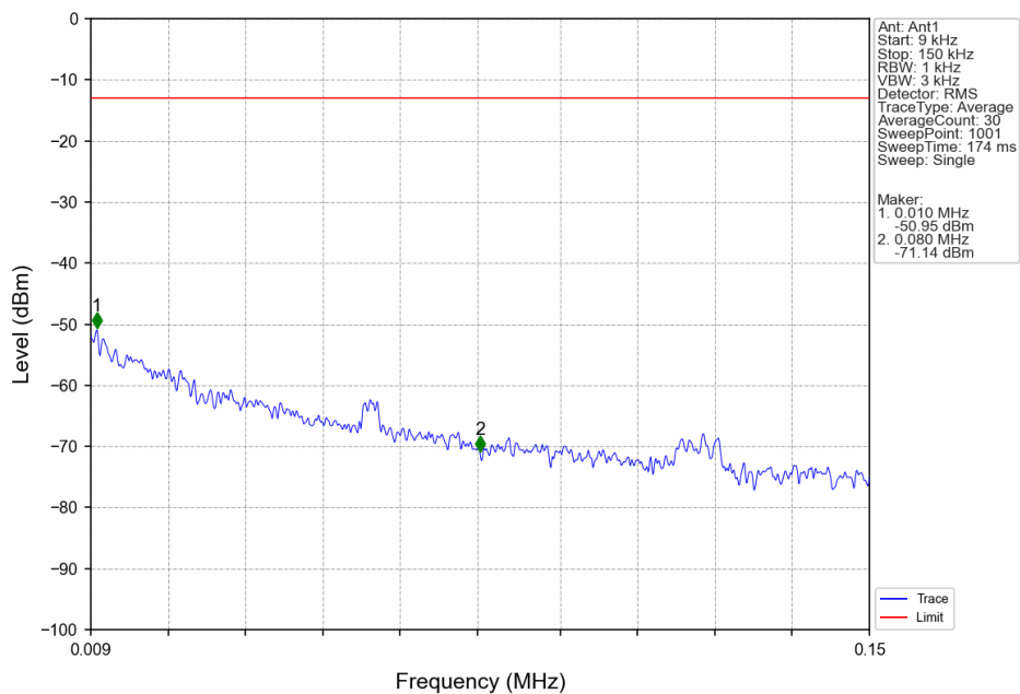
Band4 HSUPA HCH 1752.6MHz Subtest 1 NTN
