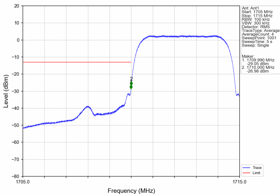
Band4_HSDPA_LCH_1712.4MHz_Subtest 1_NTN
