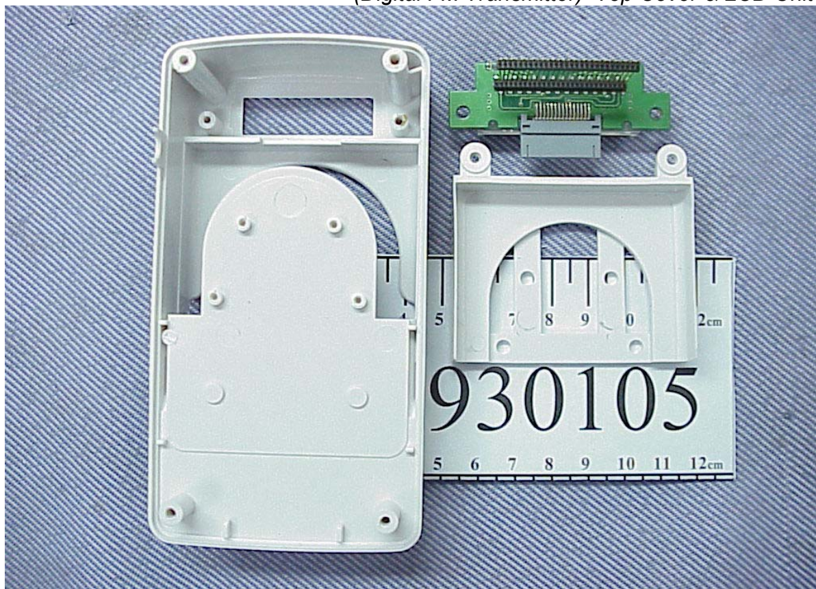
Photos 13 (Digital FM Transmitter) Top Cover & LCD Unit View
