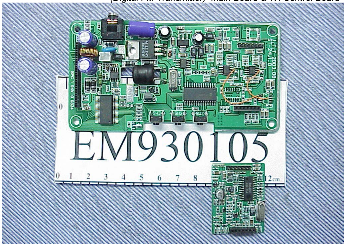
Photos 8 (Digital FM Transmitter) Main Board & TX Control Board View
