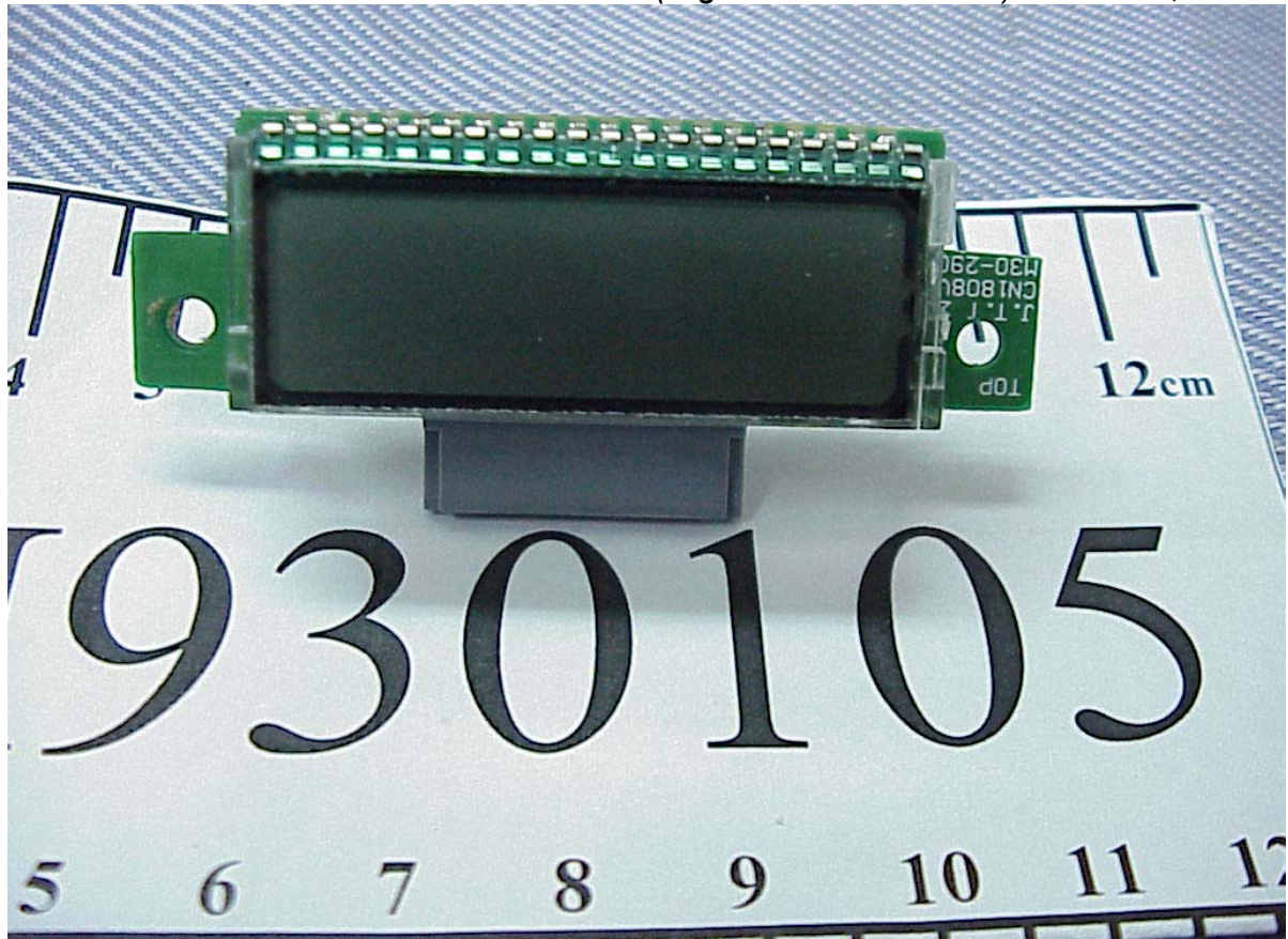
Photos 15 (Digital FM Transmitter) LCD Unit, Front View
