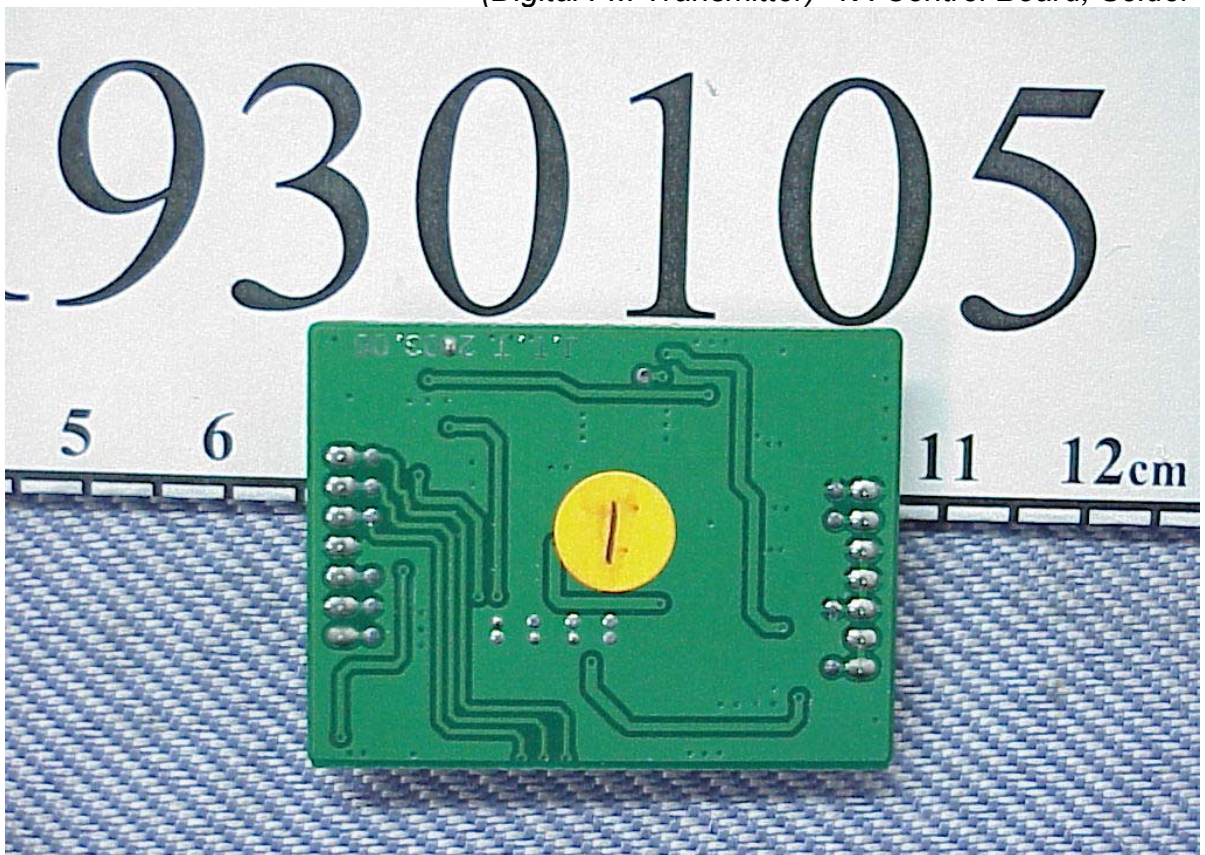
Photos 12 (Digital FM Transmitter) TX Control Board, Solder Side
