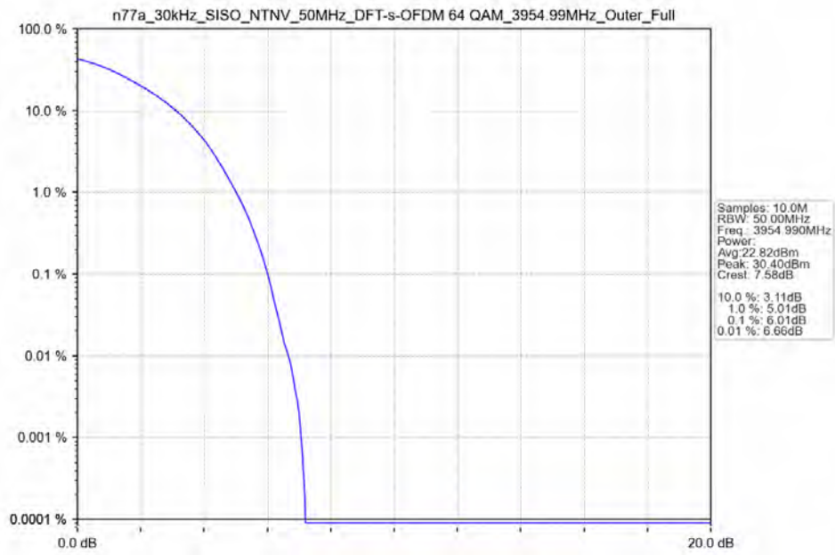
n77a_30kHz_SISO_NTNV_50MHz_DFT-s-OFDM_64_QAM_3954.99MHz_Outer_Full_Ant13
