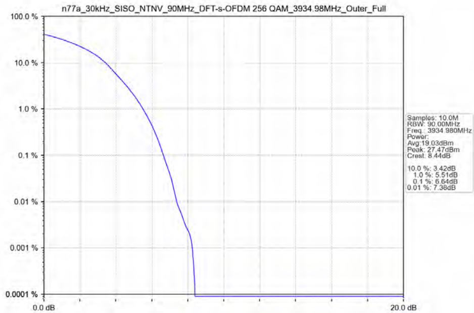
n77a_30kHz_SISO_NTNV_90MHz_DFT-s-OFDM_256_QAM_3934.98MHz_Outer_Full_Ant13
