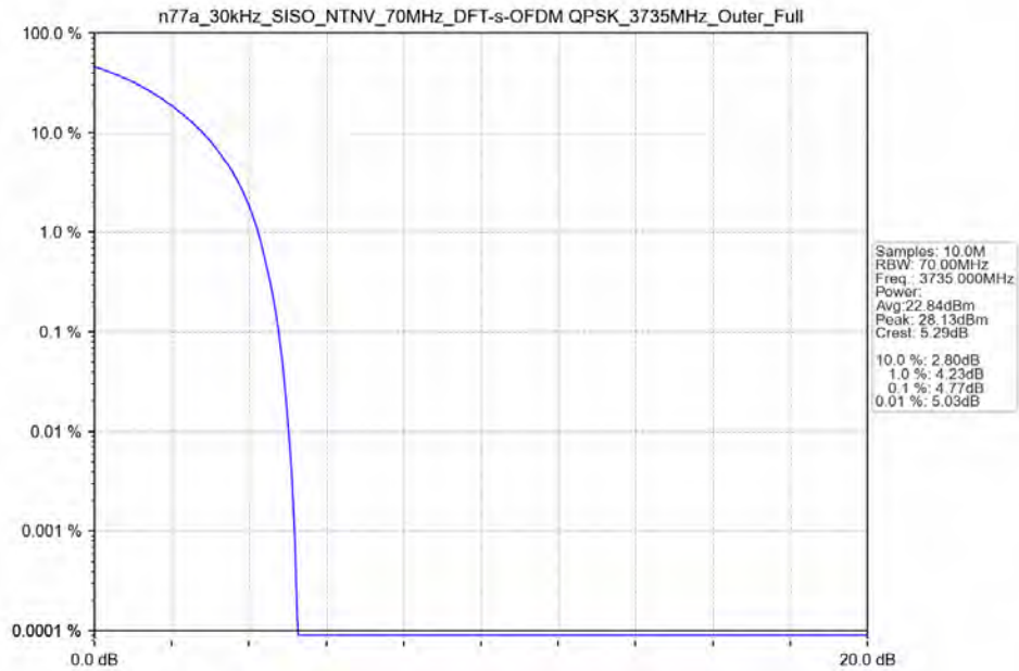
n77a_30kHz_SISO_NTNV_70MHz_DFT-s-OFDM QPSK_3735MHz_Outer_Full_Ant13
