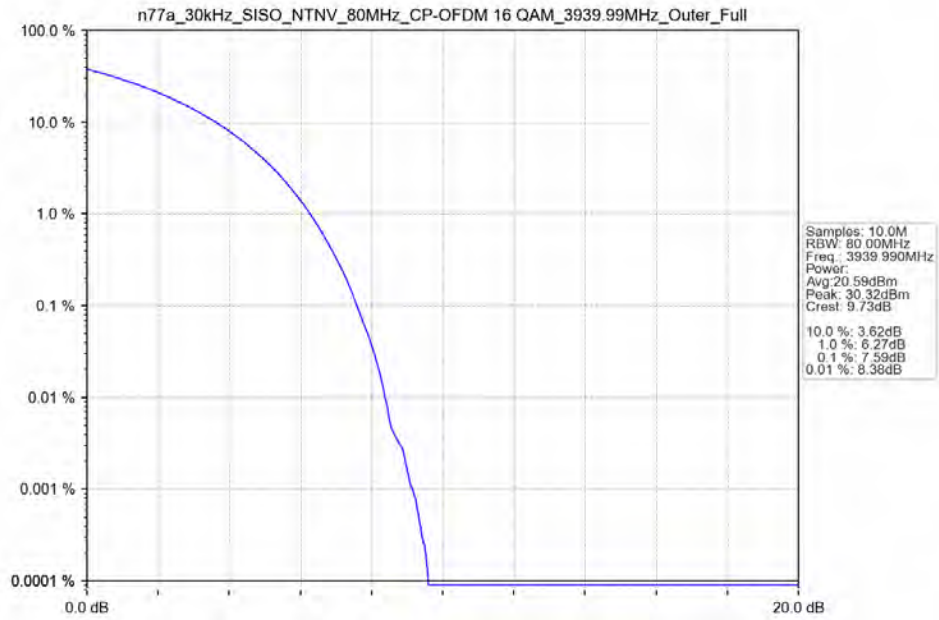
n77a_30kHz_SISO_NTNV_80MHz_CP-OFDM 16 QAM_3939.99MHz_Outer_Full_Ant13
