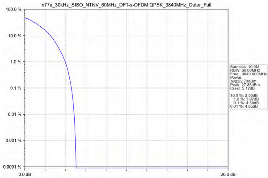
n77a_30kHz_SISO_NTNV_60MHz_DFT-s-OFDM_QPSK_3840MHz_Outer_Full_Ant13
