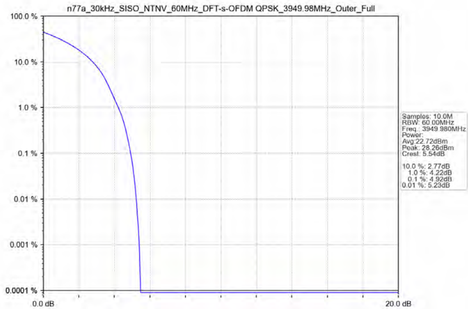
n77a_30kHz_SISO_NTNV_60MHz_DFT-s-OFDM_QPSK_3949.98MHz_Outer_Full_Ant13
