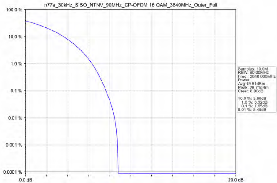
n77a_30kHz_SISO_NTNV_90MHz_CP-OFDM_16_QAM_3840MHz_Outer_Full_Ant13
