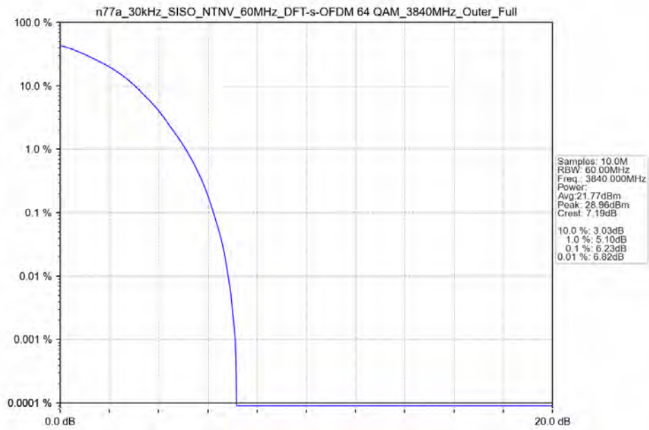
n77a_30kHz_SISO_NTNV_60MHz_DFT-s-OFDM_64_QAM_3840MHz_Outer_Full_Ant13
