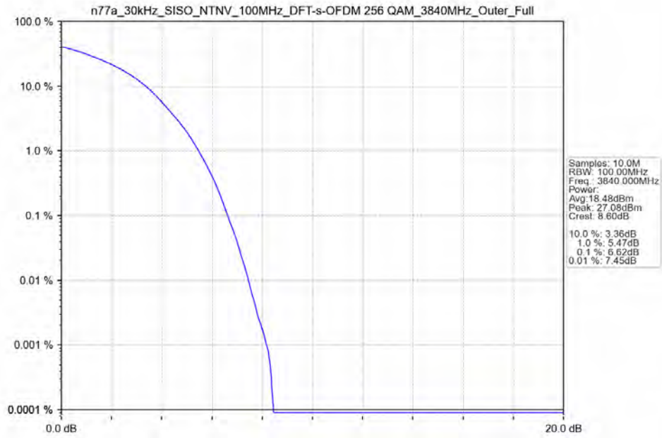
n77a_30kHz_SISO_NTNV_100MHz_DFT-s-OFDM_256_QAM_3840MHz_Outer_Full_Ant13
