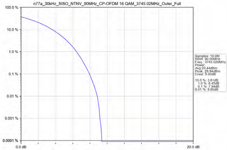
n77a_30kHz_SISO_NTNV_90MHz_CP-OFDM_16_QAM_3745.02MHz_Outer_Full_Ant13
