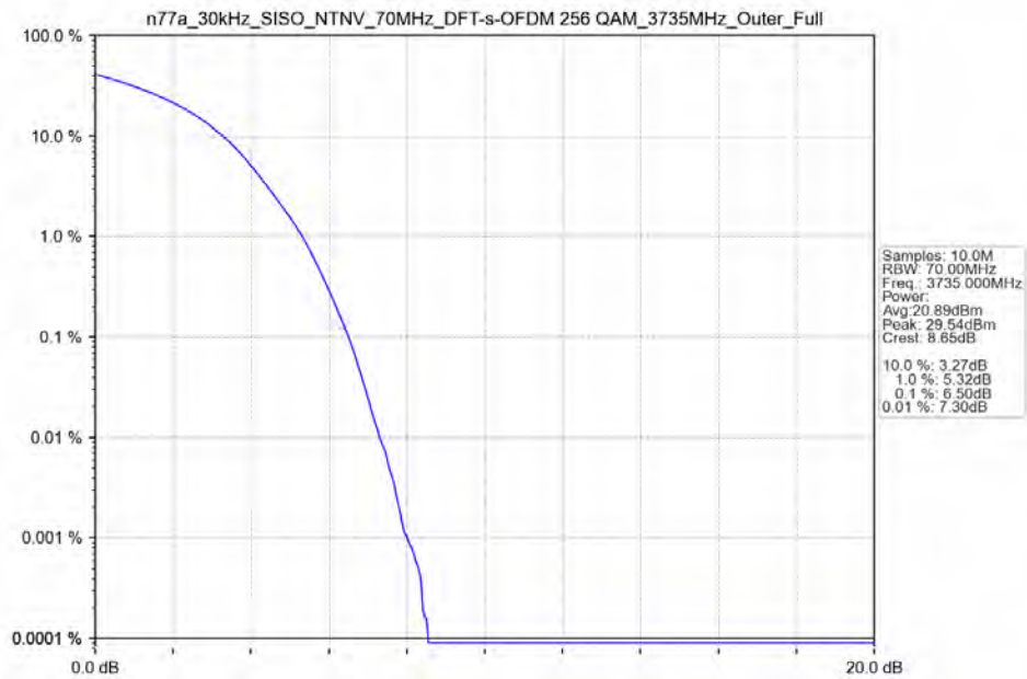
n77a_30kHz_SISO_NTNV_70MHz_DFT-s-OFDM_256_QAM_3735MHz_Outer_Full_Ant13
