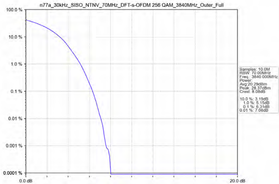
n77a_30kHz_SISO_NTNV_70MHz_DFT-s-OFDM_256_QAM_3840MHz_Outer_Full_Ant13
