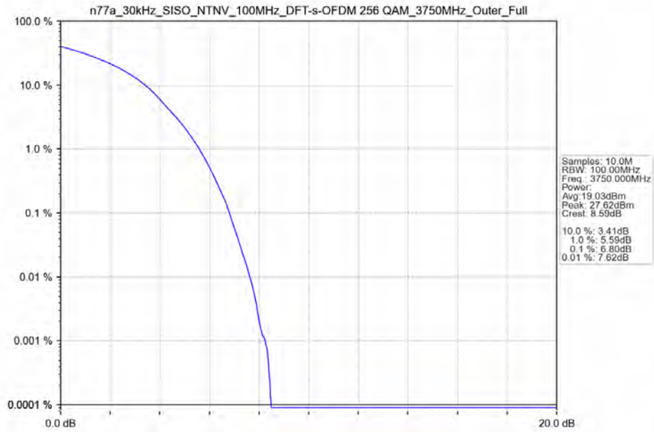
n77a_30kHz_SISO_NTNV_100MHz_DFT-s-OFDM_256_QAM_3750MHz_Outer_Full_Ant13
