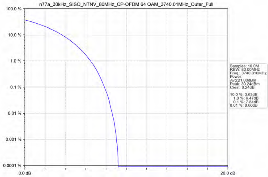
n77a_30kHz_SISO_NTNV_80MHz_CP-OFDM 64 QAM_3740.01MHz_Outer_Full_Ant13
