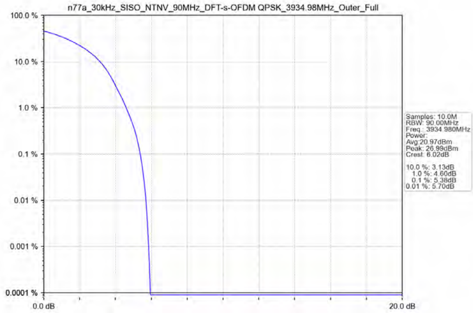
n77a_30kHz_SISO_NTNV_90MHz_DFT-s-OFDM_QPSK_3934.98MHz_Outer_Full_Ant13
