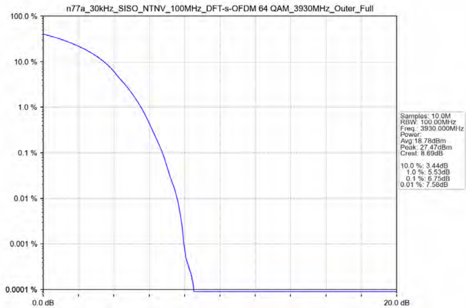
n77a_30kHz_SISO_NTNV_100MHz_DFT-s-OFDM_64_QAM_3930MHz_Outer_Full_Ant13
