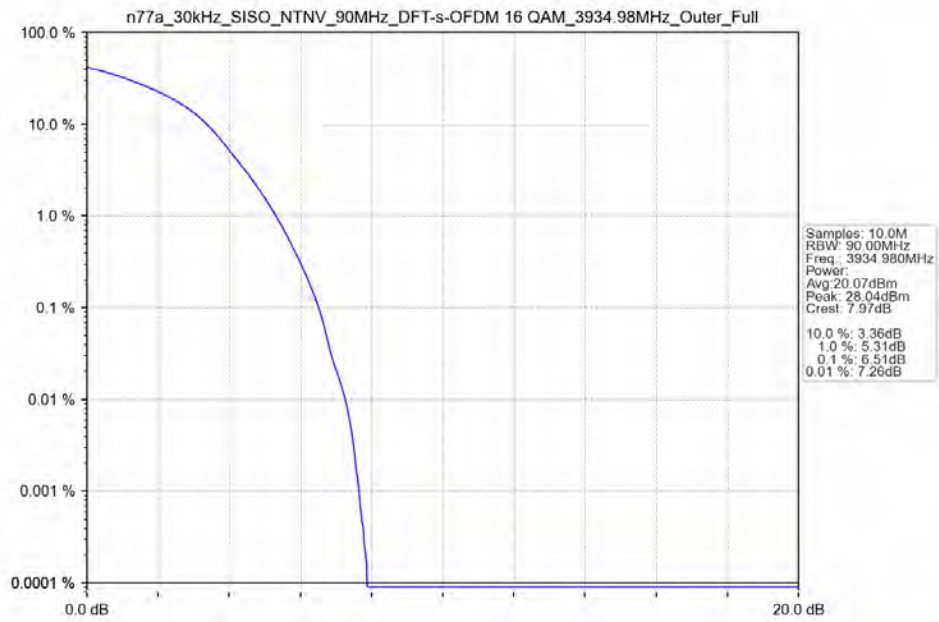
n77a_30kHz_SISO_NTNV_90MHz_DFT-s-OFDM_16_QAM_3934.98MHz_Outer_Full_Ant13
