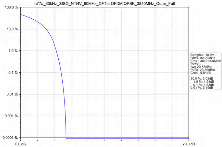
n77a_30kHz_SISO_NTNV_90MHz_DFT-s-OFDM_QPSK_3840MHz_Outer_Full_Ant13
