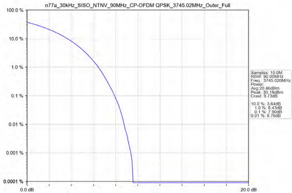
n77a_30kHz_SISO_NTNV_90MHz_CP-OFDM_QPSK_3745.02MHz_Outer_Full_Ant13
