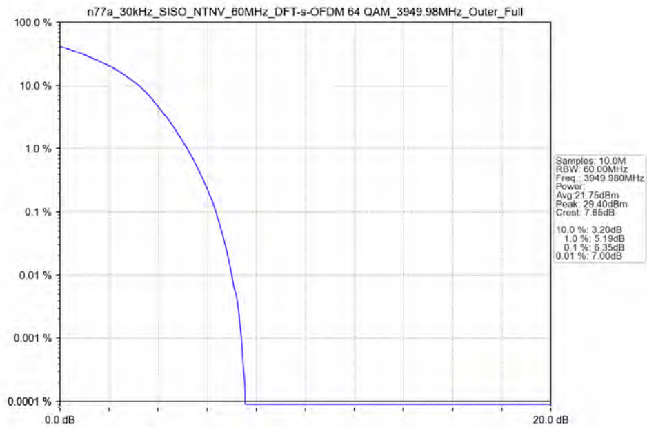
n77a_30kHz_SISO_NTNV_60MHz_DFT-s-OFDM_64_QAM_3949.98MHz_Outer_Full_Ant13
