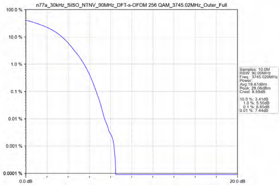
n77a_30kHz_SISO_NTNV_90MHz_DFT-s-OFDM_256_QAM_3745.02MHz_Outer_Full_Ant13
