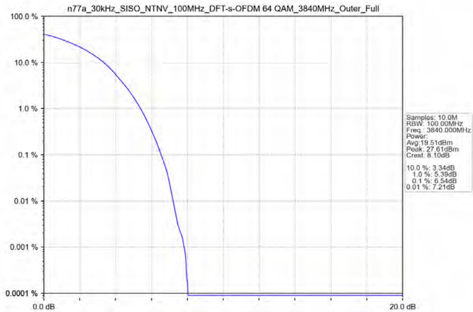
n77a_30kHz_SISO_NTNV_100MHz_DFT-s-OFDM_64_QAM_3840MHz_Outer_Full_Ant13
