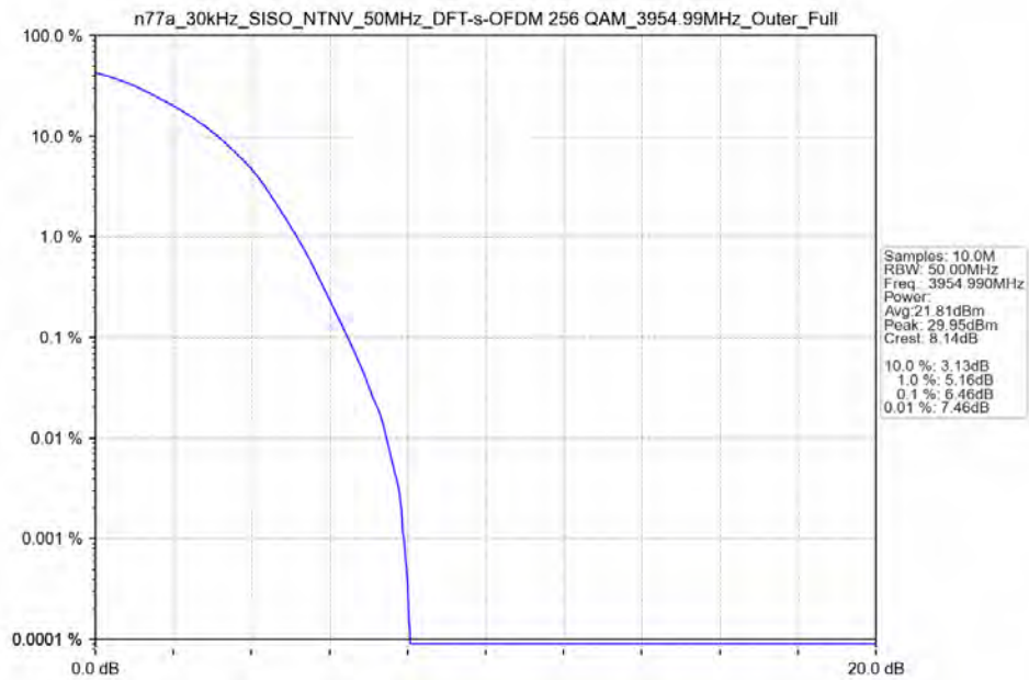
n77a_30kHz_SISO_NTNV_50MHz_DFT-s-OFDM_256_QAM_3954.99MHz_Outer_Full_Ant13
