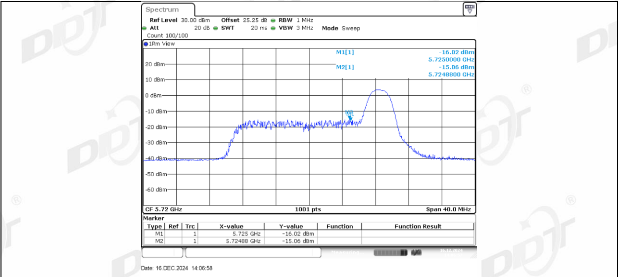
11AX20MIMO Ant2 5720 UNII-2C 52Tone RU37
