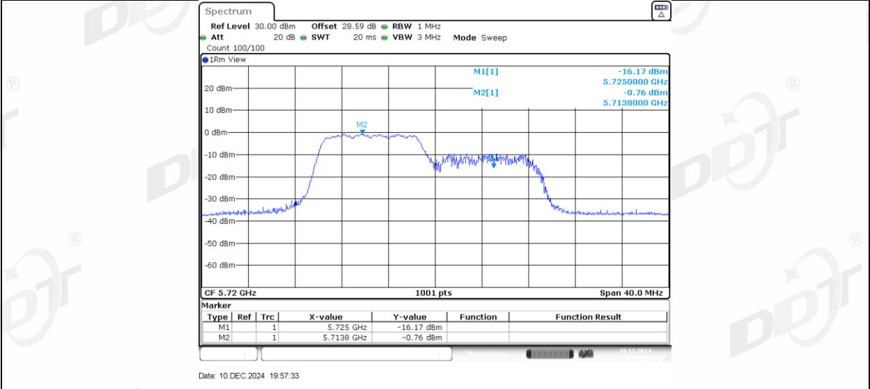
11AX20MIMO Ant1 5720 UNII-2C 106Tone_RU54
