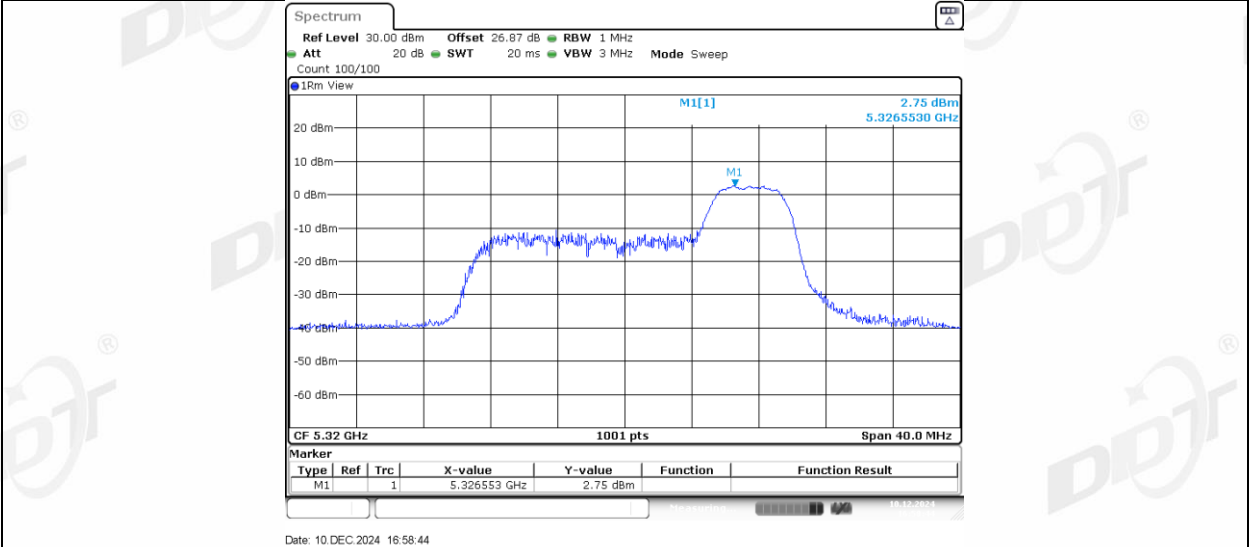
11AX20MIMO Ant2 5320_106Tone RU53
