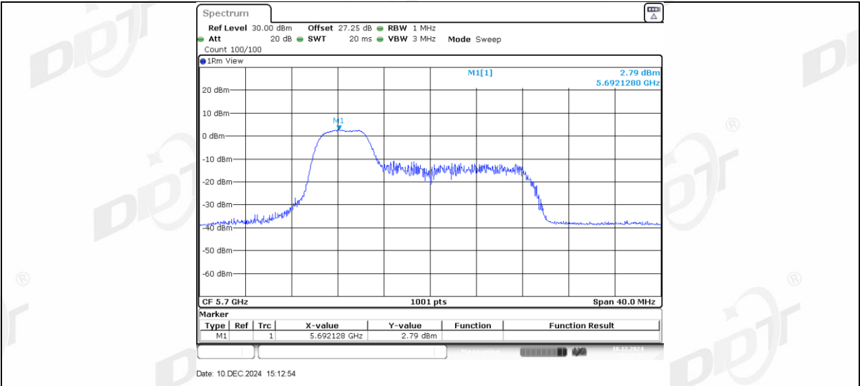
11AX20MIMO Ant2 5700_52Tone RU39
