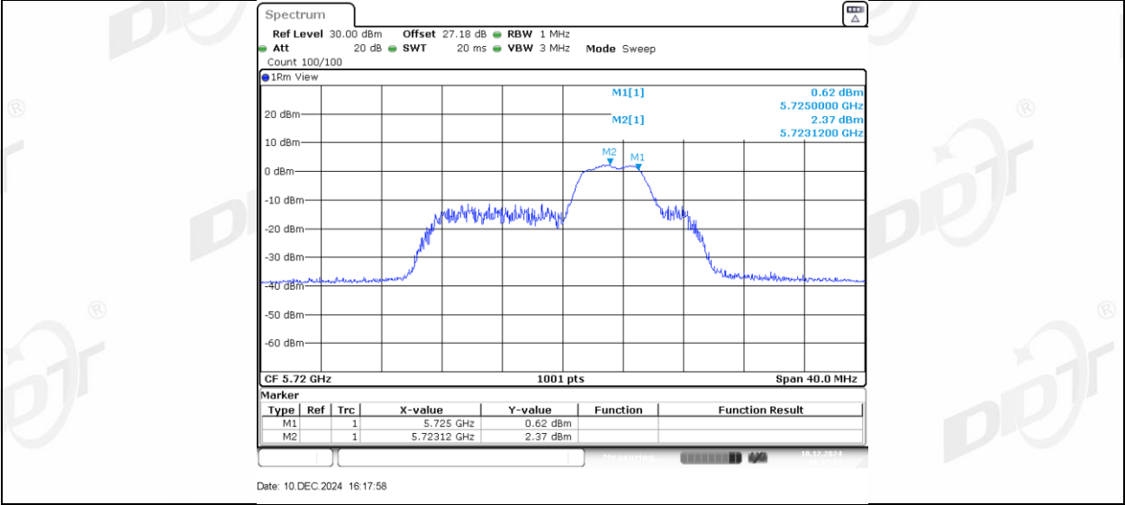
11AX20MIMO Ant2 5720 UNII-2C 52Tone RU40
