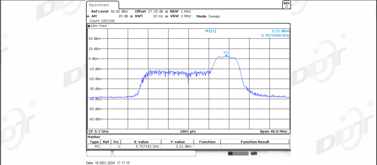
11AX20MIMO Ant2 5700_106Tone RU53
