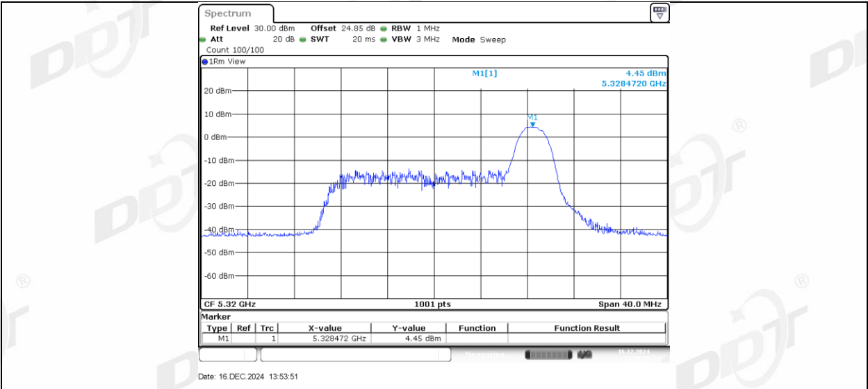
11AX20MIMO Ant1 5320_52Tone RU37
