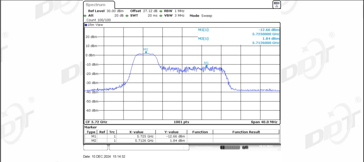
11AX20MIMO Ant1 5720 UNII-2C 52Tone RU39
