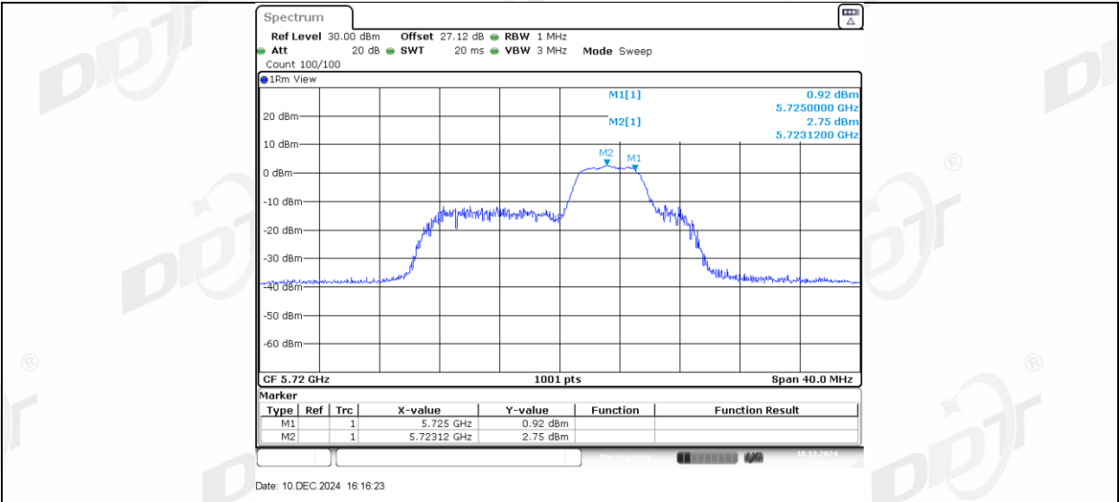
11AX20MIMO Ant1 5720 UNII-2C 52Tone_RU40
