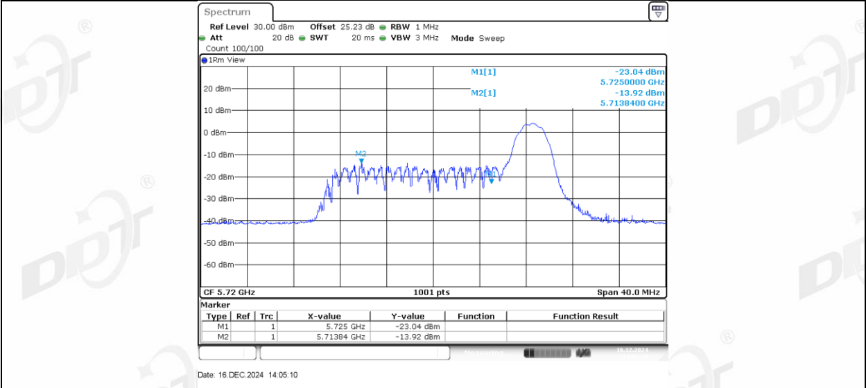
11AX20MIMO Ant1 5720 UNII-2C 52Tone RU37
