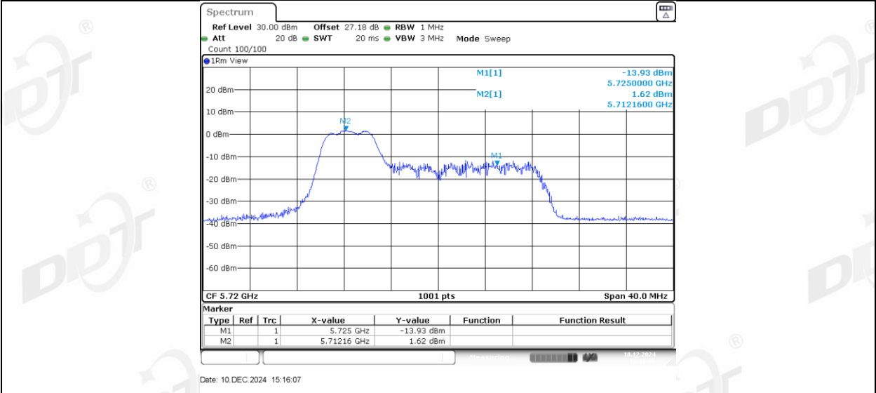
11AX20MIMO Ant2 5720 UNII-2C 52Tone RU39
