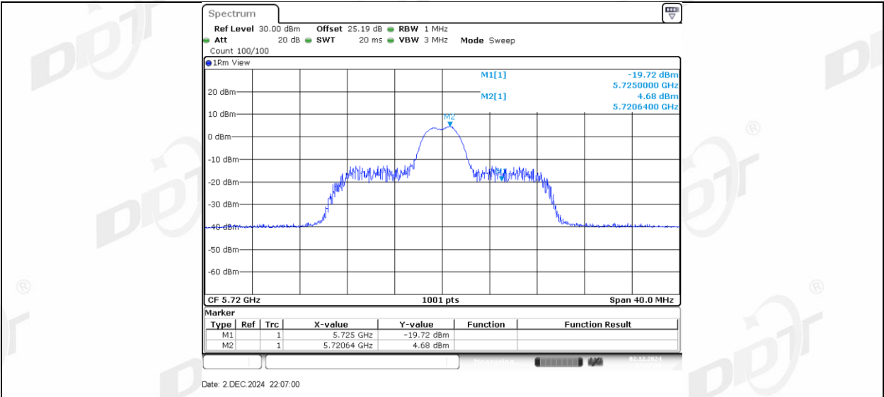
11AX20MIMO Ant1 5720 UNII-2C 26Tone RU8
