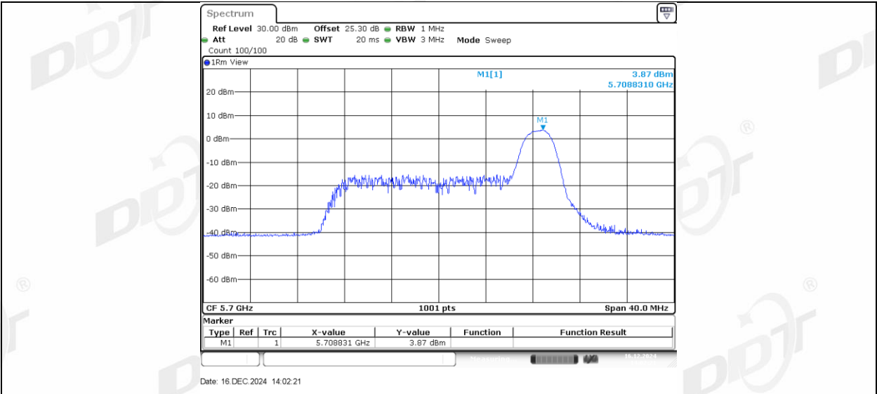
11AX20MIMO Ant1 5700_52Tone RU37
