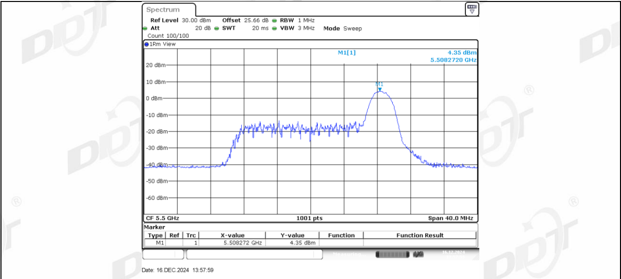
11AX20MIMO Ant2 5500_52Tone RU37
