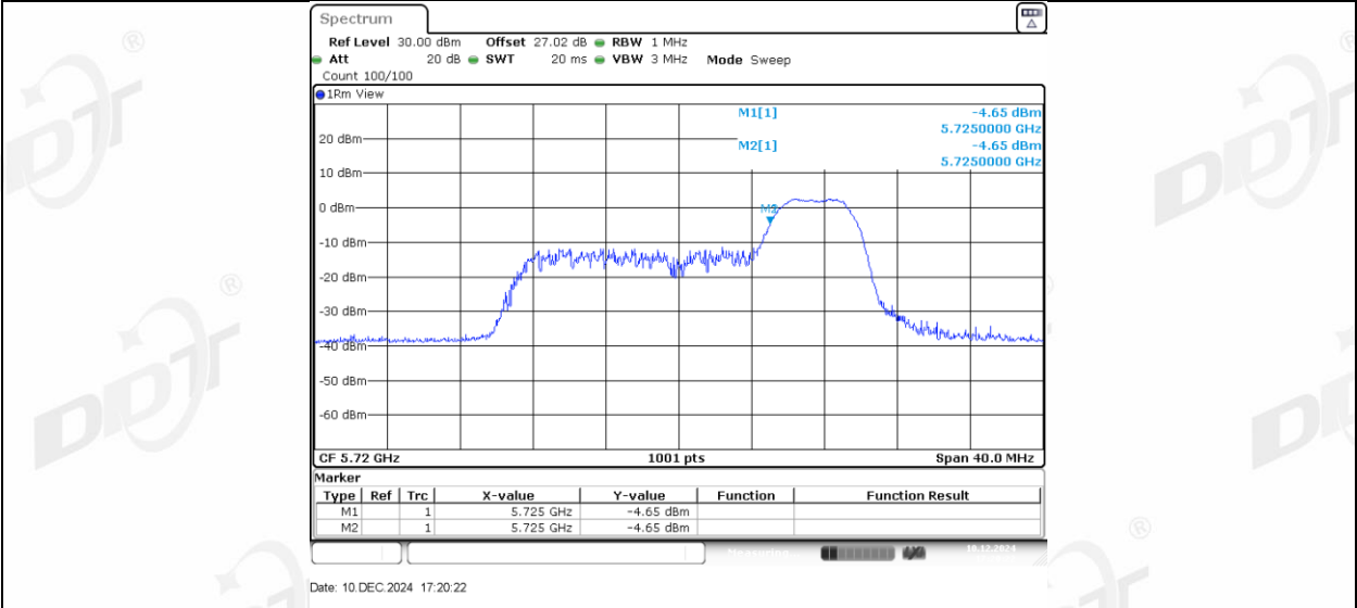
11AX20MIMO Ant1 5720 UNII-2C 106Tone_RU53
